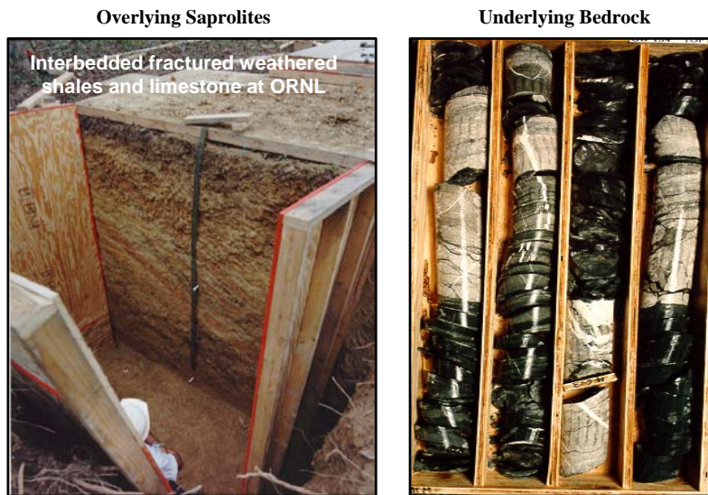
Figure 2: Typical subsurface media on the Oak Ridge Reservation consisting of interbedded shale – limestone sequences with characteristic dipping bedding planes.
