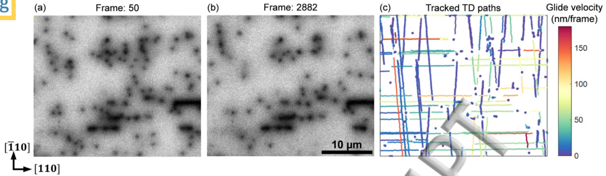
Fig. 2. Panchromatic cathodoluminescence emission from the AlGaAs ( x=0 ) heterostructure showing dark spots due to non-radiative recombination at threading dislocations. The images are taken with a 3 nA absorbed current and show the position of threading dislocations after (a) 50 frames and (b) 2882 frames (also in supplementary videos). A number of dislocations have exited the imaging area by REDG. (c) Tracks of the gliding TDs from the same area, colored by the glide velocity. Four types of dislocation behavior are seen: slow and fast motion along [\bar{1}10] , fast motion along [110] , and stationary dislocations. The inclined lines are due to the substrate offset.
