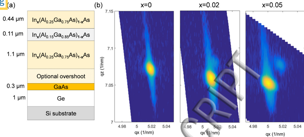
Fig. 1 (a) Layer structure of the arsenide heterostructures on silicon. The indium-free x=0 sample is used for the detailed characterization of REDG in III.A and filtering in III.C. The indium containing x=0.02 and x=0.05 form the basis of III.B where REDG is seen to be arrested. An overshoot layer is used for a second x=0.05 sample to modify the residual strain. (b) A portion of the \bar{2}24 x-ray reciprocal space maps of the films for the compositions indicated. The weaker peak seen in x=0.02 and 0.05 correspond to GaAs/Ge. We used larger scans that included the Si substrate peak to calculate the residual strain at room temperature. The sample with overshoot is not shown here.
