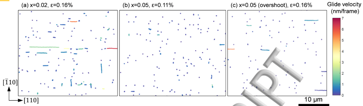
Fig. 4 Tracks of threading dislocations undergoing recombination-enhanced glide colored by their velocity (also in supplementary videos). The samples (and number of frames) are x \approx 0.02 (2100), x=0.05 (1600), and x=0.05 (2100) with the overshoot layer. The residual strain is also listed. A sample absorbed current of \approx 3 nA is used. The dislocation glide velocity clearly reduces upon the addition of indium and a majority of dislocations are stationary.
