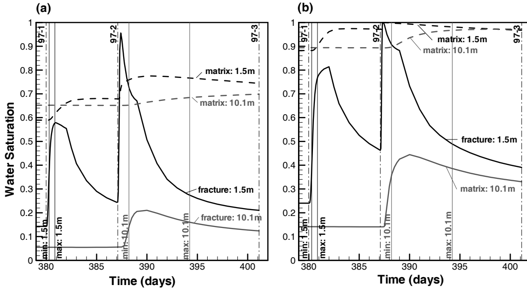
Figure 5: Simulated infiltration front arrival times at sampling points in borehole I-1 given by water saturation in the fracture and matrix continua using (a) Corey and (b) van Genuchten relative permeability functions.
