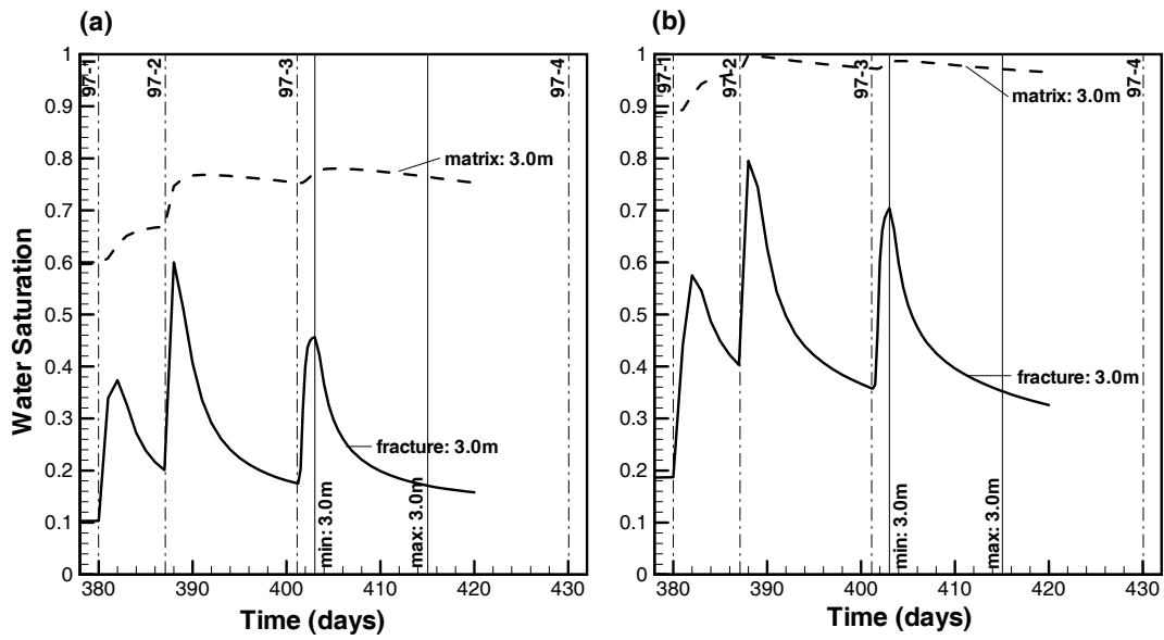
Figure 7: Simulated infiltration front arrival time in borehole T-5 given by water saturation in the fracture and matrix continua using (a) Corey and (b) van Genuchten relative permeability functions.
