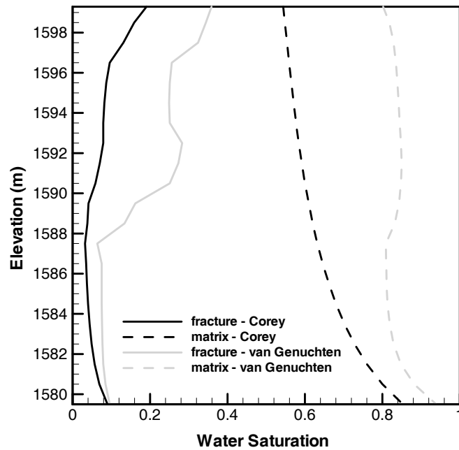
Figure 4: Water saturation profile in borehole I-1 for the fracture and matrix continua immediately prior to the 97-1 infiltration test.
