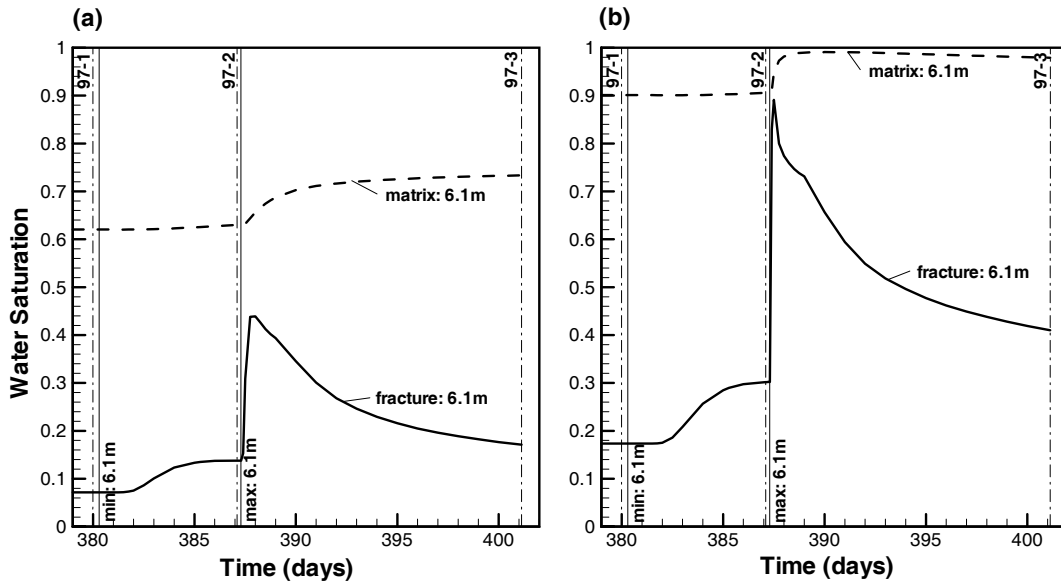
Figure 6: Simulated infiltration front arrival time in borehole I-2 given by water saturation in the fracture and matrix continua using (a) Corey and (b) van Genuchten relative permeability functions.
