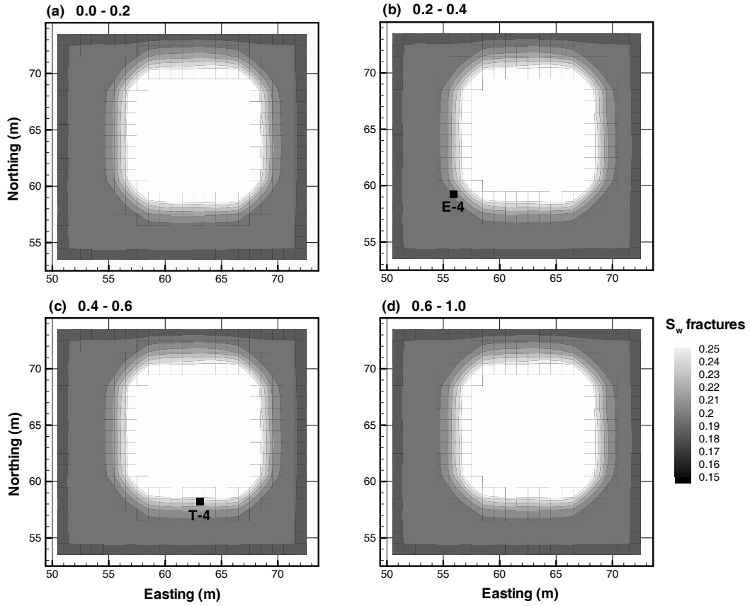
Figure 9: Water saturation distribution in the fracture continuum 2.9 days into the 97-2 infiltration test—390 days since the start of 96-1.
