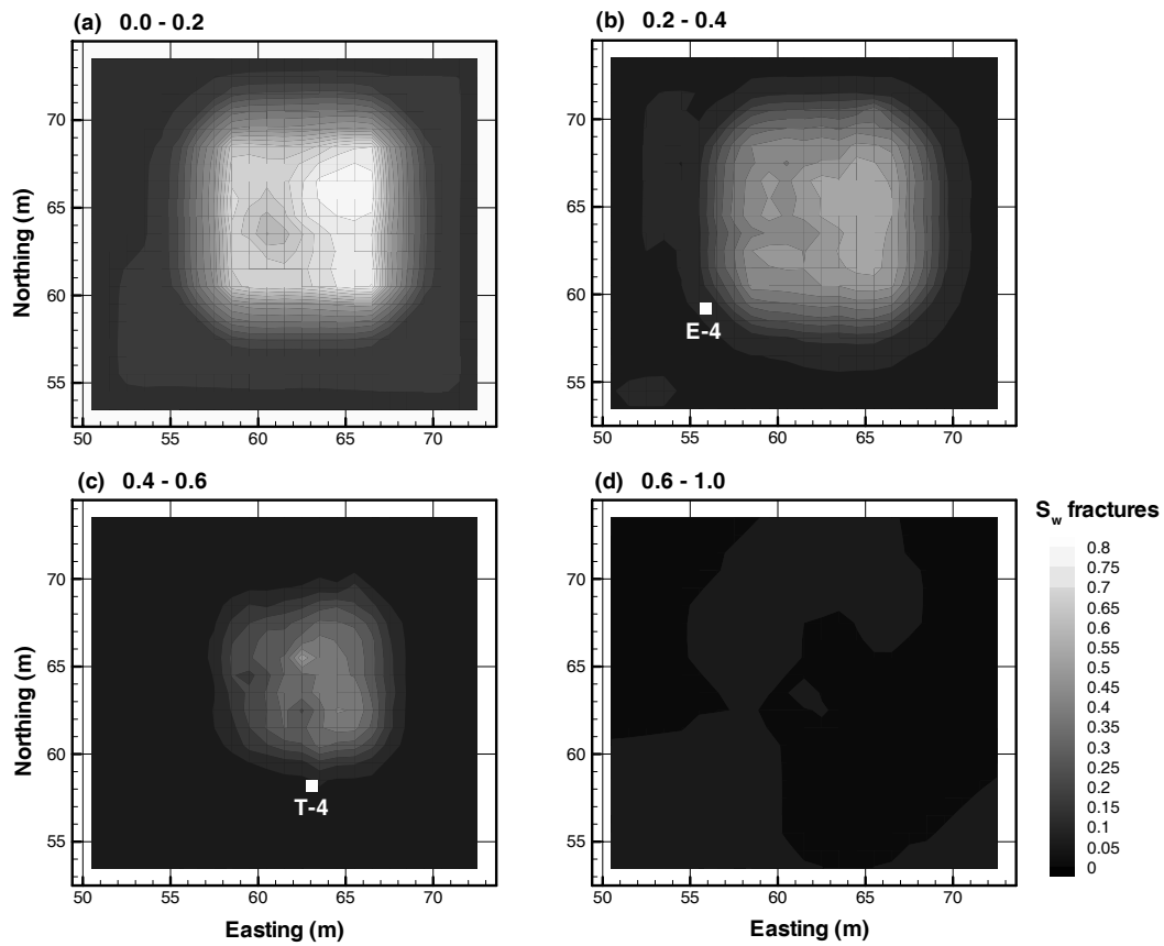
Figure 8: Water saturation distribution in the fracture continuum 0.9 days into the 97-2 infiltration test—388 days since the start of 96-1.
