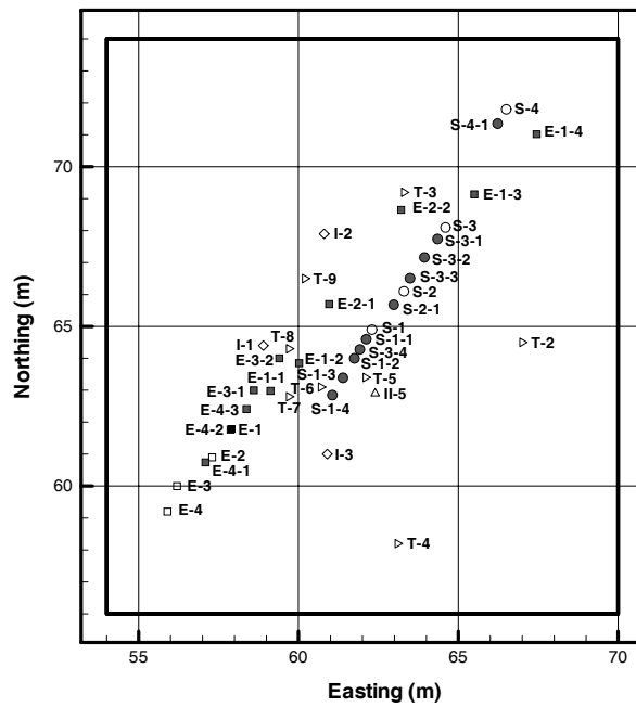
Figure 3: Plan view of the location of borehole intersections with active water conducting fractures. Open symbols indicate the surface location of a borehole while shaded symbols indicate the intersection with active water conducting fractures.
