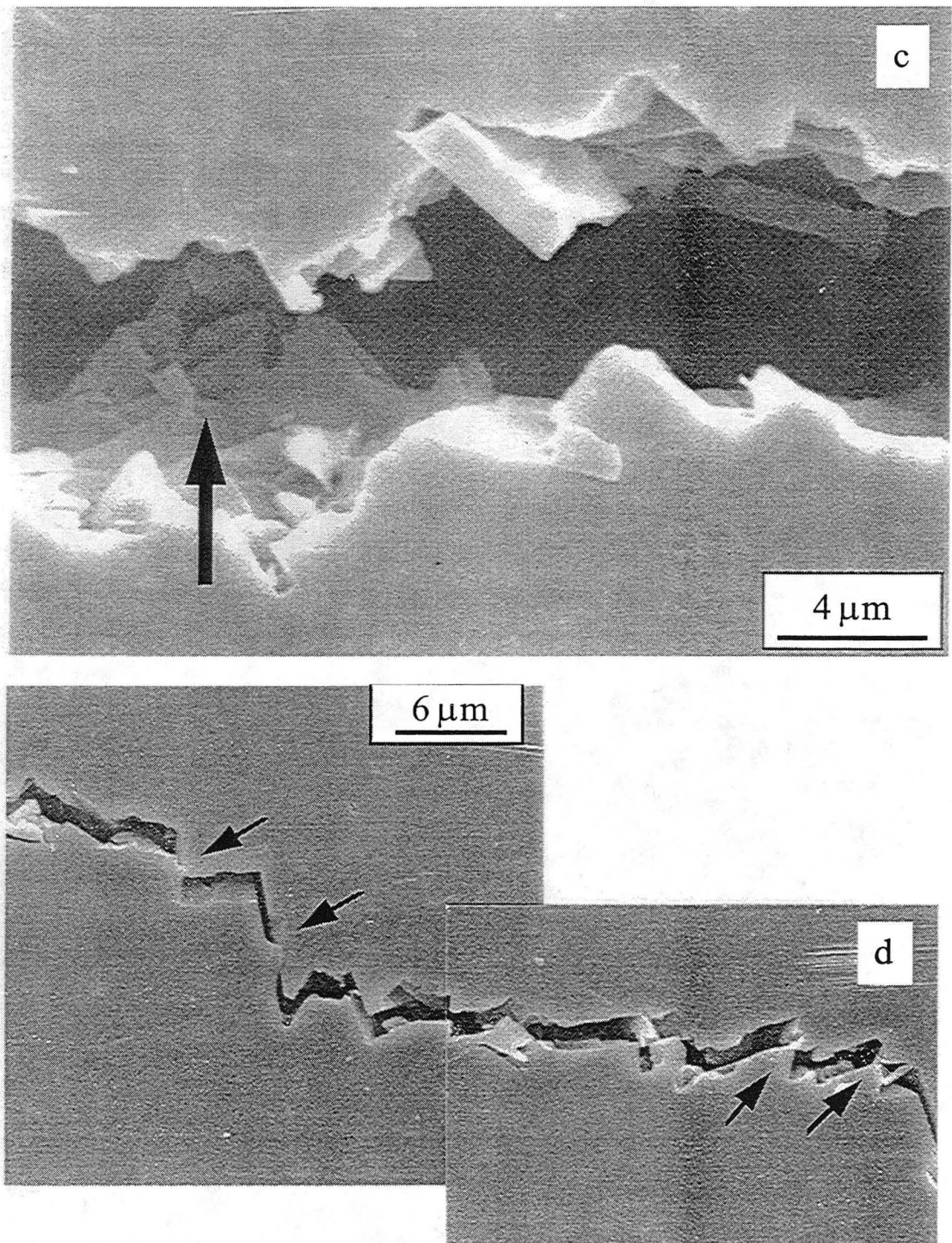
Fig. 3-14 SEM micrographs showing that grains were pulled out (a), a grain fractured after some sliding (b), a group of grains were pulled out (c), and that contacting facets provided additional sliding friction (d).
