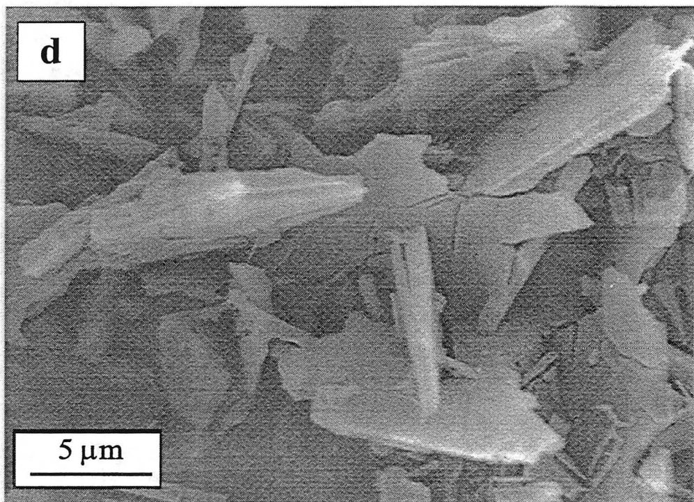
Fig. 2-6 SEM micrographs of (a) a green compact and of the ABC-SiC hot pressed at various conditions: (b) 1700°C/1h, (c) 1780°C/1h, and (d) 1900°C/4h (etched in a molten salt mixture at 500°C for 8 hours).
