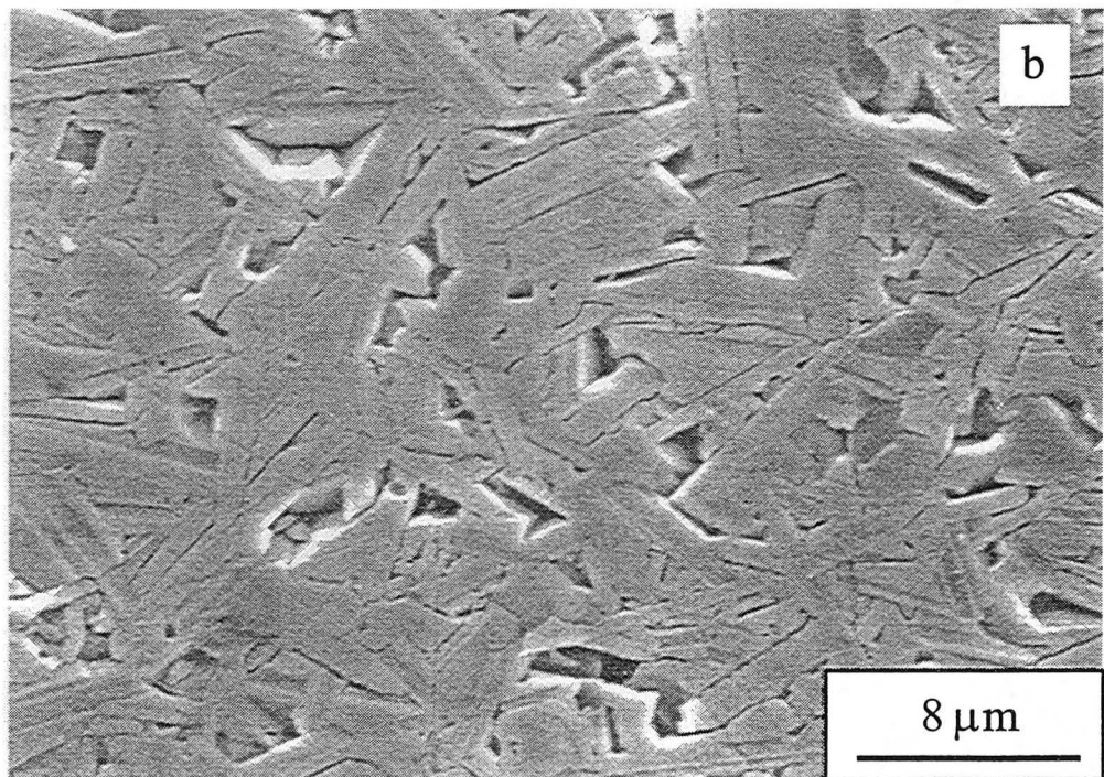
Fig. 2-9 (a) Optical and (b) SEM micrographs of an etched surface of the ABC-SiC hot pressed at 1900°C for 1 h.
