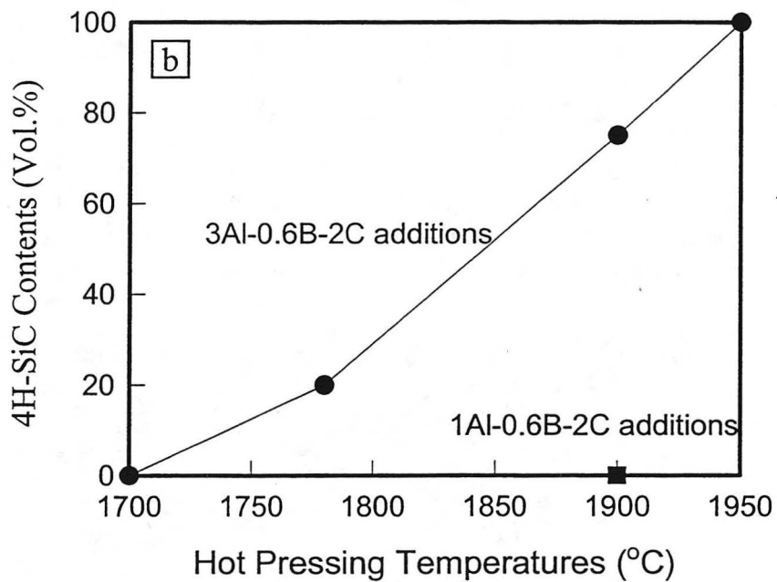
Fig. 2-3 X-ray diffraction spectra of the starting \beta -SiC powder and of the ABC-SiC materials hot pressed for 1 hour at 1700°C, 1780°C, 1900°C, and 1950°C, respectively (a). Fig. 2-3b plots the volume fraction of the 4H phase in ABC-SiC processed for 1 hour with 3 wt% Al-0.6 wt% B-2 wt% C as a function of temperature. The material with 1 wt% Al contains negligible \alpha phase after hot pressing at 1900°C for 1 hour.
