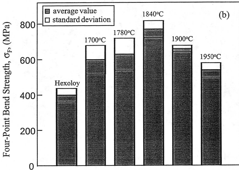
Fig. 3-2 Fracture toughness (a) and four-point bend strength (b) of the ABC-SiC materials hot pressed between 1700°C and 1950°C. Data for Hexoloy SiC, measured under identical conditions, are included for comparison.
