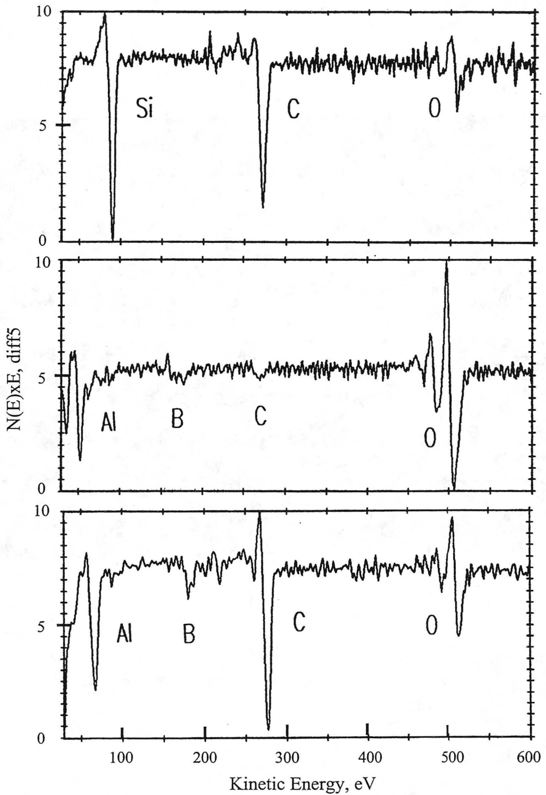
Fig. 2-16 AES spectra acquired of a SiC grain (a) and of secondary phases (b and c). (Courtesy of W. J. MoberlyChan)
