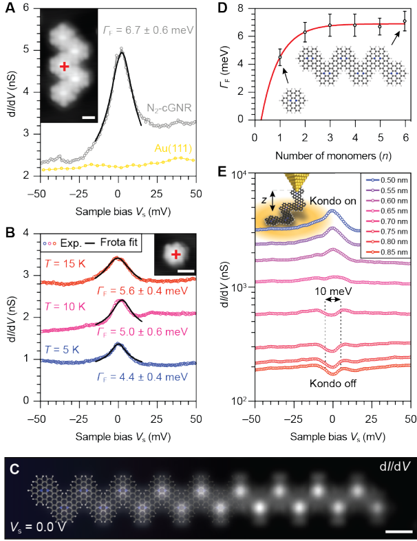
Figure 4. Kondo resonance in N_2^+ -cGNRs. (A) dI/dV spectrum recorded on a N_2^+ -cGNR at the position marked in the inset. I_F is the Fröta parameter (spectroscopy: V_{ac} = 1 mV, f = 533 Hz; imaging: V_s = 0.1 V, I_t = 200 pA). (B) Variable temperature dI/dV spectra recorded on a diazhexabenzocoronene monomer at the position marked in the inset (spectra are vertically offset by 1 nS for clarity). (C) Constant height dI/dV map of an octadecamer N_2^+ -cGNRs recorded with an unfunctionalized STM tip at V_s = 0.0 V showing the spatial density variations of the ZBR associated with the 1D Kondo chain. A structural model of N_2^+ -cGNR is overlaid on the left side of the ribbon. (D) Evolution of I_F as a function of the N_2^+ -cGNR length. (E) STS lift-off experiment performed on a heptamer N_2^+ -cGNR. Color gradient indicates the apparent z -height of the STM tip above the surface. Scale bars: 1 nm.
