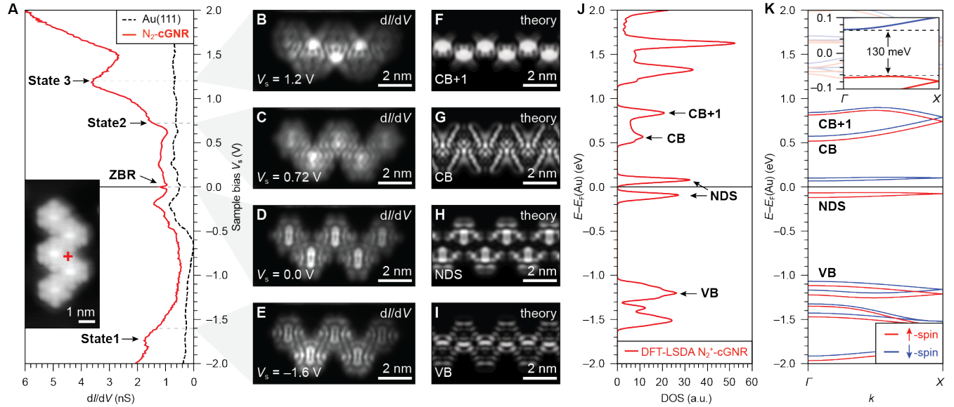
Figure 3. Electronic structure of \text{N}_2^+ -cGNRs. (A) STS dI/dV spectrum recorded on a \text{N}_2^+ -cGNR at the position marked by a red cross in the inset STM topographic image (spectroscopy: V_{ac} = 4\text{ mV} , f = 533\text{ Hz} ; imaging: V_s = 0.1\text{ V} , I = 200\text{ pA} , CO-functionalized tip). (B–E) Constant height dI/dV maps recorded at the indicated biases ( V_{ac} = 30\text{ mV} , f = 533\text{ Hz} , CO-functionalized tip). (F–I) DFT simulated LDOS maps of the CB+1, CB, NDS, and the VB of \text{N}_2^+ -cGNR. The maps are calculated at the band edge energies. (J) DFT-LSDA calculated DOS of \text{N}_2^+ -cGNR. The \text{N}_2^+ -cGNR is doped with two holes per unit cell (spectrum broadened by 30 meV Gaussian). Features associated with the CB+1, CB, NDS, and VB are indicated by arrows. (K) DFT-LSDA calculated band structure of \text{N}_2^+ -cGNR. Inset shows the opening of an indirect band gap attributed to the Stoner magnetic instability.
