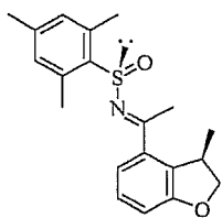
FIGURE 1. Absolute configuration determined by X-ray structure obtained for sulfanyl imine ( S 8 , R )-33.
