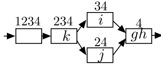
Figure 2.13: Queueing Network of Virtual Queues for the DAG in Figure 2.2
