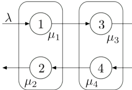
Figure 3.1: Lu-Kumar network
