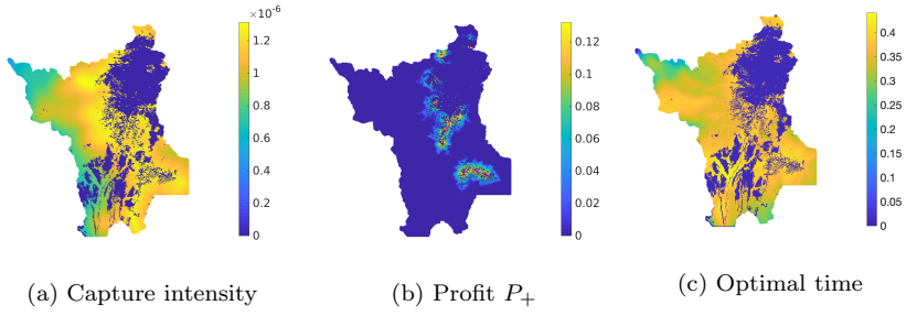
Fig. 15: (a) Capture intensity is based on benefit and distance, with w = 0.2, r = 5 in equation (18). (b) Expected non-negative profit P_+ over the entire region. (c) Optimal logging time plotted on regions with positive benefit.
