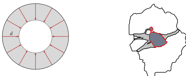
(a) Model of Albers' [1] applies only to symmetric areas (b) Model of Arnold et al. [2] applied to Yosemite National Park
