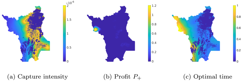
Fig. 16: (a) Capture intensity is based on benefit and distance, with w = 0.2, r = 15 in equation (18). (b) Expected non-negative profit P_+ over the entire region. (c) Optimal logging time plotted on regions with positive benefit.
