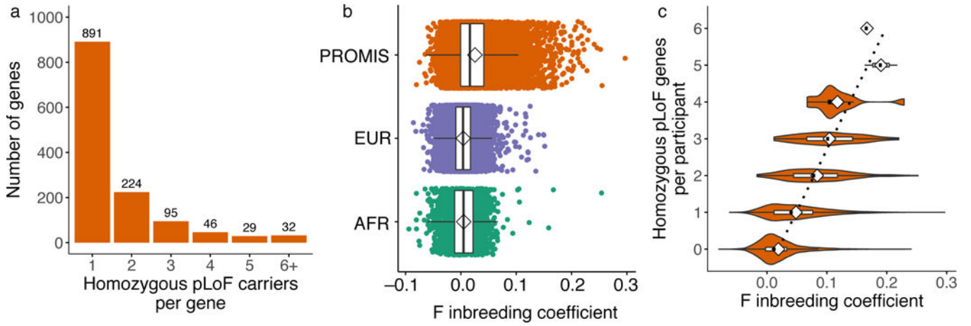
Fig 1. Homozygous pLoF burden in PROMIS is driven by excess autozygosity
