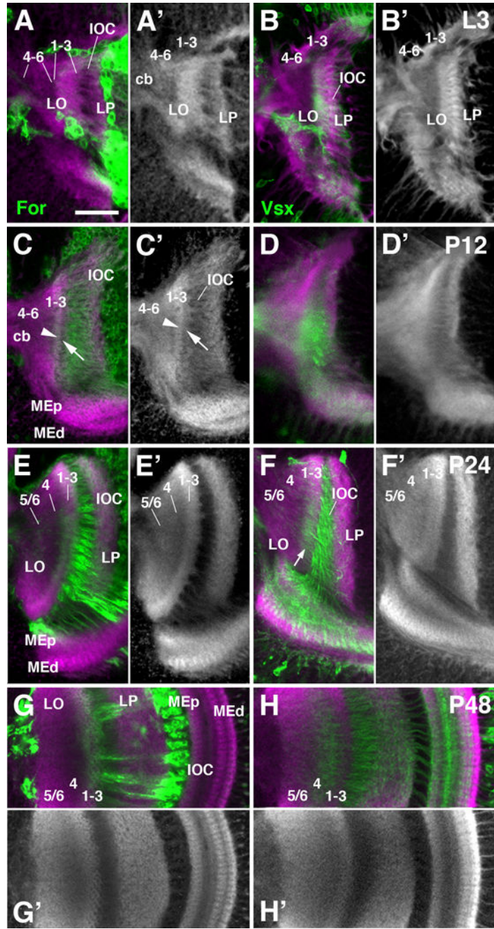
Figure 12. Layering of the lobula neuropil during metamorphosis. Frontal sections of the optic lobe labeled by for-Gal4 lineage tracing (green; A-A', C-C', E-E', G-G') and Vsx1-Gal4 (green; B-B', D-D', F-F', H-H') and counterstained with anti-DNcadherin (magenta in A-H; gray in A'-H') at late larval stage (L3; first row; A-B'), 12h pupa (P12; second row; C-D'), 24h pupa (P24; third row; E-F'), and 48h pupa (P48; fourth and fifth row; G-H'). The tripartite subdivision of the lobula neuropil is visible from P24 onward (E, E'). Prior to this stage, a thin, DNcadherin rich band demarcates a protolayer for 1-3, in which for-Gal4 -positive axon
