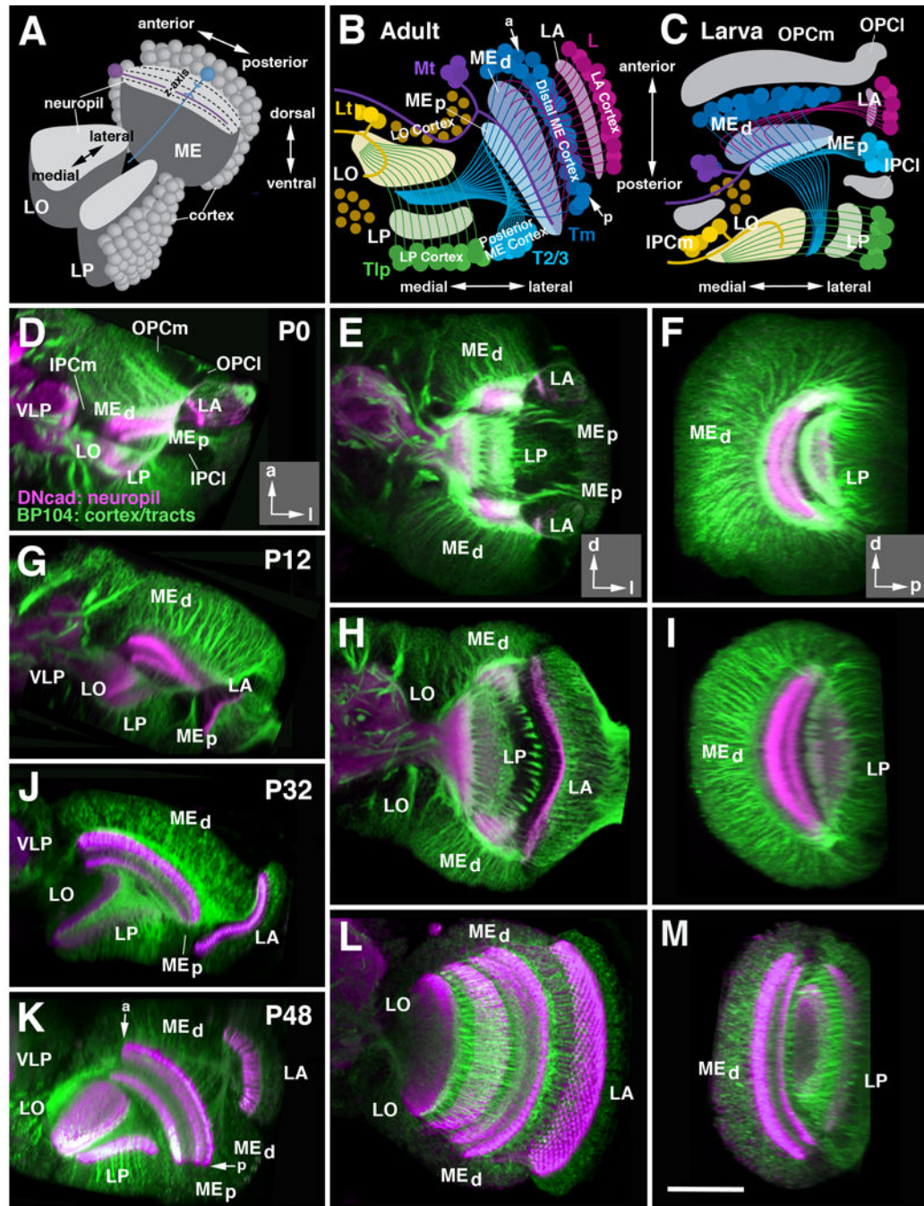
Figure 4. Morphogenesis of the optic lobe during metamorphosis. (A) Schematic cutaway model of the adult optic lobe, delineating orientation of medulla (ME), lobula (LO) and lobula plate (LP) relative to the body axis. For each of the optic ganglia, the cellular cortex and underlying neuropil is shown. Neuropils are subdivided into layers along the z-axis, as shown for the medulla (hatched lines). The large majority of neurons in all optic ganglia are columnar neurons (represented by the medulla neuron shown in blue) whose main fiber penetrates the neuropil along the z axis. Tangential neurons (purple) project parallel to
