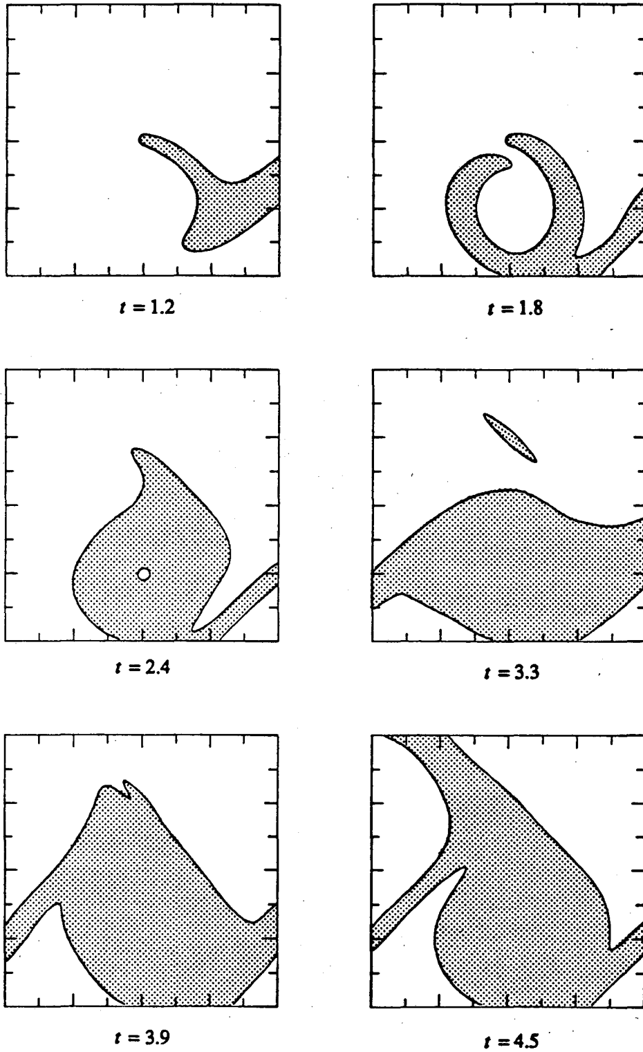
FIG. 6 Constant ignition at the center: F(\kappa) = 0.2
