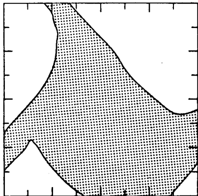
FIG. 8 Constant ignition at the center: F(\kappa) = 0.2
