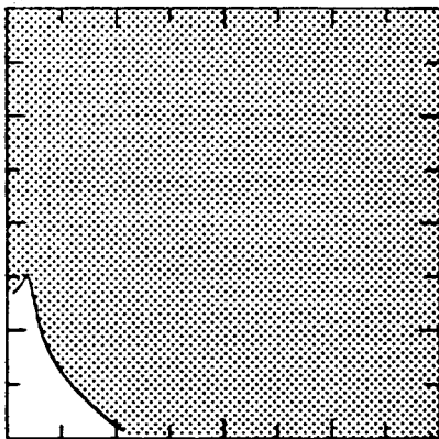
FIG. 4 Sparked ignition along the center line: F(\kappa) = 0.1
