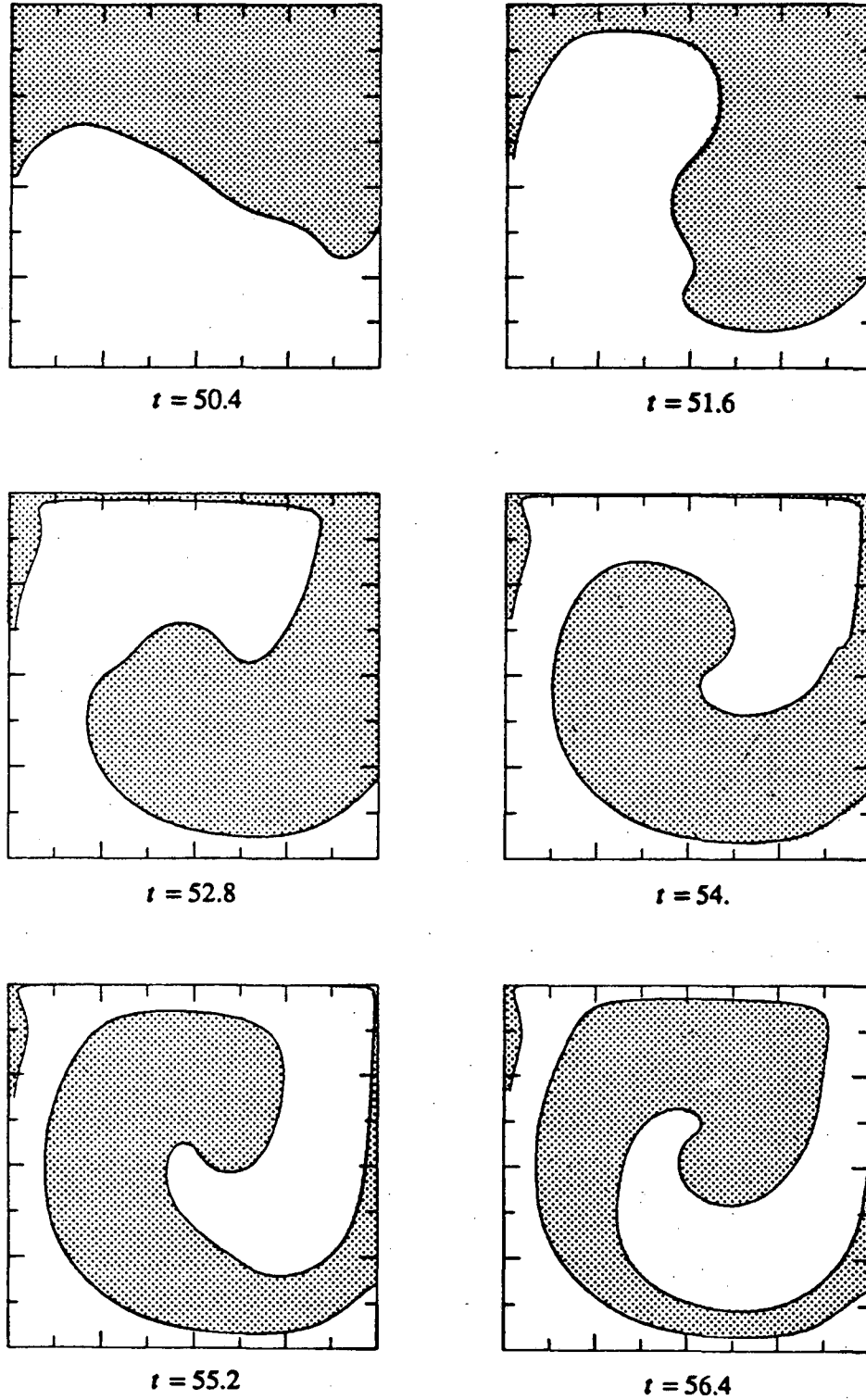
FIG. 3 Passive advection: F(\kappa) = 0
