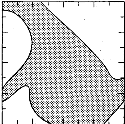
FIG. 9 Constant ignition at the center: F(\kappa) = 0.2 - 0.01\kappa
