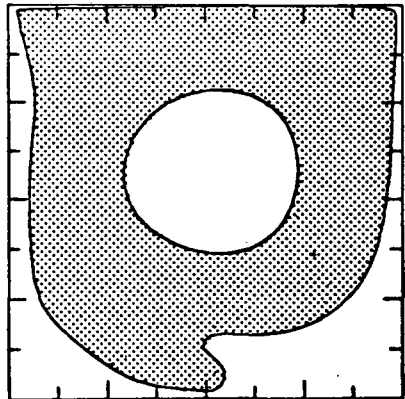
FIG. 2 Constant ignition at a bottom point: F(\kappa) = 0.01 - 0.01\kappa
