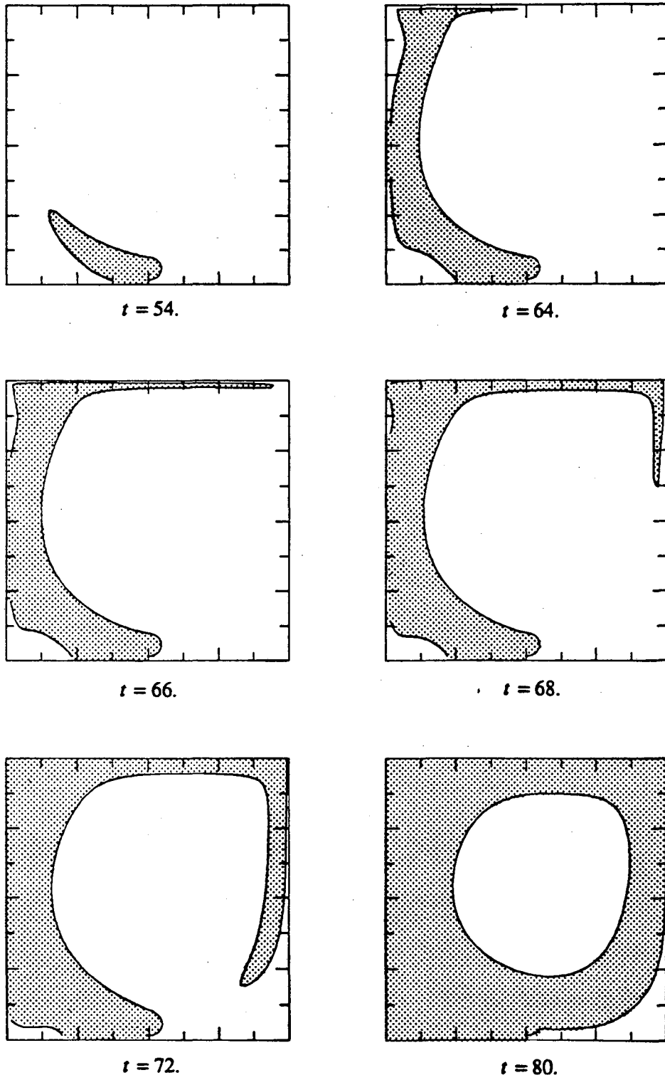
FIG. 1 Constant ignition at a bottom point: F(\kappa) = 0.01
