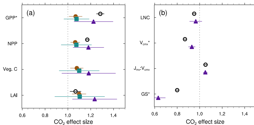
Figure 6. Observed (open circles) and simulated (solid shapes) effect size of \text{CO}_2 enrichment on various ecosystem carbon and leaf traits. Observations, where available, show the mean ( \pm 95\% confidence interval; Ainsworth & Long, 2005). Modeled responses show the global mean of grid cell effect sizes ( \pm 50\% prediction interval) for versions 4, 4.5, and 5 of CLM (brown circles, turquoise squares, and purple triangles, respectively), calculated using cells with mean GPP > 100 \text{ g C m}^{-2} \text{ yr}^{-1} . The vertical dashed line represents no effect. Variables listed include (a) gross and net primary productivity (GPP and NPP), vegetation carbon pools (Veg C), leaf area index (LAI) and (b) leaf N content (LNC), maximum carboxylation rates ( V_{\text{cmx}} ), the ratio of maximum electron transport rates ( J_{\text{mx}} ) to V_{\text{cmx}} , and stomatal conductance (GS). Asterisk denotes values for the mean of daily maximum rates.
