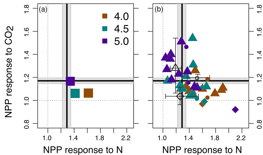
Figure 7. Simulated effect sizes of nitrogen versus \text{CO}_2 enrichment on rates of net primary productivity (NPP) that was calculated (a) globally or (b) for each plant functional type in CLM4, 4.5, and 5 (brown, turquoise, and purple symbols, respectively). In both panels, observational constraints for the nitrogen response (aboveground NPP from LeBauer and Treseder (2008)) and \text{CO}_2 response (dry matter production from Ainsworth and Long (2005)) are shown with the vertical and horizontal lines, respectively (mean \pm 95% confidence interval). The right panel shows the observed (open symbols) and simulated (filled symbols) effect sizes of individual plant functional types for woody vegetation, \text{C}_3 grasses, and \text{C}_4 grasses (triangles, circles, and diamonds, respectively).
