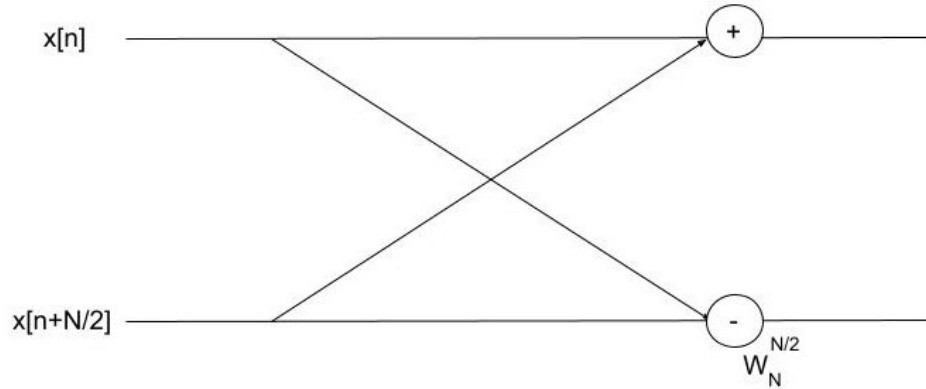
Figure 3.3: Butterfly operation
