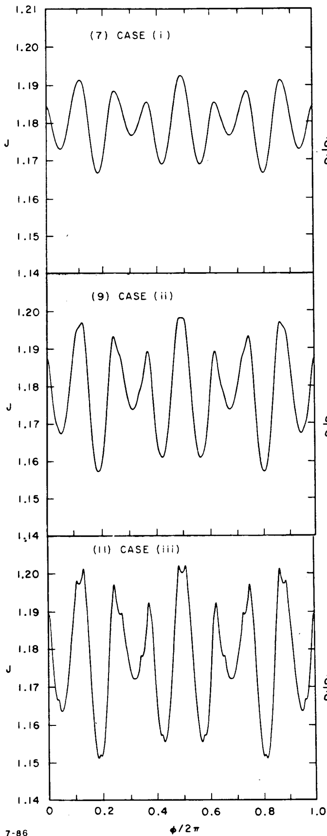
Figures 7,9,11: Invariant KAM curves J(\phi, \theta = 0) . Figures 8,10,12: The Jacobians \partial\psi/\partial\phi = \partial J/\partial\kappa at \theta = 0 . Cases (i) - (iii) are for increasing resonance widths.
