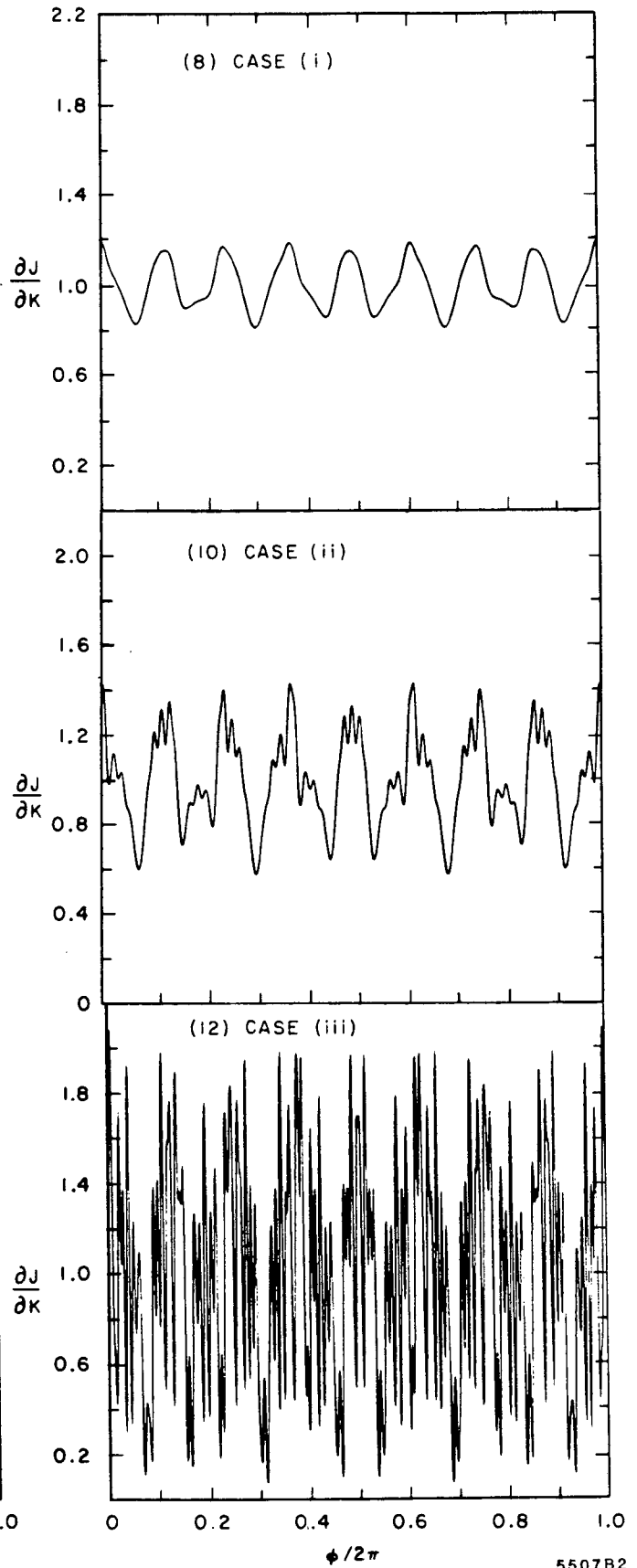
Figures 7,9,11: Invariant KAM curves J(\phi, \theta = 0) . Figures 8,10,12: The Jacobians \partial\psi/\partial\phi = \partial J/\partial\kappa at \theta = 0 . Cases (i) - (iii) are for increasing resonance widths.
