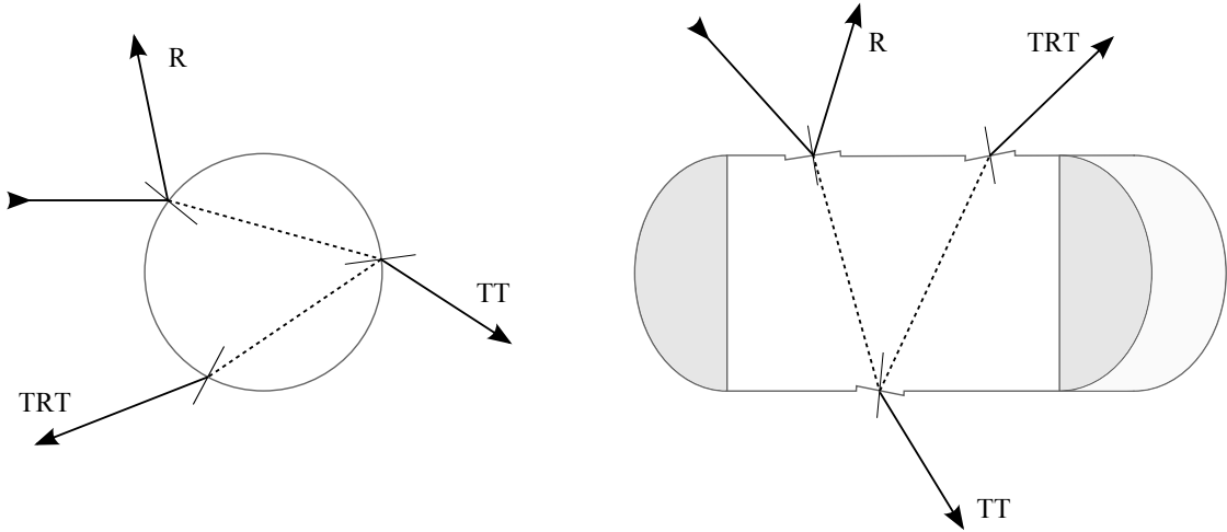
Figure 4.5: Light reflections off of a cylindrical hair fiber in the azimuthal (left) and longitudinal (right) directions. Tilted cuticles on the surface of the hair fiber deviate the direction of light reflections and refractions and cause the separation of primary (R) and secondary (TRT) highlights.
