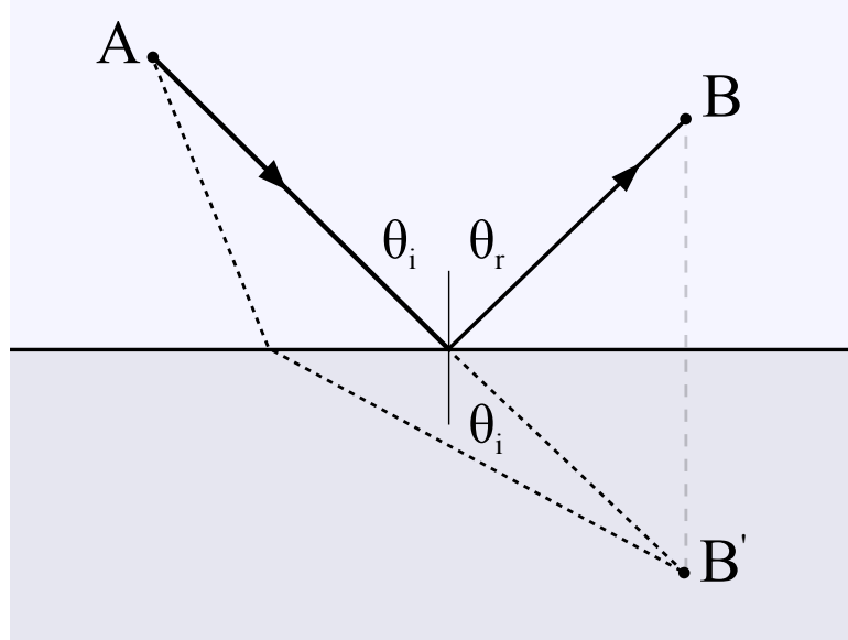
Figure 2.5: The geometry of light reflection as it goes from point A to point B . Using Fermat's principle, one can show that the reflected angle \theta_r is equal to the incident angle \theta_i .
