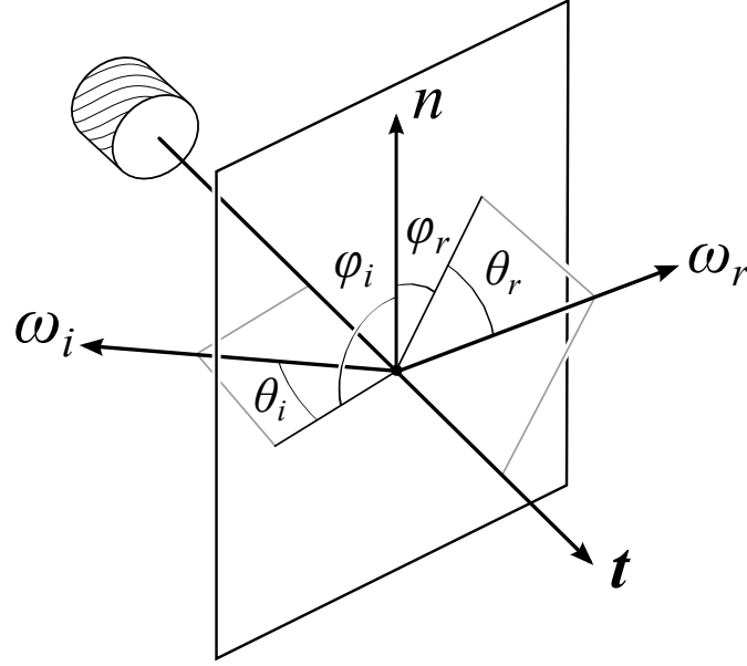
Figure 5.4: Notations and geometry of light reflection from a cylindrical fiber. Longitudinal angles \theta are computed with respect to the normal plane and the azimuthal angles \phi are computed based on the local surface normal direction n . When the thread is not part of a fabric n can be any arbitrary direction within the normal plane.
