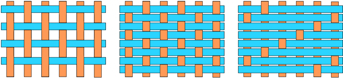
Figure 5.3: Different weaving patterns of the fabrics shown in Figure 5.2: (left) Plain, (middle) Crepe de Chine, and (right) Satin Charmeuse.
