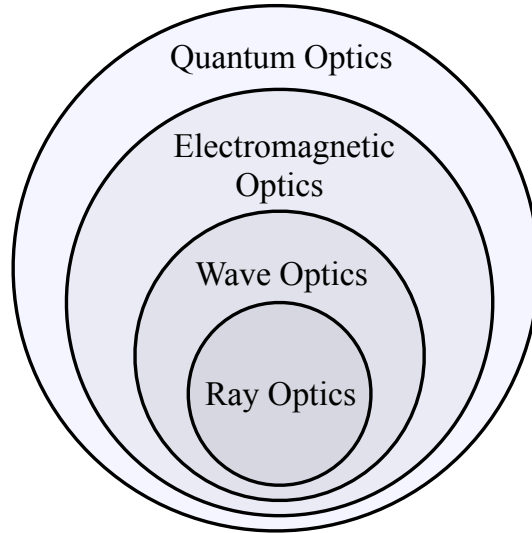
Figure 2.1: Different optical models for describing the nature of light. The theory of quantum optics is the most complete optical model to date. It subsumes electromagnetic optics, which in turn, subsumes wave optics. Ray optics is the simplest and the most widely used model in computer graphics.
