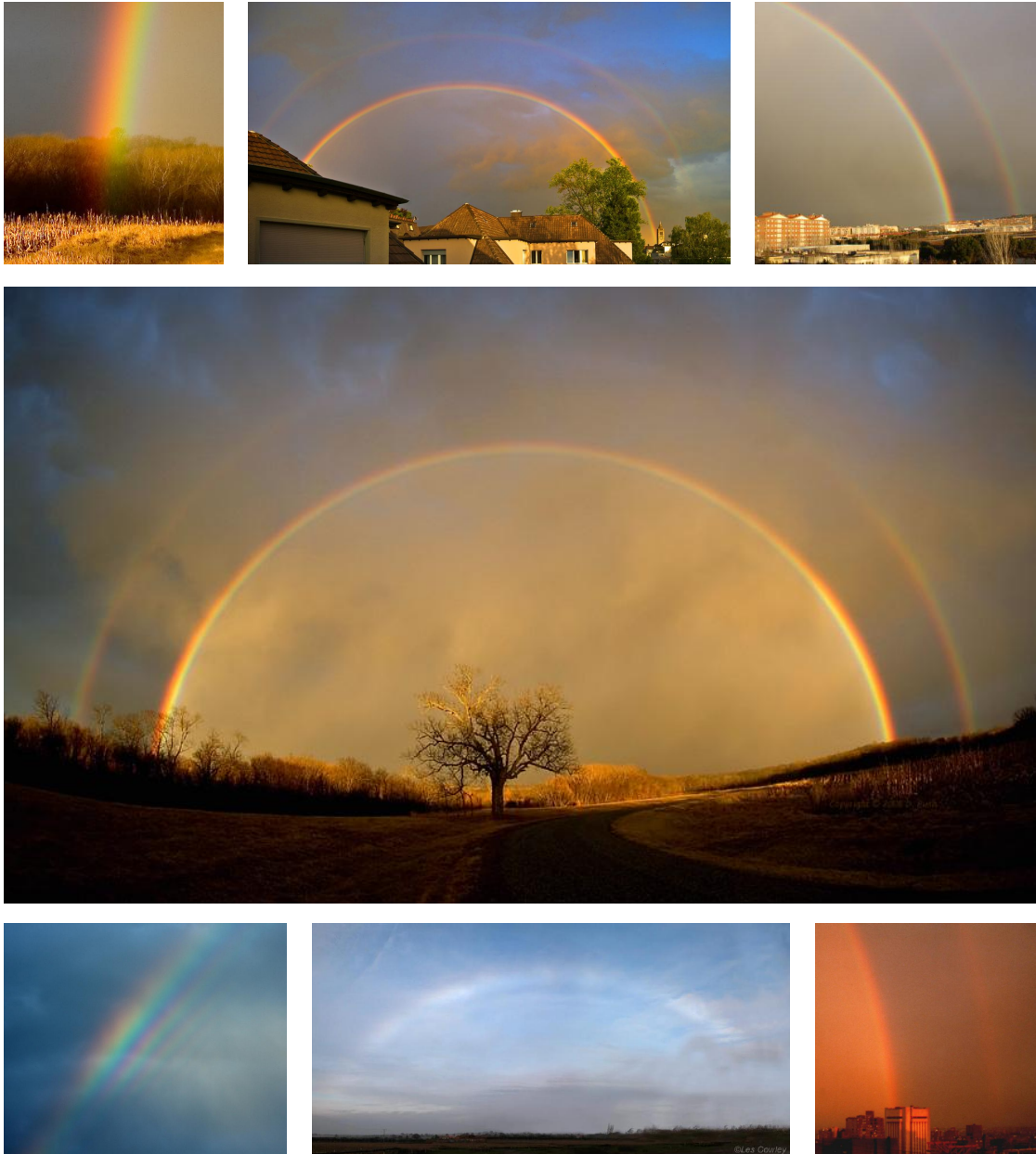
Figure 3.2: Different rainbows seen in nature. From top to bottom right to left: Primary rainbow, reproduced with permission © Dan Bush [Bus]. Double rainbow (primary and secondary rainbows). Alexander’s dark band. Double rainbow, reproduced with permission © Dan Bush [Bus]. Supernumerary bows, reproduced with permission © Ian Goddard [God]. Cloud bow, reproduced with permission © Les Cowley [Cowb]. Red bow.
