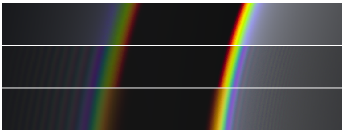
Figure 2.8: Effect of different optical phenomena on the appearance of rainbows: (top) dispersion, (middle) dispersion plus interference, (bottom) dispersion plus interference plus diffraction.
