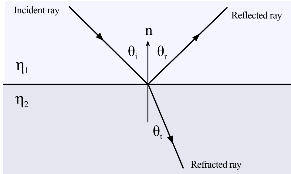
Figure 2.4: The geometry of the reflection and refraction of light: The incident ray has angle \theta_i with respect to the surface normal \vec{n} . the reflected and refracted rays have angle \theta_r and \theta_t respectively.
