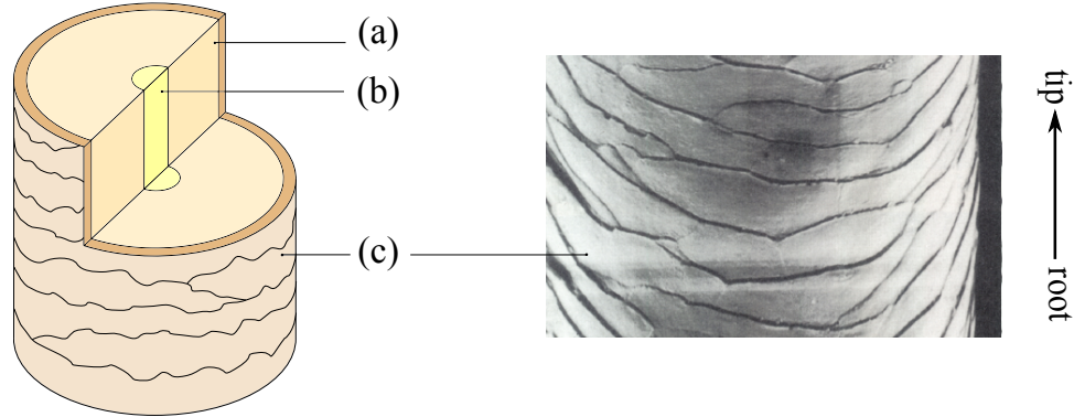
Figure 4.3: The structure of human hair fibers. Human hair consists of three main components: (a) the cortex, (b) the medulla, and (c) the cuticle. To the right is an electron micrograph of a hair fiber showing the structure of the cuticle layer. In this image the fiber is oriented with the root at the bottom and the tip at the top. The micrograph image is reprinted from [Rob94].
