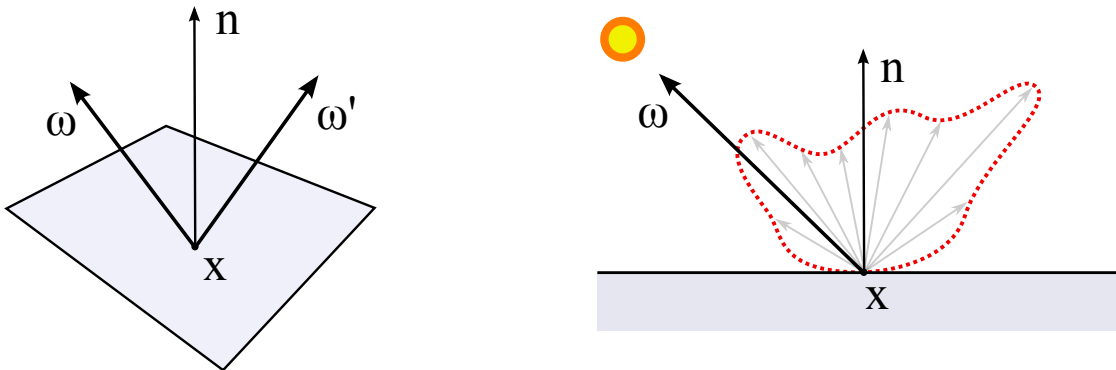
Figure 2.14: (left) The BRDF expresses the reflection profile from a point on the surface for any pair of viewing and lighting directions. (right) An example BRDF and its response to the incoming light direction \vec{\omega} .
