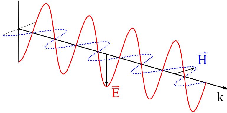
Figure 2.3: Electromagnetic wave is a paired couple of vector waves: an electric wave vector \vec{E} and a magnetic wave vector \vec{H} . These two wave vectors are perpendicular to the direction of wave vector \vec{k} .
