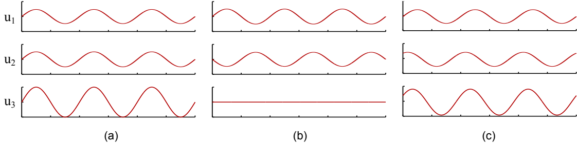
Figure 2.9: Different types of interference: (a) constructive, (b) destructive, and (c) the general case.
