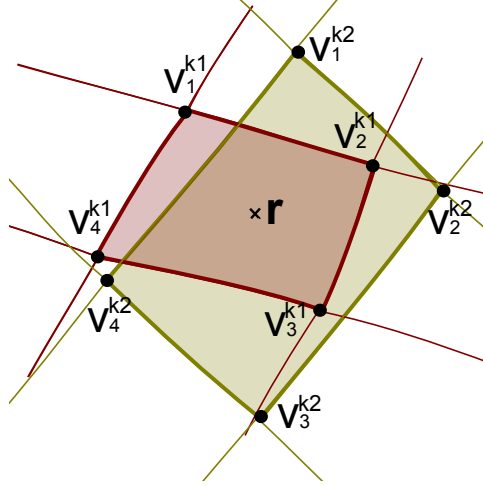
Figure 3.13: Direction \mathbf{r} intersects patches k1 (red) and k2 (yellow) (two parts of two different wavefronts). At each of both patches, bilinear interpolation from all the corners v_i^k result into an interpolated electromagnetic wave per patch. Interference is then computed by combining (adding) all the interpolated electromagnetic waves.
