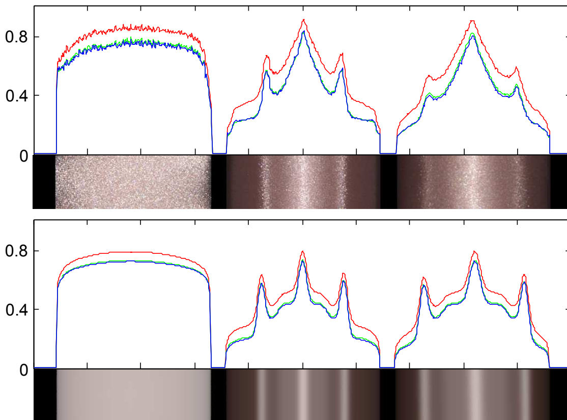
Figure 5.27: Photograph and the rendering result for the front side of Polyester Satin Charmeuse fabric.
