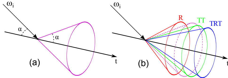
Figure 4.7: Evolution of longitudinal functions: (a) Kajiyá and Kay defined the reflection cone and it was used by Goldman and Kim in their shading model. (b) Marschner et al. introduced the separation of different scattering components on three different cones. Their longitudinal scattering function was later used by Zinke.
