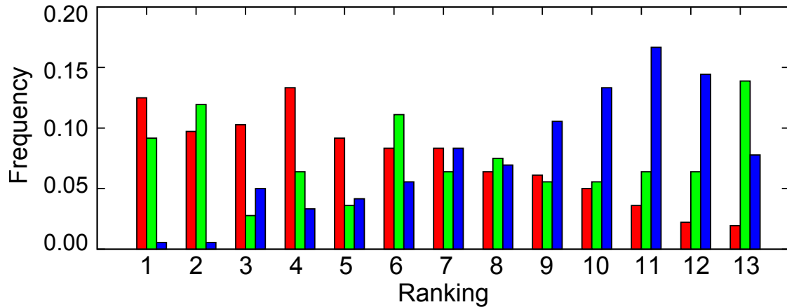
Figure 4.28: Normalized distribution of the rankings for all the shading models (1 is best, 13 is worst). The New shader (red) is generally ranked better than the Research shader (blue) while the Production shader (green) is somewhat inconsistent with really good results and some not so good. The numbers have been normalized based on the number of samples in each group.
