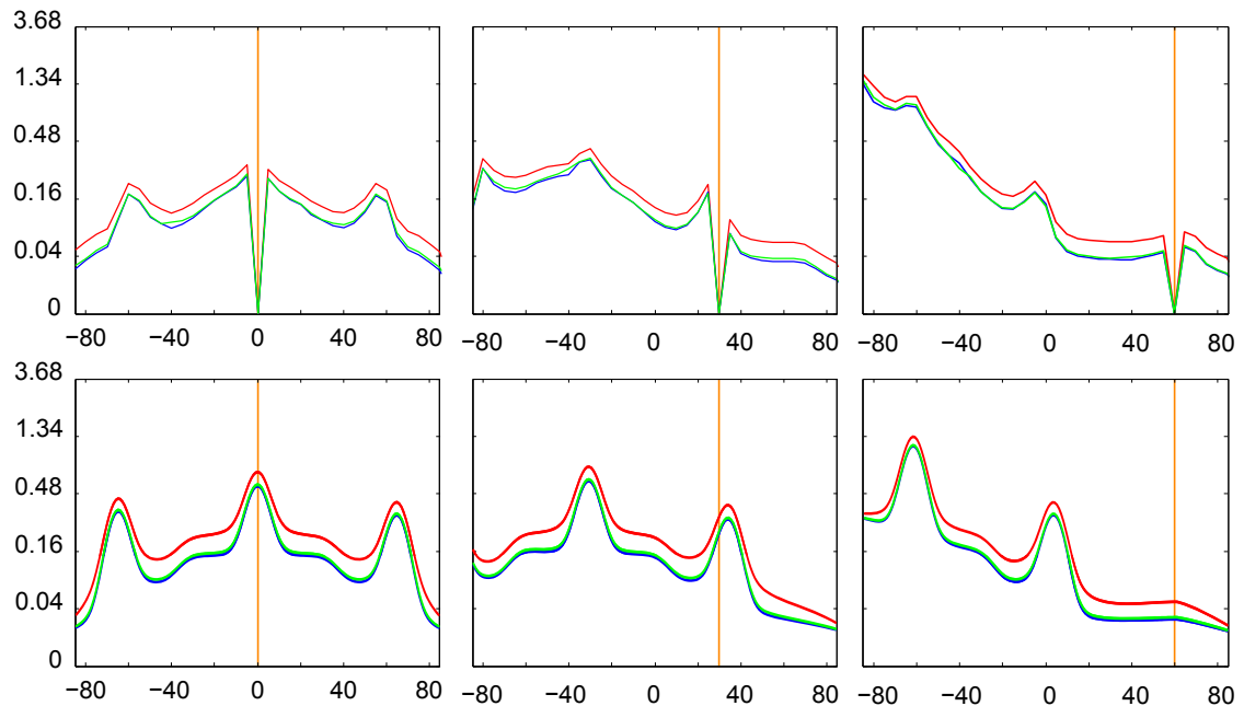
Figure 5.29: Matching a BRDF measurement of the Polyester Satin Charmeuse fabric with our model. (top) normal plain BRDF measurement of the front side of Polyester Satin Charmeuse fabric along the direction of flat threads compared to (bottom) the result of our appearance model.
