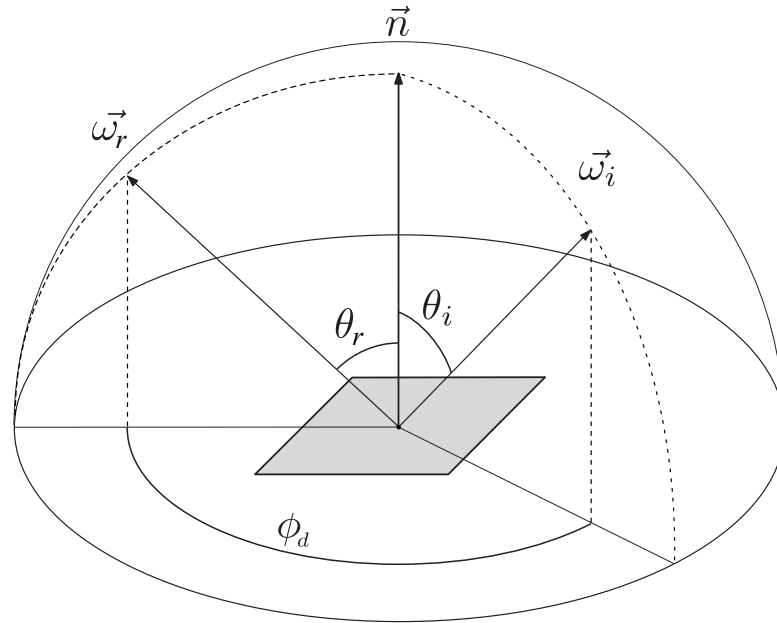
Figure 5.9: An illustration of the acquisition setup and coordinate system for measuring cloth.
