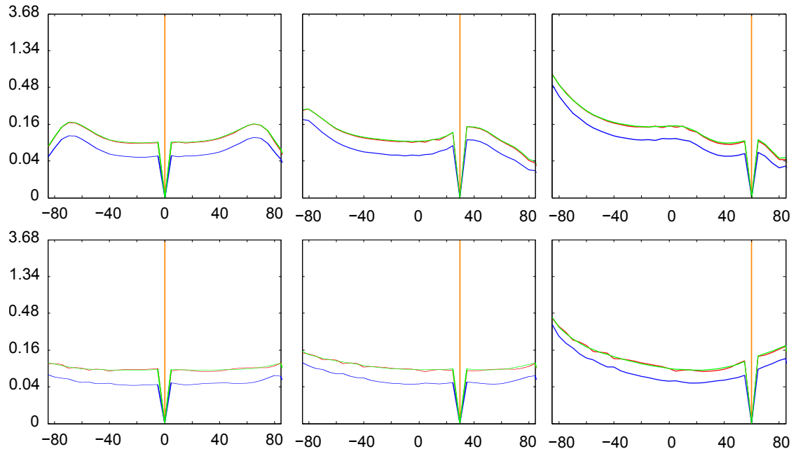
Figure 5.13: BRDF measurements for Silk Crepe de Chine for 0^\circ , 30^\circ , and 60^\circ incident angle. The top row corresponds to the in plane measurements parallel to the direction of flat threads, and the bottom row represents the measurements in the perpendicular direction.
