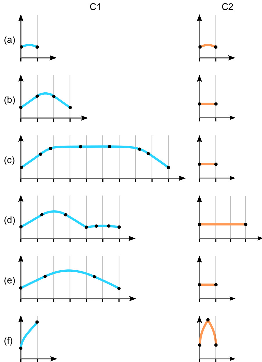
Figure E.1: The tangent curves of all fabrics presented in our cloth appearance model. The tangent curves are for (a) Linen Plain, (b) Silk Crepe de Chine, (c) front face of Polyester Satin Charmeuse, (d) back face of Polyester Satin Charmeuse, (e) Silk Shot fabric, and (f) Velvet. The numerical values are listed in Table E.1.
