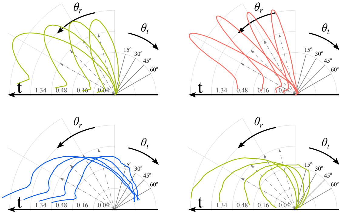
Figure 5.18: Polar plots of measured incidence plane BRDF for different threads. Each quadrant of the figure contains the RGB average BRDF for a thread type. Starting at the top row, and moving left to right we have flat silk thread, flat polyester thread, twisted linen thread, and twisted silk thread.
