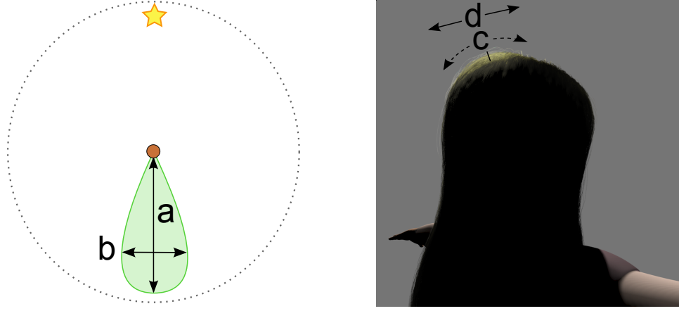
Figure 4.16: Visualizing the transmission component's control parameters on the corresponding azimuthal scattering function (left) and a backlit rendering (right). (a) The intensity I_{TT} , (b) the azimuthal width \gamma_{TT}^2 , (c) the longitudinal shift \alpha_{TT} , and (d) the longitudinal width \beta_{TT}^2 of the transmission highlight.
