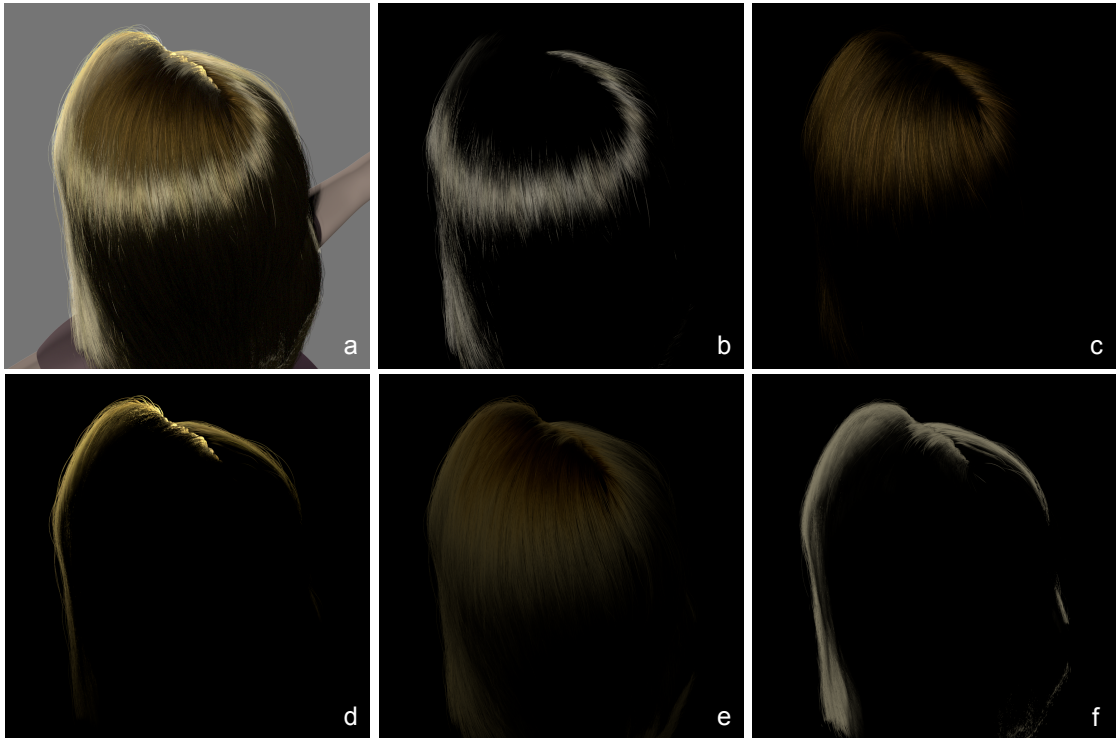
Figure 4.19: Visualizing the decomposed components of our hair shading model. (a) Final rendering result. (b) Primary highlight component R' , (c) secondary highlight component TRT' , (d) transmission component TT' , (e) backscattering component B.S.' , and (f) forward scattering component F.S.' .
