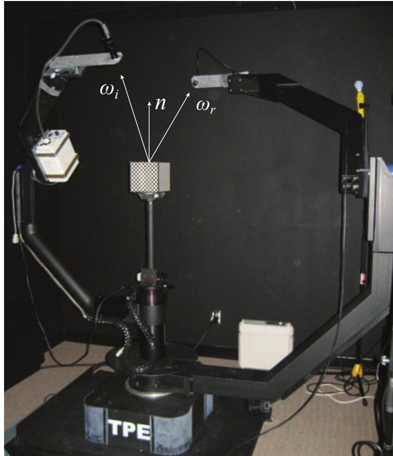
Figure 5.8: Gantry facility at University of California, San Diego. This device is a fully automatic, four-axis image-based gonioreflectometer.
