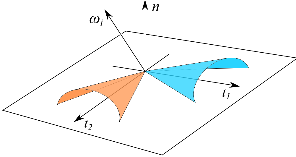
Figure 5.21: Our shading model treats the fabric as a mesh of microcylinders oriented in two orthogonal directions.
