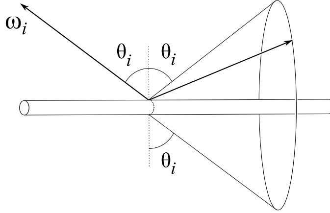
Figure 5.19: Reflection cone off of a smooth cylinder. The reflected rays lie on a cone centered around the tangent direction of the cylinder.
