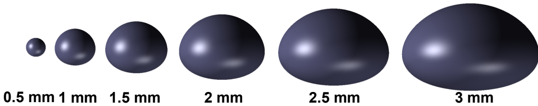
Figure 3.8: Nonspherical raindrop shape with increasing radii as proposed by Beard and Chuang [BC87].
