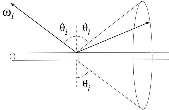
Figure 4.4: Reflection cone from a smooth cylinder. Kajiya and Kay pointed out that light reflections off of a cylinder form a cone.
