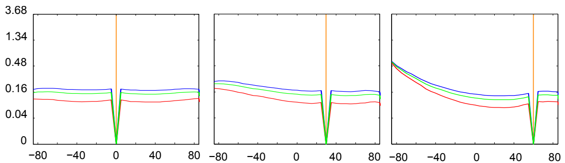
Figure 5.11: BRDF measurements for Linen Plain for 0^\circ , 30^\circ , and 60^\circ incident angles.
