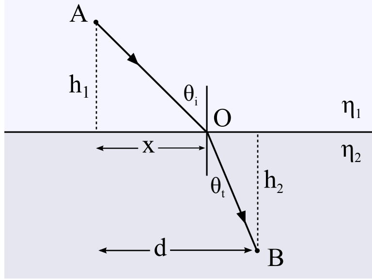
Figure 2.6: The geometry of light refraction as it goes from point A to point B . Using Fermat's principle, one can show that the refracted angle \theta_t and the incident angle \theta_i follow Snell's law.
