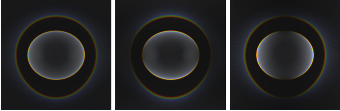
Figure 3.19: The effect of the different polarization states on the perception of a rainbow from 0.5mm radius non-spherical water drop: (left) circular, (middle) horizontal, and (right) vertical polarizations.
