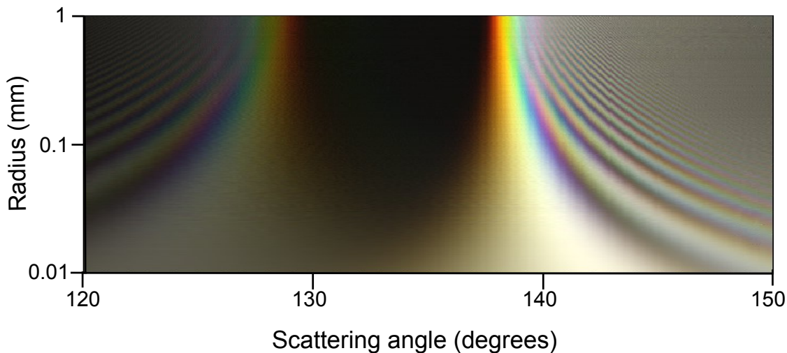
Figure 3.10: Lee diagram showing the variation in appearance of primary and secondary rainbows caused by scattering of sunlight by a spherical water drop as a function of radius (Lorenz-Mie theory calculations).
