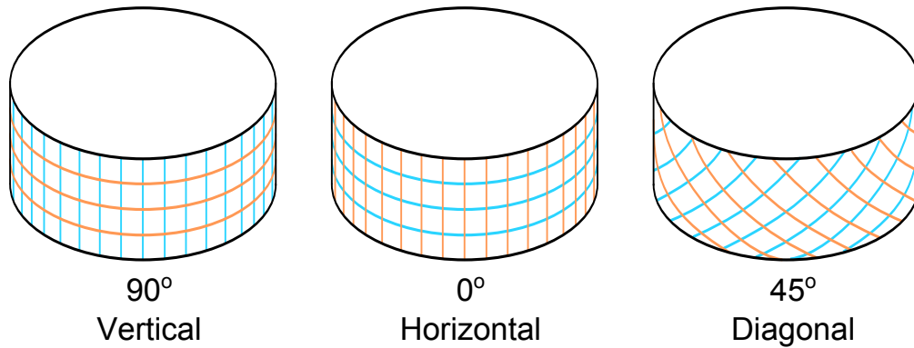
Figure 5.24: To capture the anisotropic behavior of different fabrics, we have wrapped the fabric around a cylinder in three different orientations where the flat threads stay (left) vertical, (middle) horizontal, and (right) diagonal.
