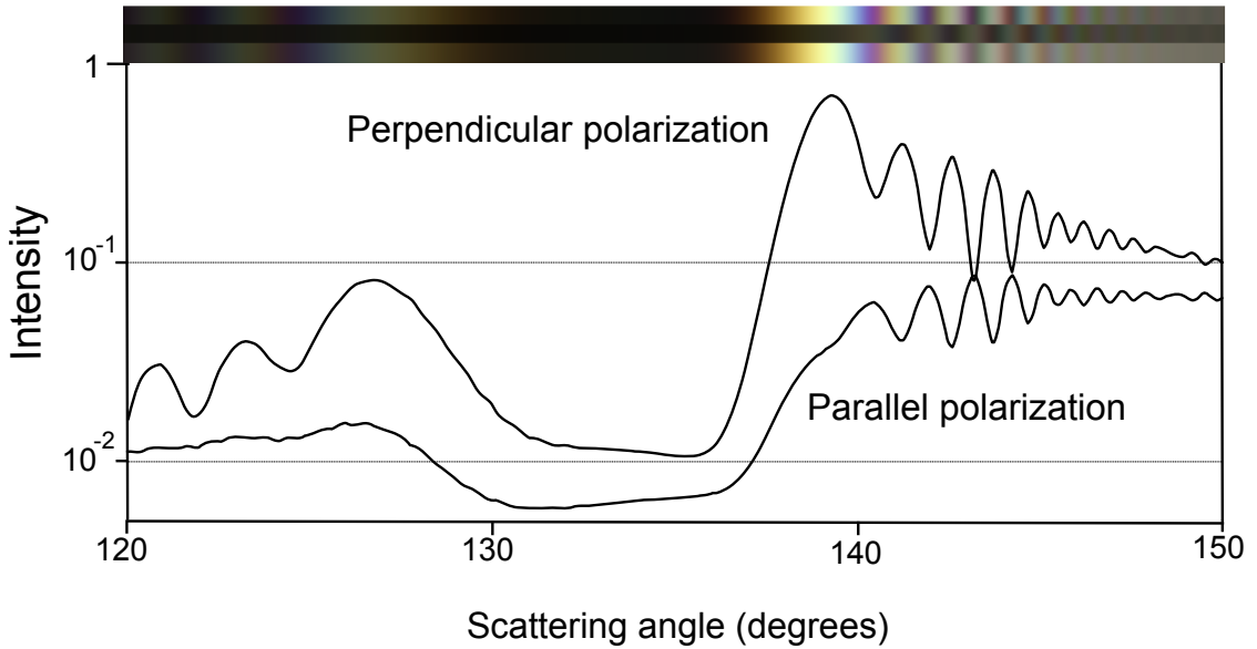
Figure 3.7: Graph of intensity as a function of scattering angle for the primary rainbow caused by scattering of sunlight by a spherical drop of water of radius 0.1\text{ mm} . The color stripes on top represent, from top to bottom, the phase function for perpendicular polarization, parallel polarization and unpolarized light, respectively.
