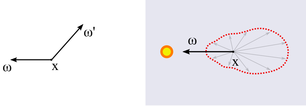
Figure 2.15: (left) Phase function expresses the angular distribution of light scattering at a given point inside a medium. (right) An example phase function and its response to the incoming light direction \vec{\omega} .
