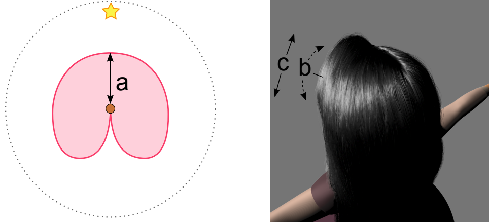
Figure 4.15: Visualizing the primary highlight’s control parameters on its corresponding azimuthal scattering function (left) and a frontlit rendering (right). (a) The intensity I_R , (b) the longitudinal shift \alpha_R , and (c) the longitudinal width \beta_R^2 of the primary highlight.
