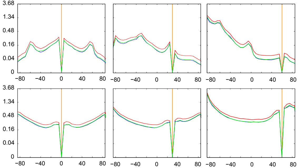
Figure 5.16: BRDF measurements for Polyester Charmeuse for 0^\circ , 30^\circ , and 60^\circ incident angles. Top row corresponds to in plane measurements along the direction of flat threads, and the bottom row represents measurements in the perpendicular direction.
