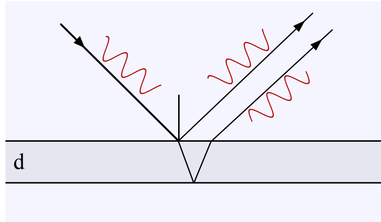
Figure 2.10: Thin film interference of light. The light gets reflected off the external and internal surfaces of a thin film. The reflected lights have a phase difference causing them to interfere.
