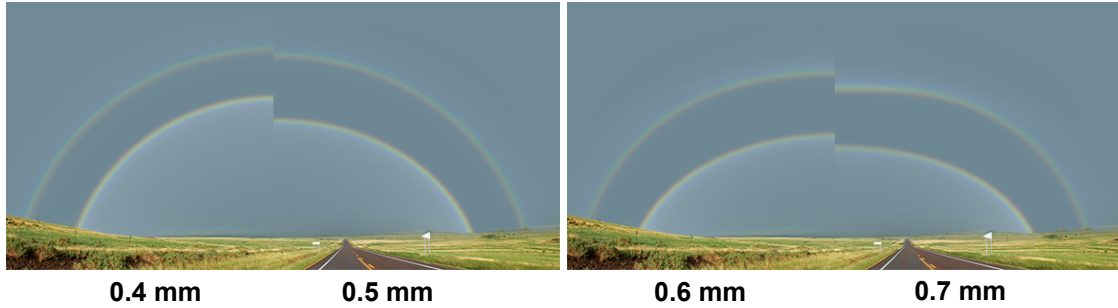
Figure 3.17: The effect of different water drop radii on the apparent geometry of the rainbow.
