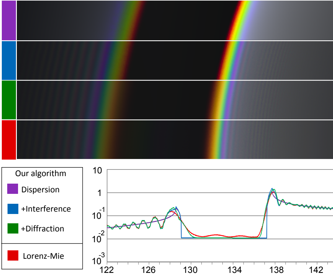
Figure 3.12: Comparison between the different phenomena simulated by our method (dispersion, interference and diffraction) and the same simulation from the Lorenz-Mie theory, for a 0.4mm radius spherical water drop. Top: Renderings for 33 wavelength. Bottom: Graphs for 650nm wavelength.
