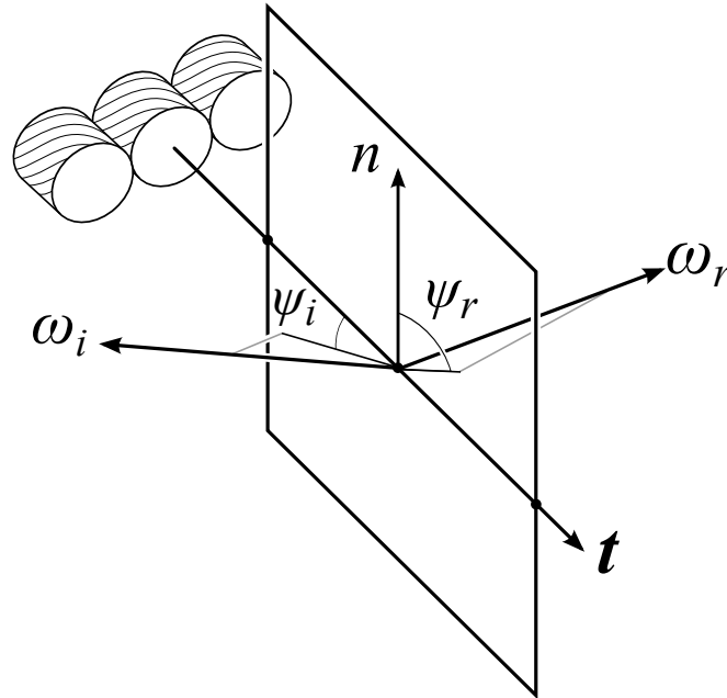
Figure 5.5: Longitudinal angles \psi_i and \psi_r are the angles between local surface normal n and the projection of \omega_i and \omega_r on to the plane spanned by vectors t and n .
