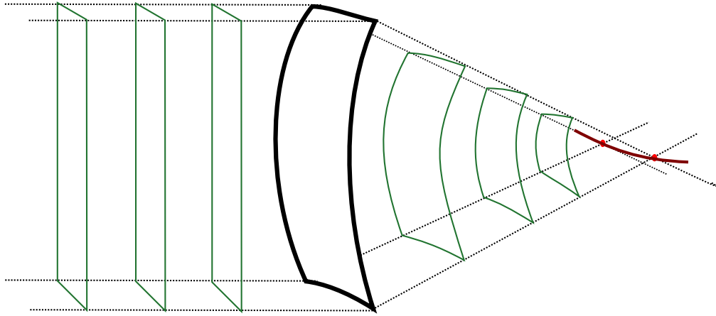
Figure 3.6: A focal line defines the curve along which all the differential focal points of the wavefront lie. The thick black represents a portion of the surface of the water drop. The green patches represent the wavefront itself. Notice how they converge to the red line, which is the focal line.
