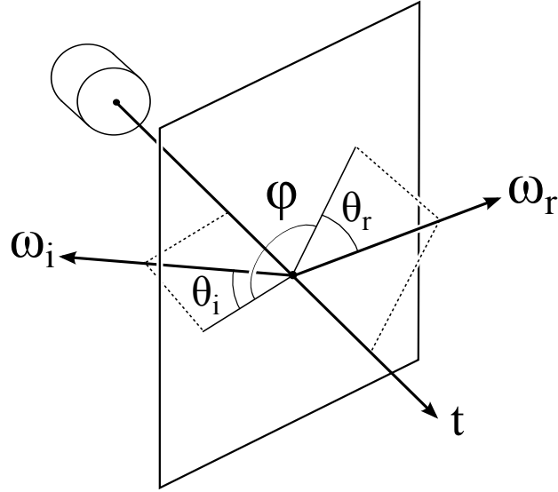
Figure 4.2: The geometry notations used for describing the light scattering from cylinders.
