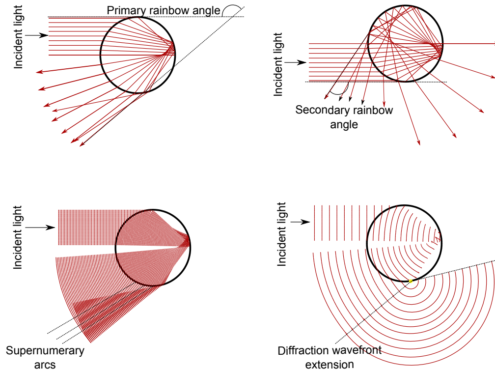
Figure 3.5: Generation of rainbows from the point of view of geometric and wave optics: (a) primary rainbow angle, after a single internal reflection, (b) secondary rainbow angle, after two internal reflections, (c) supernumerary rainbows are generated from constructive and destructive interference patterns (inspired by Lee and Fraser [LF01]), (d) diffraction extends the wavefront and avoids abrupt intensity changes.
