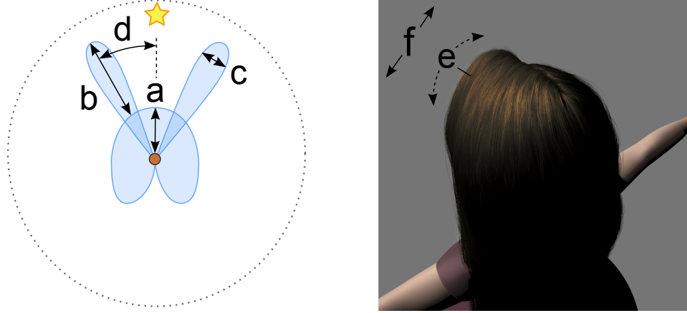
Figure 4.17: Visualizing the secondary highlight’s control parameters on the corresponding azimuthal scattering function (left) and a frontlit rendering (right). (a) The intensity of the secondary highlight I_{TRT} , (b) the relative intensity of glints I_g , (c) the azimuthal width of the glints \gamma_g^2 , (d) the half angle between the glints G_{angle} , (e) the longitudinal shift \alpha_{TRT} , and (f) the longitudinal width \beta_{TRT}^2 of the secondary highlight.
