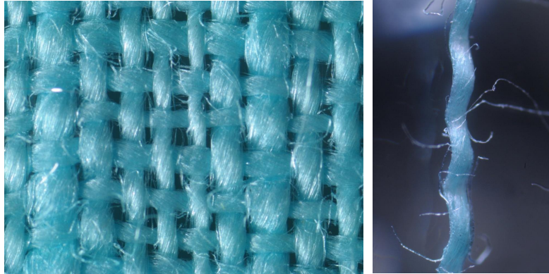
Figure 5.10: Microscope pictures of the Linen Plain fabric. The fabric (left) is made from one type of thread (right) with varying thicknesses.
