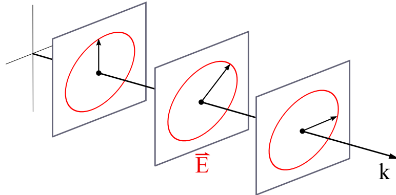
Figure 2.13: Polarization state of the light is perpendicular to the direction of the wave vector \vec{k} .
