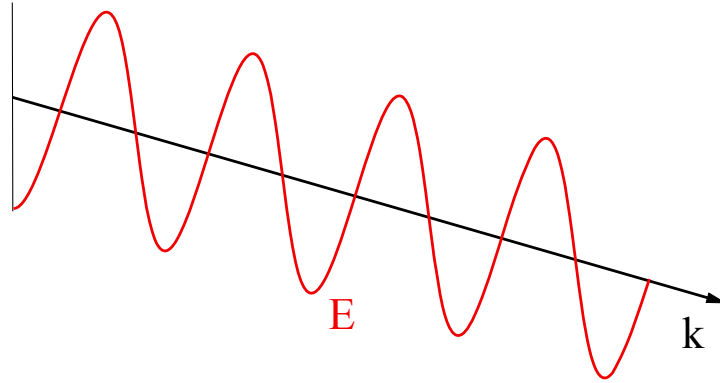
Figure 2.2: Electric wave E is a scalar function that oscillates perpendicular to the direction of its propagation \vec{k} .
