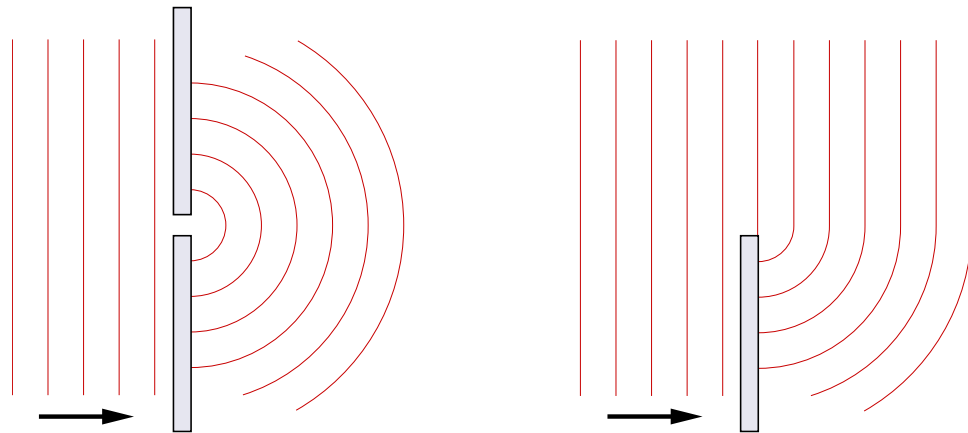
Figure 2.12: Diffraction of light as it hits a surface with a small hole or a sharp edge. The arrow shows the propagation direction of the wave. Every point of a wave serves as a point source of spherically symmetric waves.
