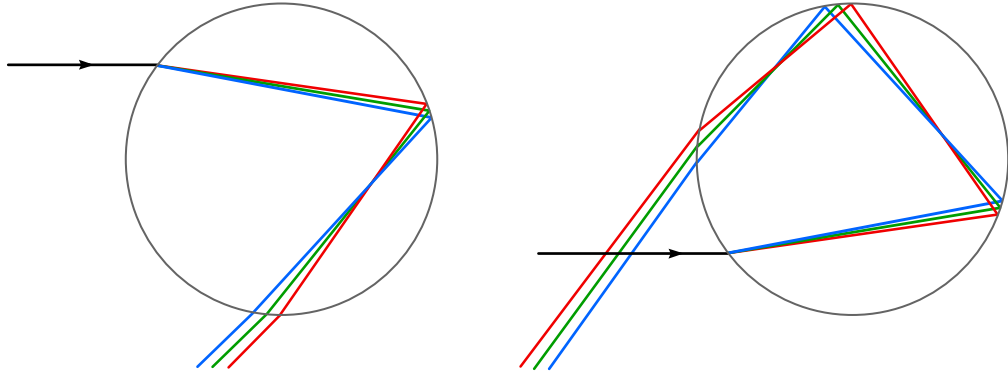
Figure 3.4: Dispersion of light as it gets reflected and refracted by the water drop causes the primary bow (left) and the secondary bow (right).
