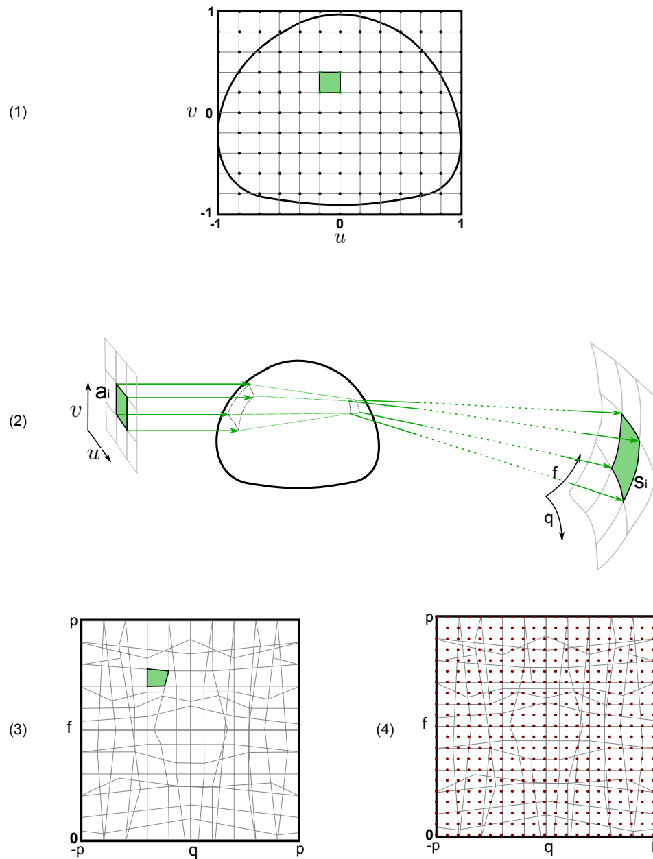
Figure 3.11: Steps of the algorithm. (1) Casting the grid of rays towards the particle. (2) Rays are reflected and refracted towards the water drop, forming patches. (3) Outgoing patches are collected in an infinite collecting sphere. (4) The stored patches in the collecting sphere are queried at specific directions, sampling the phase function.
