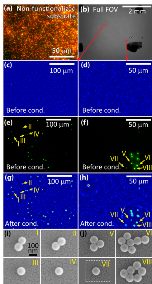
Figure 3. Specific capture and wide-field imaging of individual biofunctionalized nanoparticles on a chip. (a) Conventional 40\times fluorescent microscope image of the bead mixture on a nonfunctionalized substrate. Many plain red 100 nm beads can be seen, as can a few streptavidin-coated green 110 nm beads. (b–j) Images of green streptavidin-coated beads specifically captured on biotinylated glass, mimicking the capture of virus-sized particles. (b) Full FOV holographic on-chip microscope image before deposition of vapor-condensed nanolenses. (c, d) Two regions of interest showing that beads cannot be detected without condensed nanolenses. (e, f) Conventional fluorescent 40\times objective microscope images showing specific capture of only streptavidin-coated beads. (g, h) Holographic images of the sample with vapor-condensed nanolenses showing particle detection. (i, j) SEM images that verify the sizes of the detected particle clusters. For all lens-free images, the working distance is z_2 \approx 280 \mu\text{m} .
