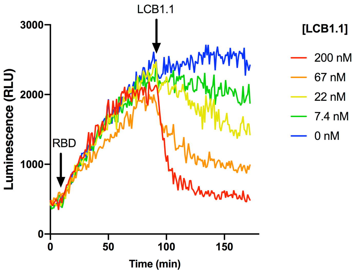
Extended Data Fig. 2 | Reversibility of lucCageRBD. Time-course luminescence of the lucCageRBD assay using 200 nM of RBD WT and different concentrations of the de novo LCB1.1 binder. All experiments were performed in triplicate, representative data are shown.
