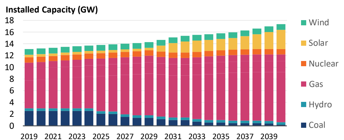
MODELED CAPACITY MIX EVOLUTION WITHOUT EE
