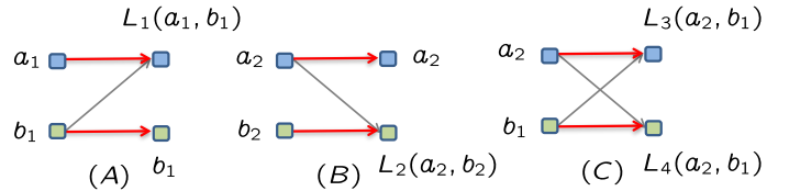
Fig. 2. A 2 user interference channel with topology alternating between the three states shown. Each topology by itself has sum-capacity 1, but joint coding across the alternating topologies achieves sum-rate 4/3 . L_i(x, y) represents a linear combination of x, y .
