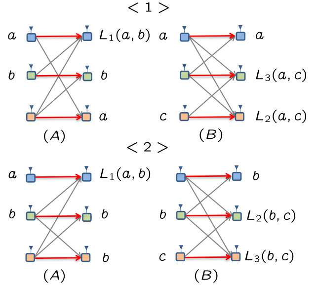
Fig. 4. Two examples of the 3 user interference channel with topology alternating between the two states shown. Example 1 is at the top of the figure and example 2 is at the bottom of the figure. Each topology by itself has sum-capacity 1, but joint coding across alternating topologies achieves sum-capacity 3/2 .
