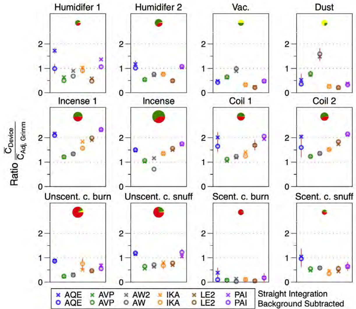
Figure 5. Ratios of event-integrated \text{PM}_{2.5} reported by each low-cost monitor to the estimated true event-integrated \text{PM}_{2.5} from WRAS adjusted by gravimetric data: mineral and combustion sources. Pie charts are sized proportionally to the estimated true \text{PM}_{10} integrated over the event with red, green and yellow corresponding to mass fractions of the following particle size ranges (in \mu\text{m} ): 10–2.5, 2.5–0.25, <0.25.
