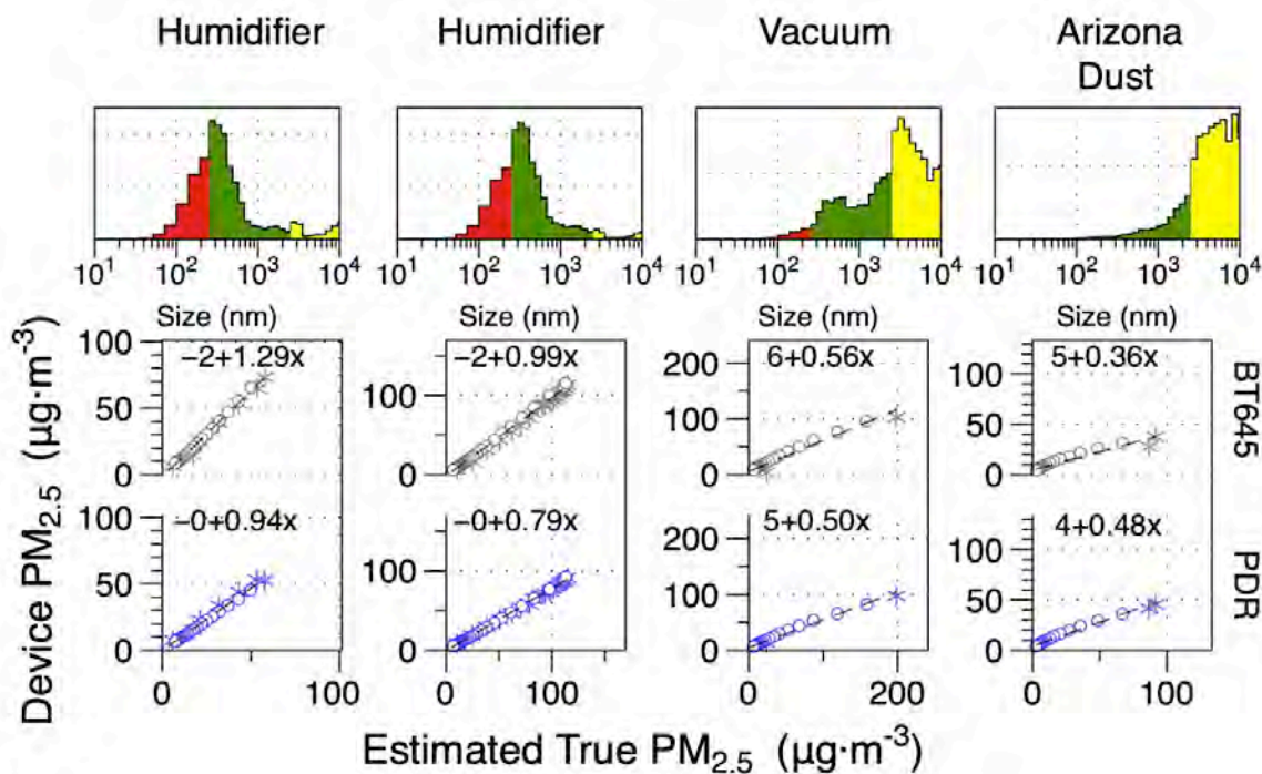
1 2 Figure S8. Correlations of 5-min average PM 2.5 reported for professional monitors with estimated 3 true PM 2.5 from WRAS adjusted to gravimetric data for mineral sources. 4
