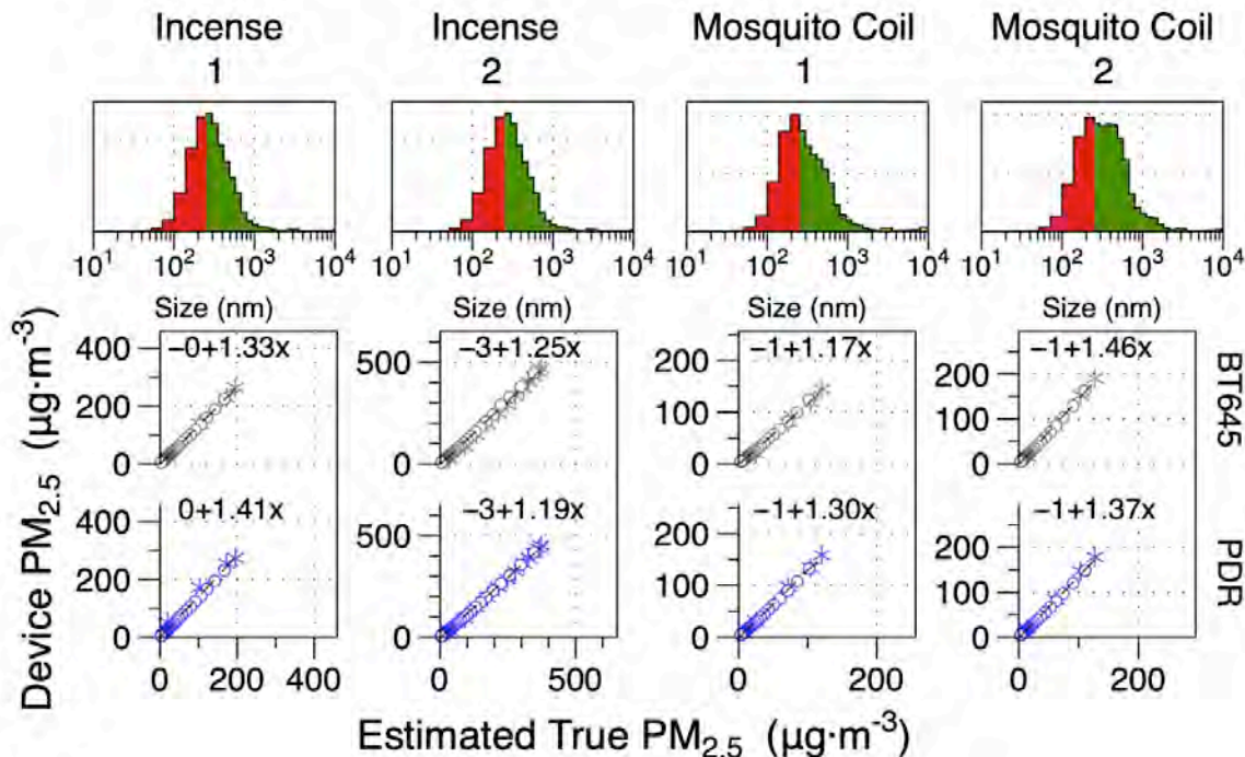
5 6 Figure S9. Correlations of 5-min average PM 2.5 reported for professional monitors with estimated 7 true PM 2.5 from WRAS adjusted to gravimetric data for incense and mosquito coil sources. 8
