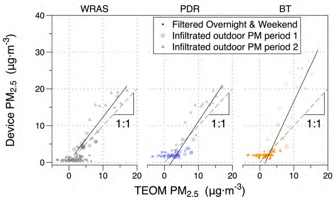
5 Figure S6. Hourly PM 2.5 reported by professional grade monitors and the TEOM during overnight 6 periods with the room open to outdoor air and no filtration and during no-source periods with 7 filtered supply air.
