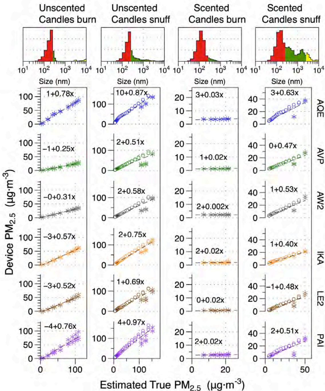
1 2 Figure 11. Correlations between 5-min average PM 2.5 reported by low-cost monitors and estimated 3 true PM 2.5 from WRAS adjusted to gravimetric data for candles under steady burn and after 4 being extinguished (snuff). Histograms at top show the distribution of PM mass over range of 10 5 nm to 10 \mu m. 6
