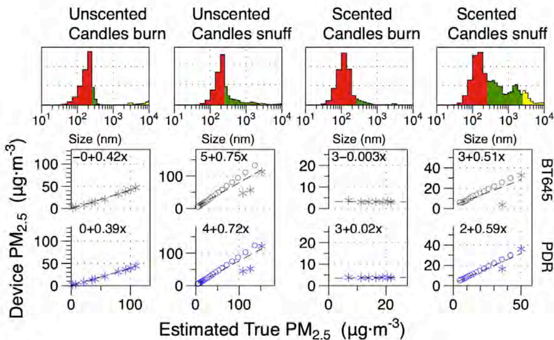
1 2 3 Figure S12. Linear correlations of 5-min average PM_{2.5} reported for professional monitors with estimated true PM_{2.5} from WRAS adjusted to gravimetric data for candles.
