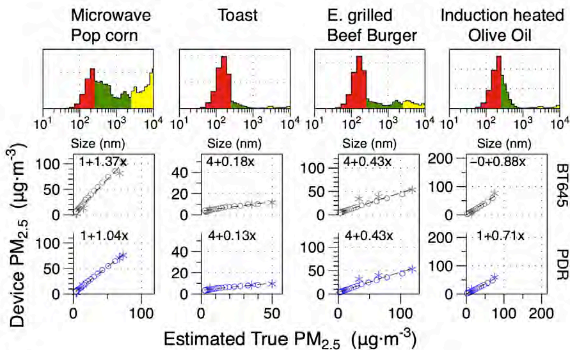
4 5 6 7 Figure S13. Linear correlations of 5-min average PM_{2.5} reported for professional monitors with estimated true PM_{2.5} from WRAS adjusted to gravimetric data for electric cooking.
