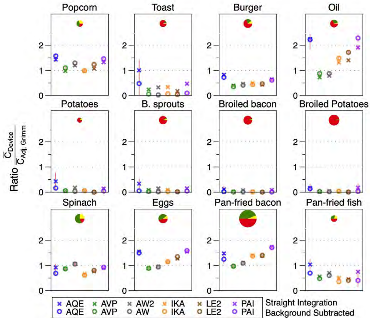
Figure 6. Ratios of event-integrated PM 2.5 reported by each low-cost monitor to the estimated true event-integrated PM 2.5 from WRAS adjusted by gravimetric data: cooking sources. Refer to Figure 5 caption for description of pie charts.
