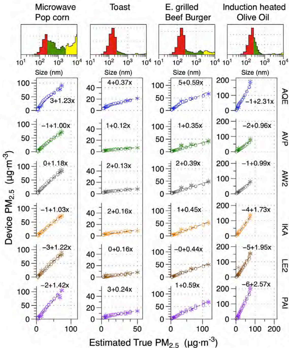
1 2 Figure 14. Correlations between 5-min average PM 2.5 reported by low-cost monitors and estimated 3 true PM 2.5 from WRAS adjusted to gravimetric data for electric cooking. Histograms at top show 4 the distribution of PM mass over range of 10 nm to 10 μm. 5
