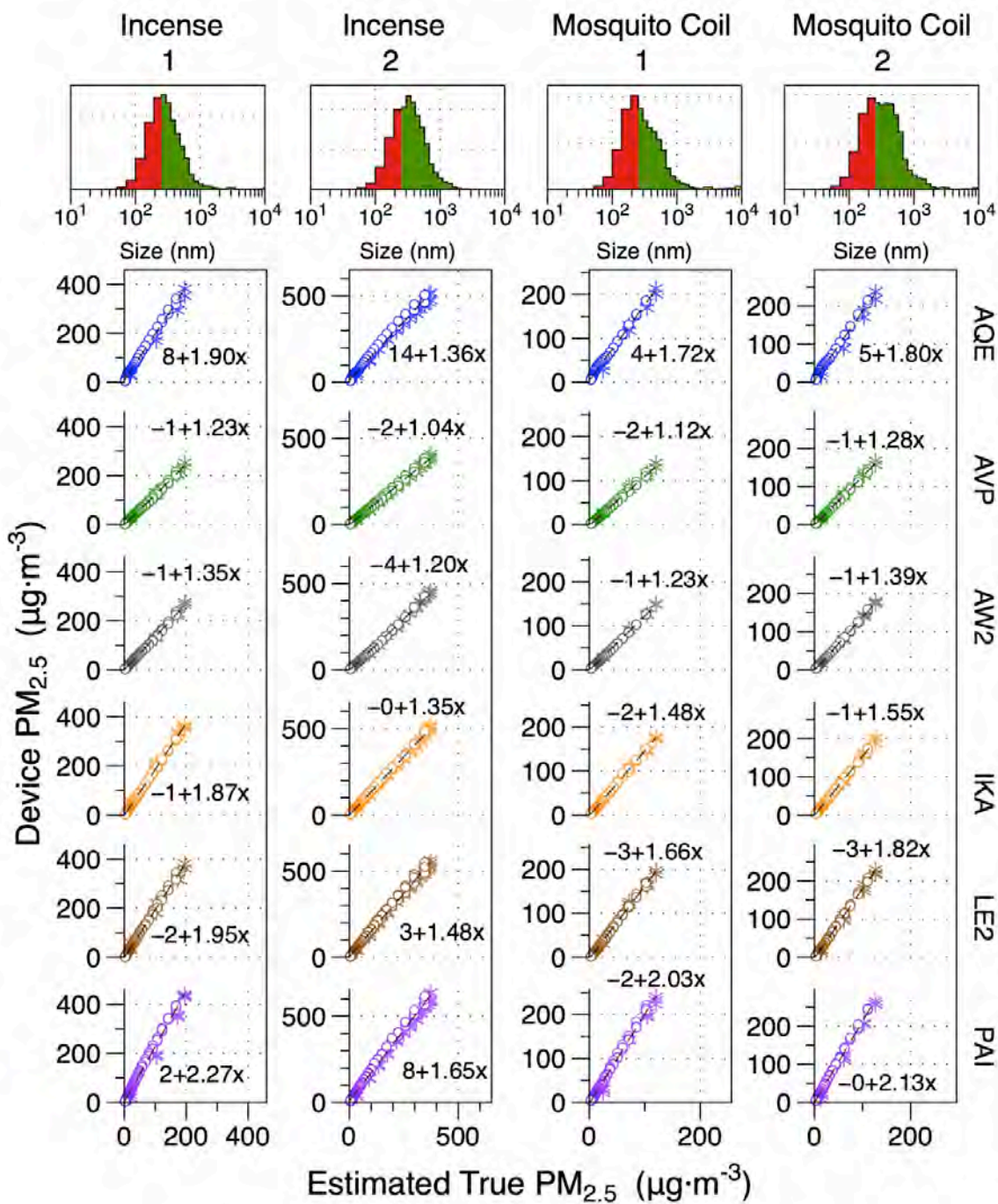
Figure S10. Correlations between 5-min average PM 2.5 reported by low-cost monitors and estimated true PM 2.5 from WRAS adjusted to gravimetric data for incense and mosquito coil. Histograms at top show the distribution of PM mass over range of 10 nm to 10 µm.
