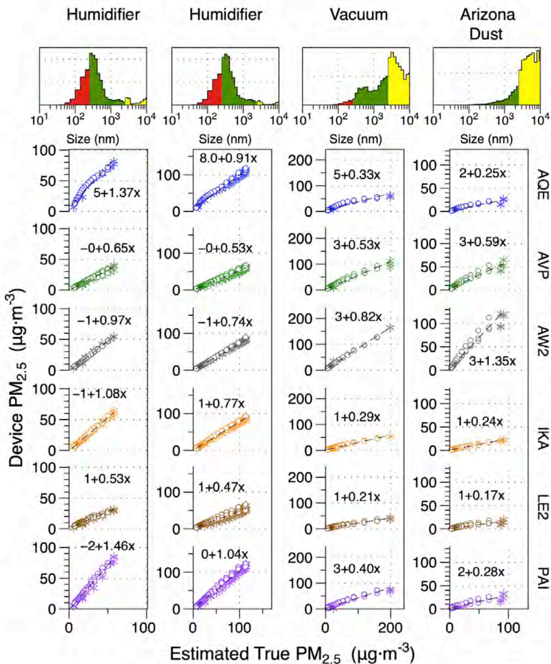
1 2 Figure S7. Correlations between 5-min average PM 2.5 reported by low-cost monitors and estimated 3 true PM 2.5 from WRAS adjusted to gravimetric data for mineral sources. Histograms at top show 4 the distribution of PM mass over range of 10 nm to 10 µm. 5
