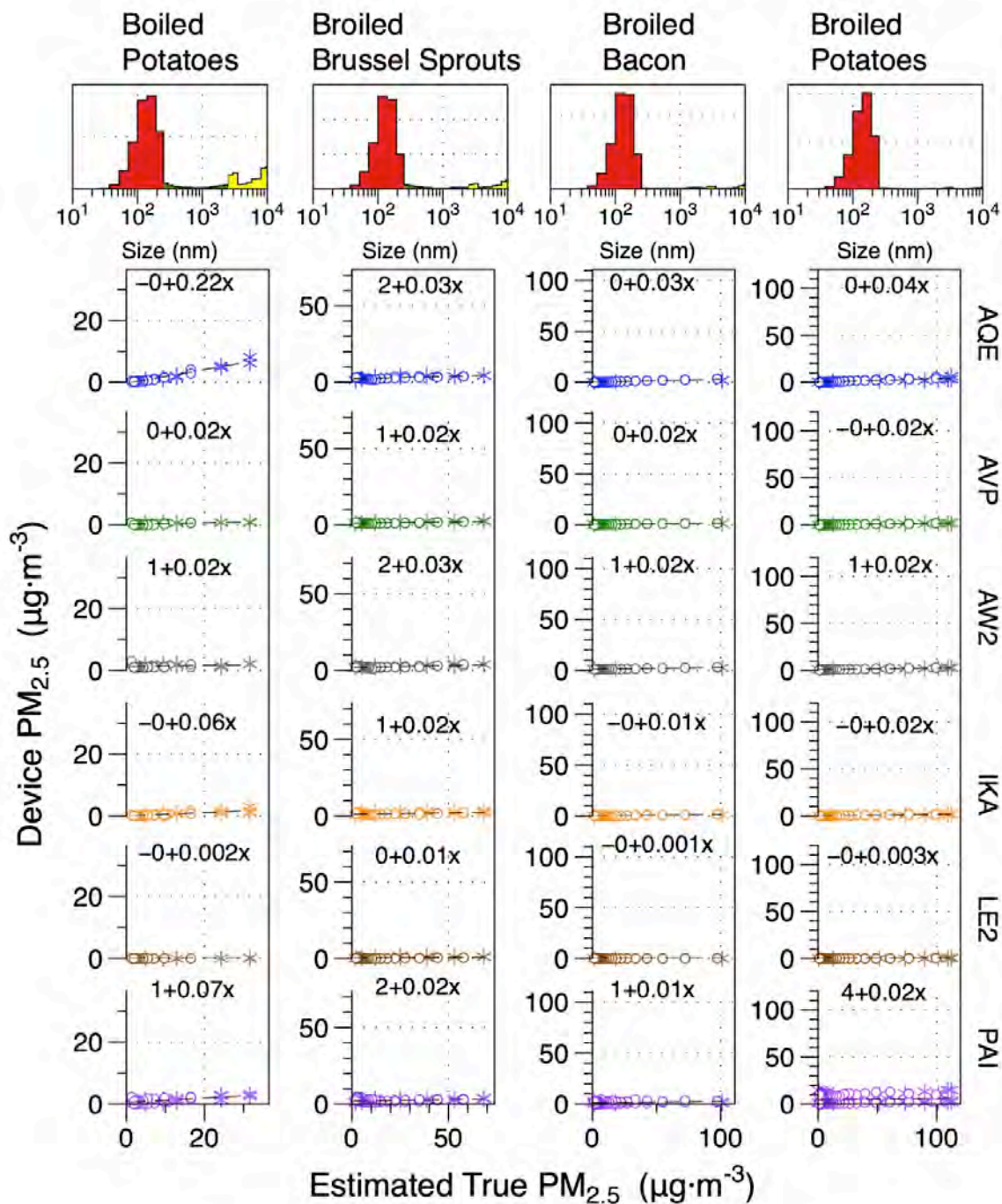
1 2 Figure 15. Correlations between 5-min average PM 2.5 reported by low-cost monitors and estimated 3 true PM 2.5 from WRAS adjusted to gravimetric data for gas cooking without frying. Histograms at 4 top show the distribution of PM mass over range of 10 nm to 10 μm. 5
