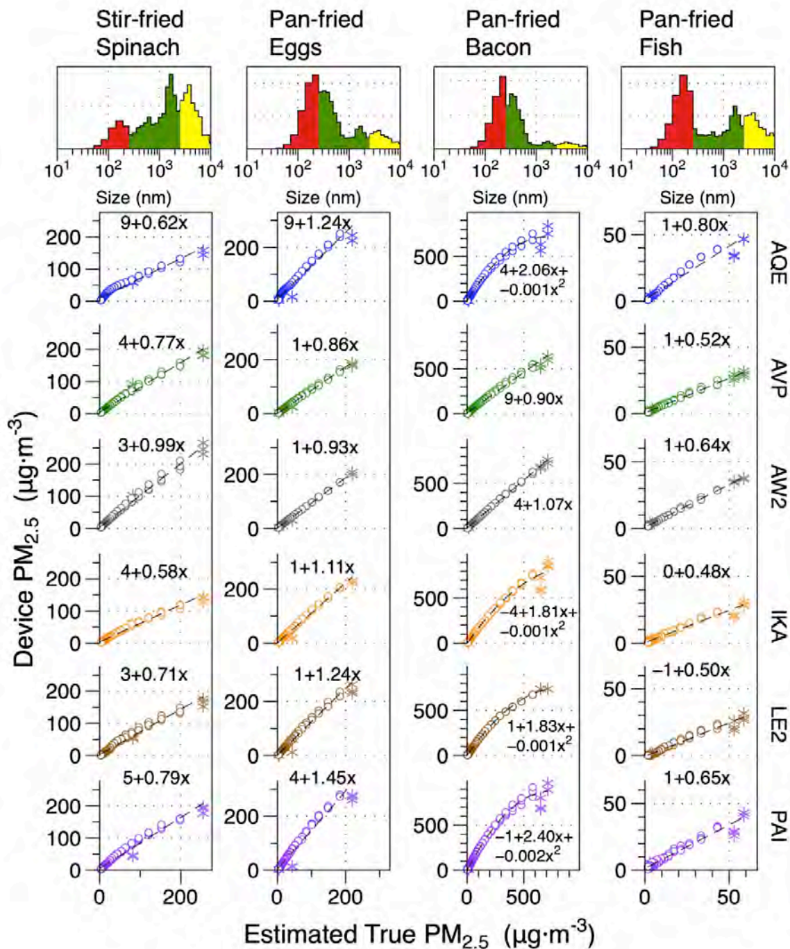
1 2 Figure 18. Correlations between 5-min average PM 2.5 reported by low-cost monitors and estimated 3 true PM 2.5 from WRAS adjusted to gravimetric data for cooking by frying and stir-frying. 4 Histograms at top show the distribution of PM mass over range of 10 nm to 10 μm.
