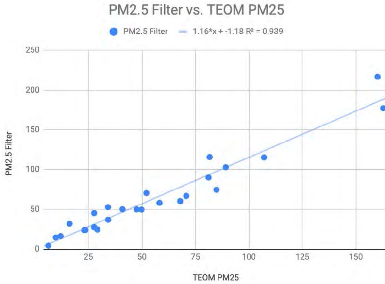
1 2 Figure S2. Correlation of PM2.5 measured with gravimetric samples to time-correlated measurements with 3 the TEOM-FDMS.
