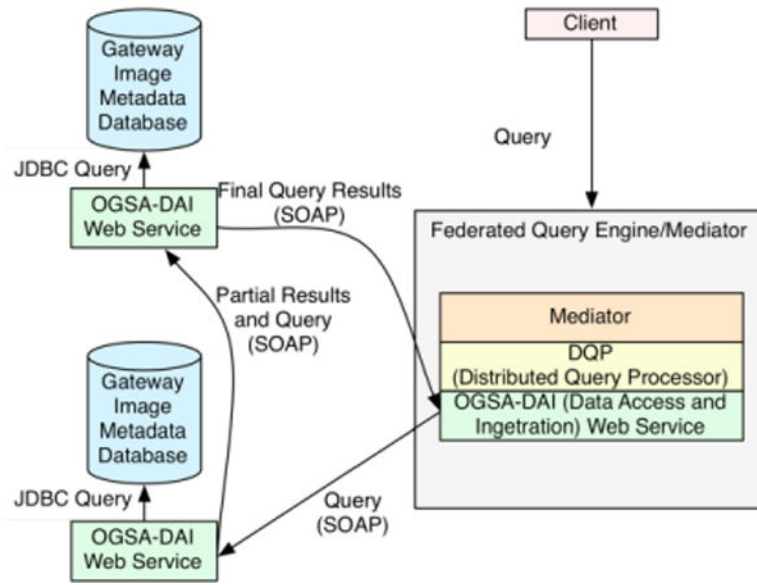
Figure 4. Implementation of Federated Query Engine/Mediator
