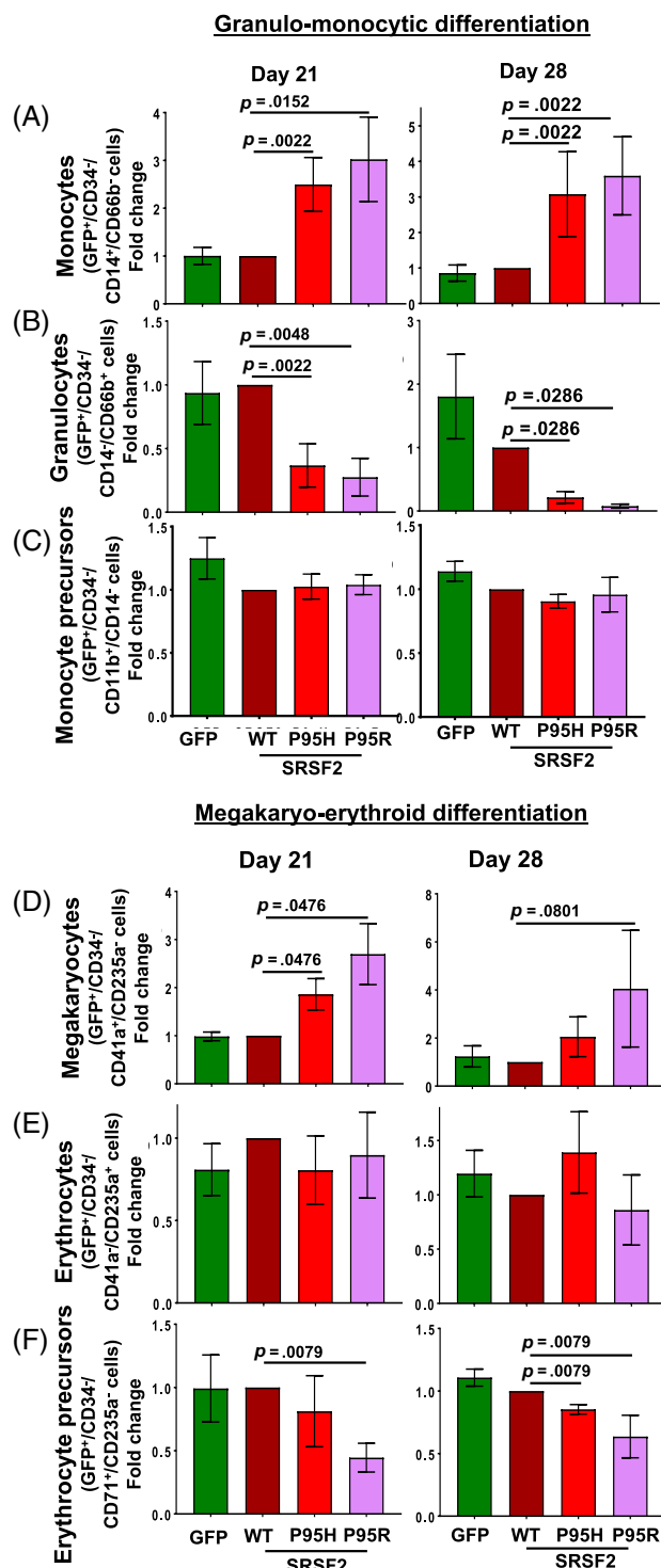
Figure 3. Mutations of SRSF2 skew myeloid differentiation. Immunophenotypic detection of lineage cells expressing the WT and mutant proteins was carried out by flow cytometry for granulo-monocytic differentiation and megakaryo-erythroid differentiation. Fold change in the percentages of (A) monocytes (CD34 + /GFP + /CD14 + /CD66b − ), (B) granulocytes (CD34 + /GFP + /CD14 − /CD66b + ), (C) monocyte precursors (CD34 + /GFP + /CD11b + /CD14 − ), (D) megakaryocytes (CD34 + /GFP + /CD41a + /CD235a − ), (E) erythrocytes (CD34 + /GFP + /CD41a − /CD235a + ), and (F) erythroid precursors (CD34 + /GFP + /CD71 + /CD235a − ) were calculated relative to the wildtype for days 21 and 28. Percentages of positive populations are shown in Supporting Information Figure S6B, S6C, respectively. All data are represented as mean \pm standard error of four independent experiments. The p values were calculated using the Mann–Whitney test in GraphPad Prism v7. The p values \leq 0.05 were considered significant and are shown. Abbreviation: WT, wildtype.
