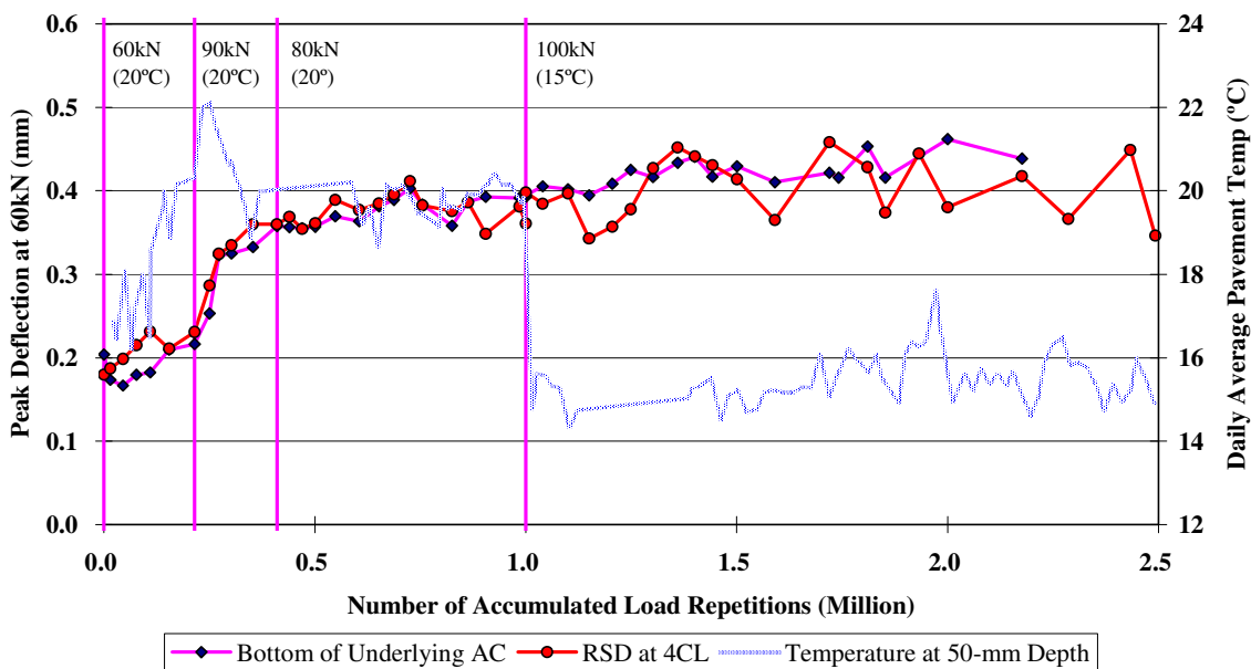
Figure 3.17: Elastic deflections at MDD4 with 60 kN test load.
