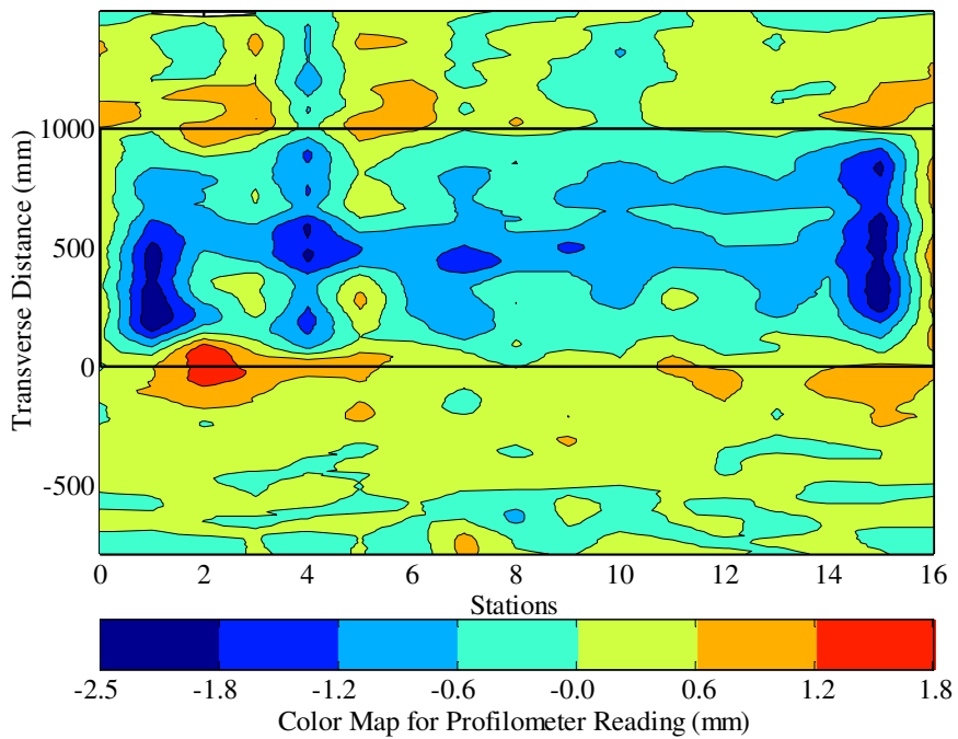
Figure 3.24: Contour plot of permanent deformation after 215,000 repetitions.
