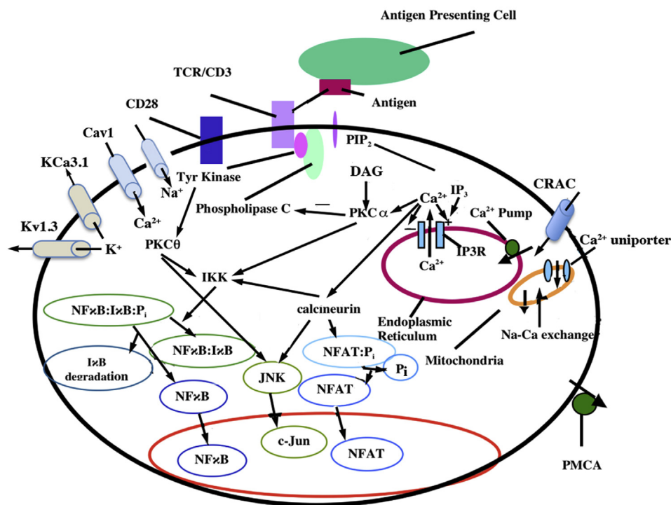
Figure 1. Schematic diagram for T cell activation and mechanism of \text{IP}_3 activation. (A) Schematic diagram of the mechanism of \text{Ca}^{2+} dynamics in T-cells. (B) \text{IP}_3 activation pathway. (C) The model of \text{IP}_3 /channel subunit [78]. Each subunit represents an \text{IP}_3 binding site, activating and inactivating \text{Ca}^{2+} binding site. Each state is labeled X_{ikj} , where i ( \text{IP}_3 binding site), j (activating \text{Ca}^{2+} binding site) and k (inactivating \text{Ca}^{2+} binding site) are equal to 0 (unoccupied binding site) or 1 (occupied binding site) [78].
