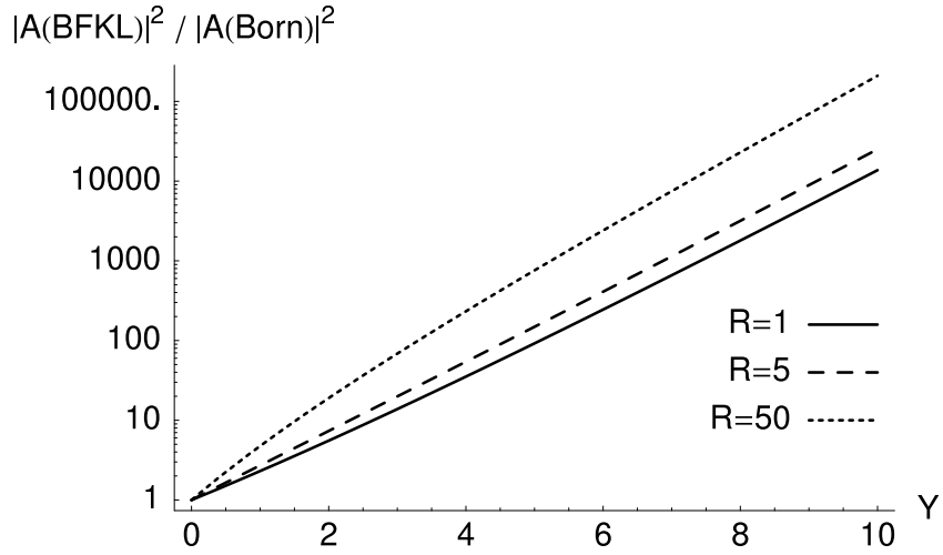
Figure 3: Ratio of the leading order BFKL cross section \left. \frac{d\sigma}{dt} \right|_{t_{min}} to the Born level cross section as a function of the rapidity Y , using \bar{\alpha}_s = 0.2 . The solid curve is for R = Q_1/Q_2 = 1 , the dashed curve is for R = 5 , and the dotted curve is for R = 50 .
