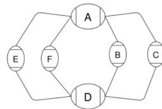
Fig. 4. A cyclic chain containing two snarls, (\bar{a}, \bar{d}) and (d, a)
