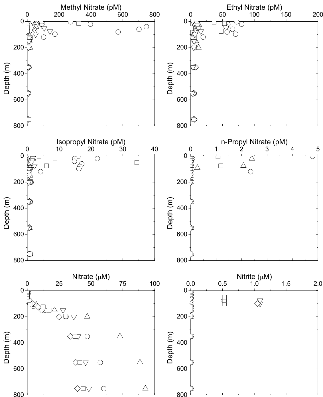
Figure 4. Depth profiles for casts taken in the Equatorial waters (0–2.5°N). Note the change in the x axes relative to the Warm Pool waters. Cast 9 (open circles), Cast 10 (open right-side up triangles), Cast 11 (open diamonds), Cast 12 (open squares), Cast 16 (open upside-down triangles), Cast 17 (open sideways triangles).
