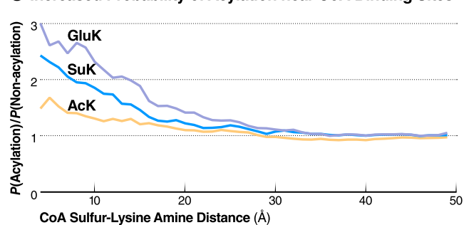
Figure 3. Structural modeling of CoA conformation reveals proximal hyperacylation near CoA-binding sites (a) Schematic diagram of the computational approach used to calculate the minimal distance between a lysine residue the CoA's thiol group in a protein CoA-binding pocket. A conformational ensemble of physically plausible CoA conformation was made by combining experimentally observed bond rotational angles from CoA crystal structures after the phospho-ADP moiety. Full structural models of CoA-binding proteins from acylomic datasets were generated using Swissmodel. The CoA ensemble was docked into each protein model to generate a set of sterically accessible CoA thiol locations and used to score each modeled lysine residue's amine-thiol distance. (b) Table showing the numbers of non-acylated and acylated lysine residues found on CoA-binding proteins. Relative odds ratio for CoA-reachable lysines (< 5 Å from the nearest CoA ensemble sulfur) being acylated vs. more distal lysine residues were calculated for each of acetylation, succinylation, and glutarylation. The significance of the results was calculated using Fisher's exact test. (c) Relative probability of lysine acylation on CoA binding protein lysines as a function of a lysine's distance from the CoA ensemble. Data shown for acetylation, succinylation, and glutarylation.
