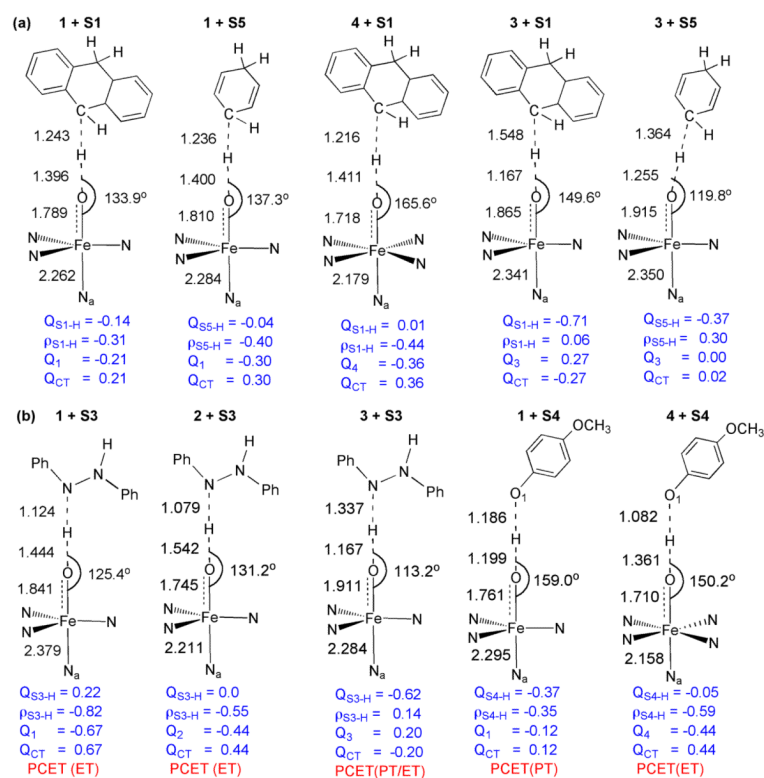
Figure 6. Schematic representations of bond activation TSs along with NBO charges ( Q ) and spin densities ( \rho ) on the H-abstracted moiety ( S-H ), the charge on the oxidant ( Q_{1-4} ), and the amount of charge transferred ( Q_{CT} ) from the substrate to the oxidant or vice versa in the cases of (a) C-H activation ( S1 and S5 ) and (b) N-H/O-H activation ( S3 and S4 ).
