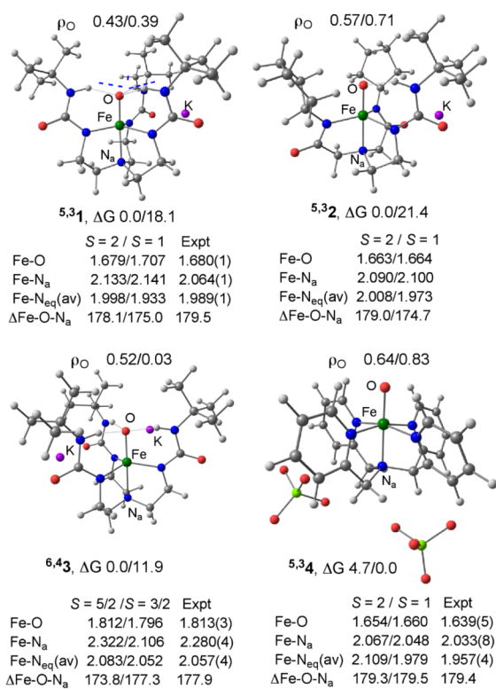
Figure 2. Computed and experimental (Expt) 17a,b,d;29 geometric parameters (bond length in Å and angle in °) and relative free energies including solvation correction ( \Delta G in kcal/mol) of the lowest spin states for 1–4 . The pink spheres in 1–3 represent the \text{K}^+ ions. \rho_{\text{O}} is the spin density on the oxo ligand in S = 2;1 for 1, 2, 4 and in S = 5/2;3/2 for 3 .
