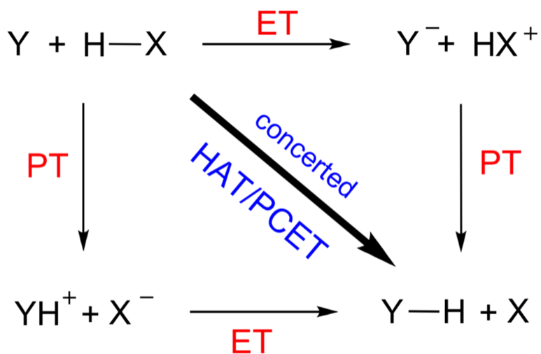
Scheme 4. The mechanistic spectrum of HAT and PCET.
