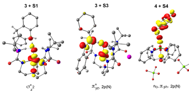
Figure 9. SNOs in TSs: \phi_{PT} type SNOs for 3+S1 , 3+S3 , vs. the typical \phi_{HAT} type in 4+S4 . The hydrogen atoms not in O---H---X moiety are omitted for clarity.
