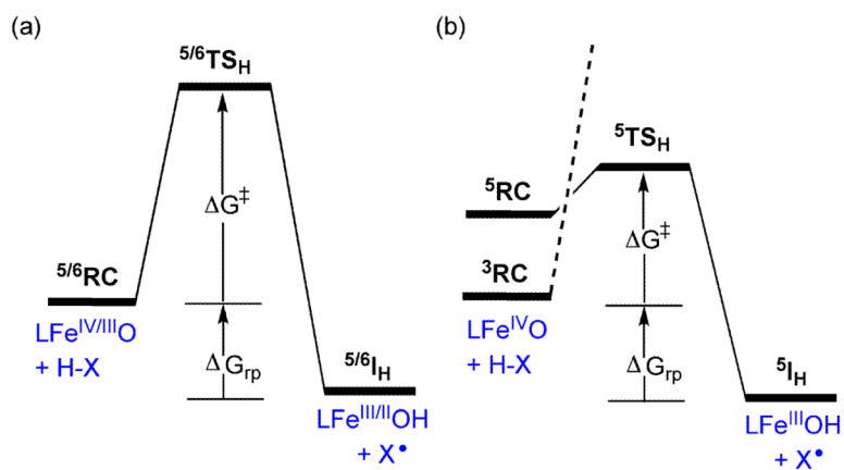
Figure 3. Generic energy profiles, starting from the reactant complex ( RC ). \Delta G^\ddagger is the free energy barrier and \Delta G_{rp} is the thermodynamic driving force of the reaction. (a) \text{LFe}^{\text{IV/III}}\text{O} (of 1–3 in their ground spin states) + \text{H-X} to the intermediates \text{LFe}^{\text{III/II}}\text{OH} + \text{X}^\bullet . (b) \text{LFe}^{\text{IV}}\text{O} of 4 , which involves TSR (the dashed line signifies that the S=1 process correlates to a high energy {}^3\text{TS}_\text{H} species 24,28 )
