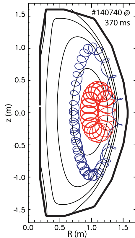
Figure 12. Orbits of 90 keV ions with pitch of v_{\perp}/v_{\parallel} = 0.40 and 0.71 in a typical equilibrium.
