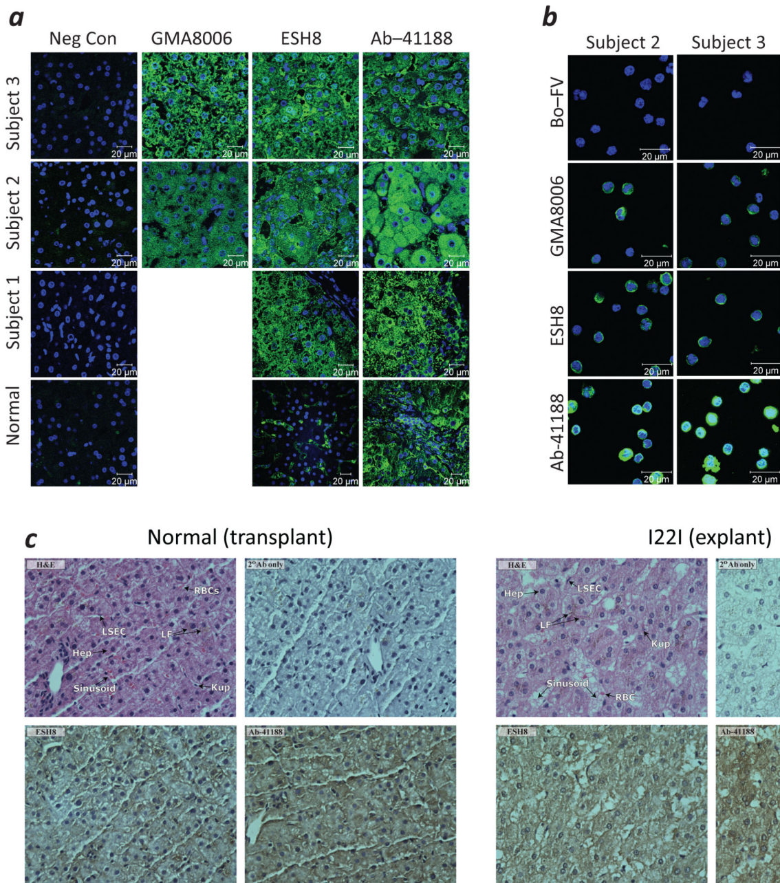
Figure 3. FVIII expression in liver tissue obtained from individuals with HA ( a ) Confocal images of histologic sections obtained from the explanted liver of the individual with the I22I whose cells were used to generate the Inv cells (Sample 1), biopsies of his transplanted liver (Normal), and explanted livers from two additional subjects with the I22I (Subjects 2 & 3) immunostained with the indicated mAbs. The areas stained by the Abs specific to FVIII are depicted in green and the DAPI stained nuclei in blue. ( b ) Confocal images of PBMCs which were frozen at the time of transplant for Subjects 2 and 3 (Fig. 3a) stained with the indicated mAbs. Areas stained by the Abs specific to FVIII are depicted in green and the DAPI stained nuclei in blue. ( c ) Immunohistochemistry stained sections from a biopsy of the
