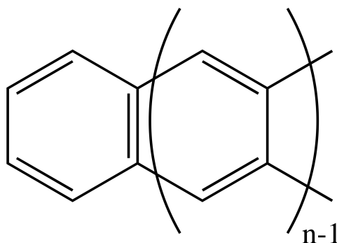
Figure 3: The chemical structure of n -acene ( C_{2n}H_{4n}C_{4n}H_{2n} ).
