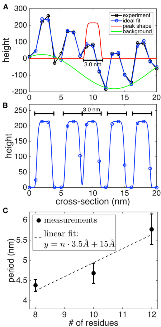
FIGURE 3 Agreement between predicted and observed \beta -tape periodicity. (A) A representative line cross-section profile observed in AFM (black) is fit to a sum of five peaks (modeled as generalized error distributions, red) on top of a varying height background (modeled as a sinusoid, green); final fit curve is shown (blue). The best-fitting peak shape (shape parameter of \sim 7.0 ) indicates a flat-topped distribution, such that gaps between adjacent peaks are expected. This is seen in (B), where the background is subtracted from the best-fit curve. (Black bars) Predicted \beta -tape width, 3.0 nm. (C) Error-weighted linear regression of AFM-derived row periodicity as a function of peptide length. To see this figure in color, go online.
