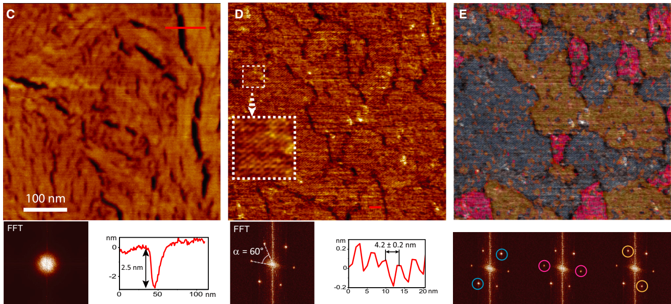
FIGURE 2 Designed peptide assemblies with long-range order. (A) Assembly protocol to obtain dry peptide assemblies on graphene/graphite. (B) Sequences of the peptides tested in this article. (C) AFM image of peptide 2 in air. FFT image and line cross section through an area that contains a void are also shown below the image. (D) AFM image of the same sample while the sample has been immersed in water for ~20 min (same scale as in C), as well as FFT and line cross section. A 2 \times magnified view of an area ( dashed square ) reveals a periodic structure that consists of rows with a spacing of 4.0–4.5 nm, and the FFT reveals ordering in six directions with C 6 symmetry. (E) Selected peak-pair inverse-FFT mapping of the peptide domains. Each color represents the inverse-FFT of each set of diametrically opposite peaks (see colored circles below the image). To see this figure in color, go online.
