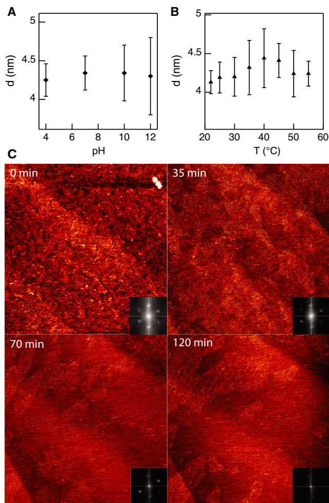
FIGURE 5 Stability to extreme buffer conditions. (A) Spacing ( d ) of peptide layer 2 (obtained from FFT of images) under >30 -min incubation in solutions of different pH values. (B) Similar to (A), except that temperature was the changing parameter (obtained at pH 7). (C) Representative AFM images of peptide 2 taken from a time-series under incubation in 8 M urea at indicated times. (Insets) FFTs of the respective images. To see this figure in color, go online.
