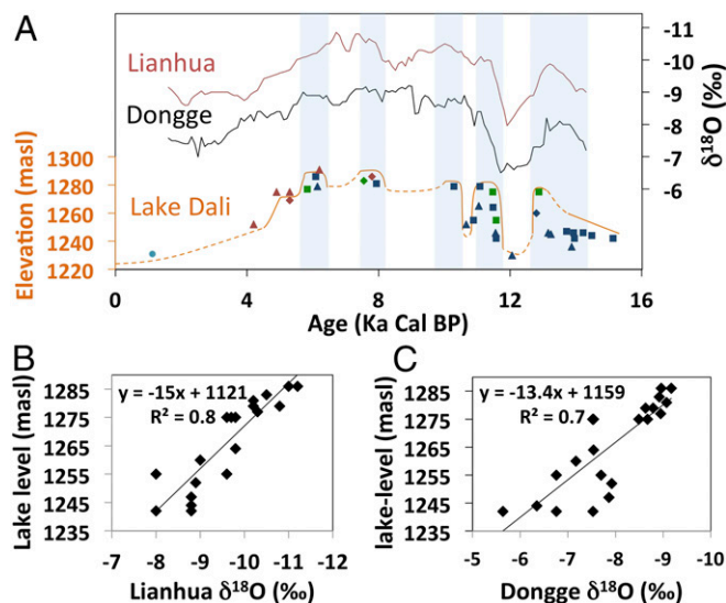
Fig. 3. Lake Dali lake level vs. cave \delta^{18}O_c . (A) Smoothed \delta^{18}O_c Lianhua (red curve, 5-point average) and Dongge (black, 10-point average), and Lake Dali lake level (orange). (B) Correlation between Lianhua \delta^{18}O_c and Lake Dali lake level. (C) Correlation between Dongge \delta^{18}O_c and Lake Dali lake level. Light-blue bars represent highstands of the lake.
