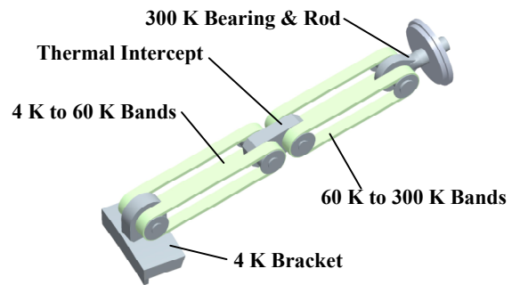
Figure 4: A Coupling Magnet Cold Mass Support.
