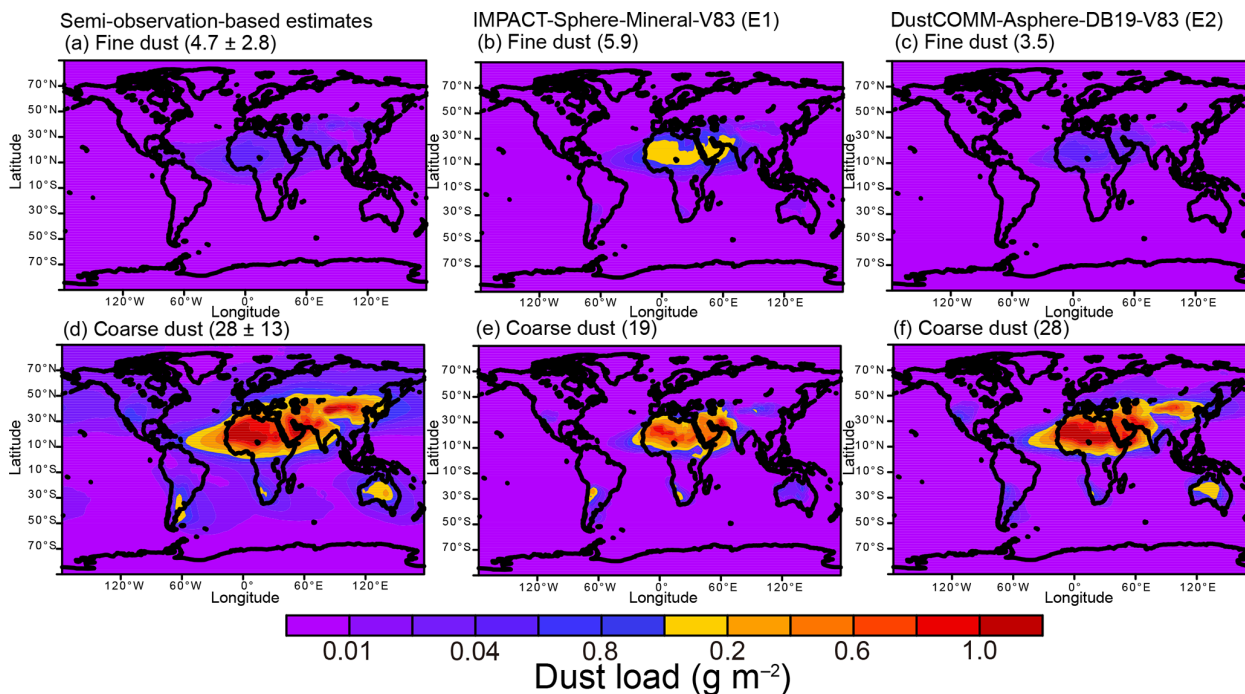
Figure 3. Model-simulated dust loads at fine (smaller than 2.5 \mu\text{m} in diameter) and coarse size ranges (larger than 2.5 \mu\text{m} in diameter) before and after adjusting the size-resolved dust load with DustCOMM. Results are shown for (a) fine dust from DustCOMM, (b) fine dust from IMPACT-Sphere-Mineral-V83 (E1), (c) fine dust from DustCOMM-Asphere-DB19-V83 (E2), (d) coarse dust from DustCOMM, (e) coarse dust from E1, and (f) coarse dust from E2 simulations. The parentheses represent the global dust burden ( T_g ). The values of dust load at each bin are listed in Table 3.
