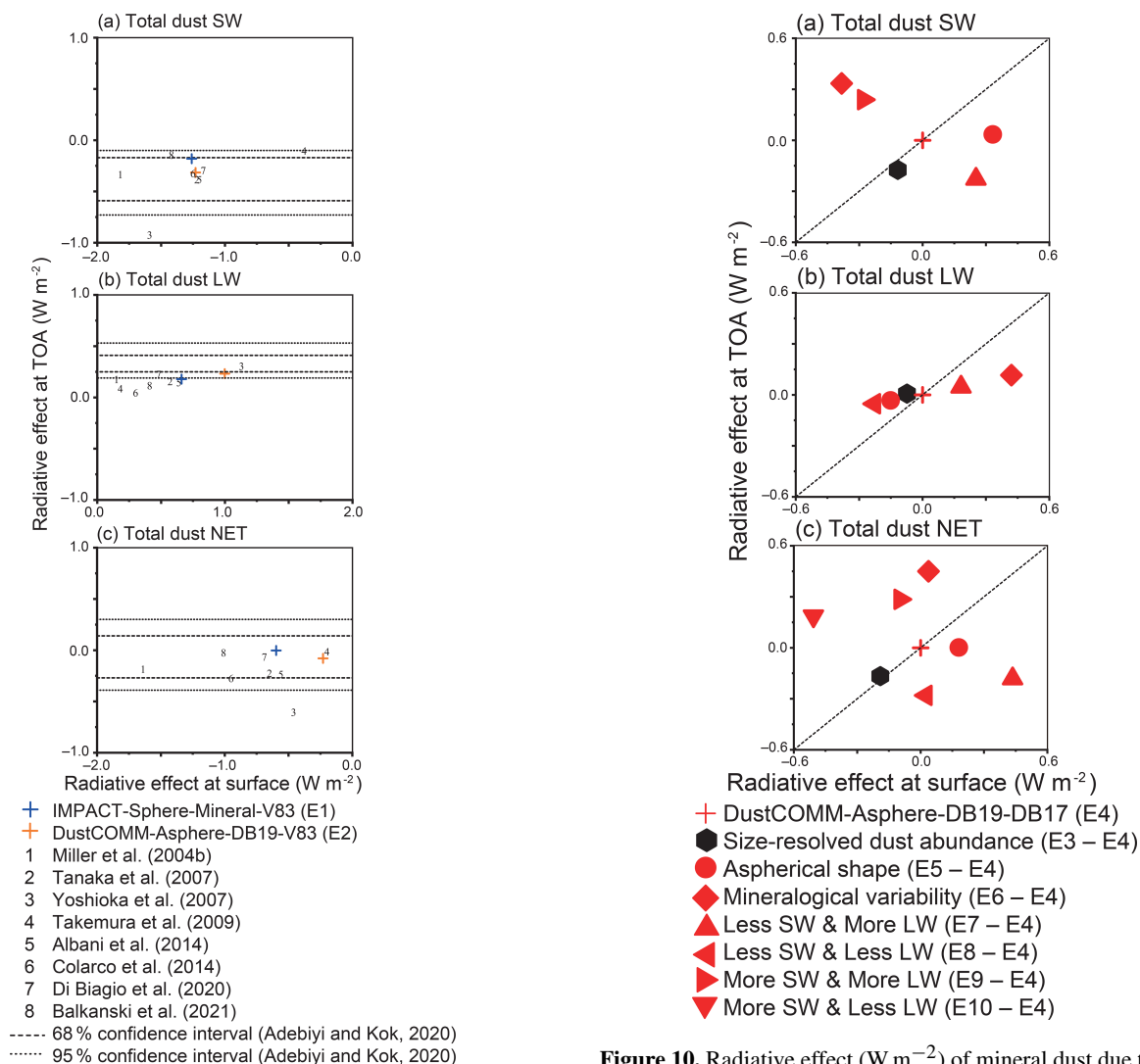
Figure 9. Variability of dust radiative effect ( \text{W m}^{-2} ) in different model simulations at the surface and TOA for (a) total dust SW, (b) total dust LW, and (c) total dust NET. The annually averaged values are listed in Table 5.
