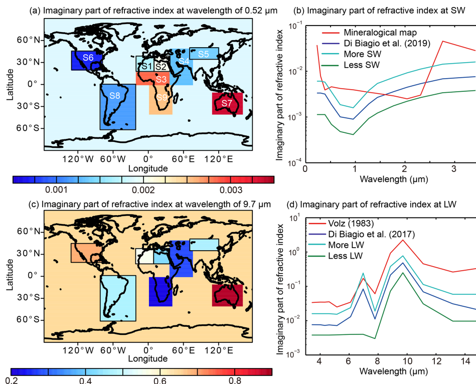
Figure 1. Imaginary part of the refractive index at (a) 0.52 \mu\text{m} , (b) SW, (c) 9.7 \mu\text{m} , and (d) LW. The refractive index obtained from 19 samples was aggregated into nine main source regions, and the arithmetic mean was calculated for each source region (Di Biagio et al., 2017, 2019). The global mean is used for others. The coordinates of the nine source regions were (S1) western North Africa (18–37.5° N, 20° W–7.5° E), (S2) eastern North Africa (18–37.5° N, 7.5–35° E), (S3) the Sahel (0–18° N, 20° W–35° E), (S4) Middle East/Central Asia (0–35° N, 30–70° E and 35–50° N, 30–75° E), (S5) East Asia (35–50° N, 70–120° E), (S6) North America (20–45° N, 130–80° W), (S7) Australia (10–40° S, 110–160° E), (S8) South America (0–60° S, 80–20° W), and (S9) southern Africa (0–40° S, 0–40° E).
