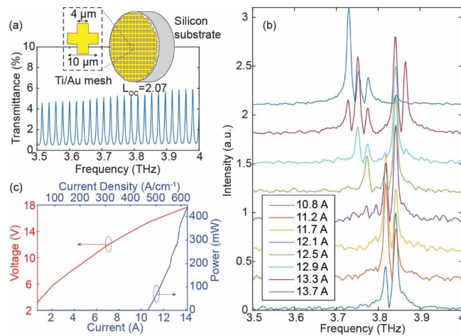
Figure 4. (a) Analytical transmittance of the silicon output coupler with a thickness of 2.07 mm. Inset shows the inductive mesh designed with a period of 10 μm and width of 4 μm. (b) Normalized lasing spectra at the cavity length supporting multiple lasing modes measured under different biases (offset for clarity). (c) Corresponding pulsed L - I - V curves measured at 77 K.
