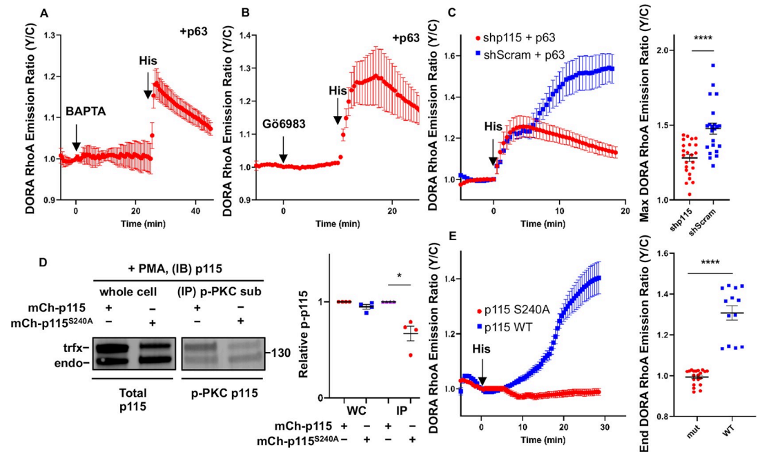
Fig 2. Second phase of RhoA activation is dependent on the \text{Ca}^{2+} /PKC/p115 signaling axis. (A–B) Representative average time courses \pm SEM of the Y/C emission ratio changes in HeLa cells coexpressing p63 and DORA RhoA. Cells were stimulated with either 20 \mu\text{M} BAPTA (A) ( n = 4 cells) or stimulated with 1 \mu\text{M} Gö6983 (B) ( n = 7 cells). Then cells were subsequently stimulated with 100 \mu\text{M} histamine. (C) Left: Representative average time courses \pm SEM of the Y/C emission ratio changes in HeLa cells expressing DORA RhoA, p63, and either shRNA p115 (red) or shRNA Scrambled (blue) and stimulated with 100 \mu\text{M} histamine (shp115: n = 5 cells; shScrambled: n = 4 cells). Right: Maximum emission ratio changes upon histamine stimulation (shp115: n = 23 cells; shScrambled: n = 22 cells). **** P < 0.0001 ; unpaired two-tailed Student's t test. (D) Left: Representative western blot images of HeLa cells show that PKC phosphorylates p115 on the serine 240 residue. HeLa cells expressing either mCherry-tagged p115 or p115 S240A were stimulated with 50 ng/mL PMA and subjected to immunoprecipitation with antibodies to phospho-PKC substrate. Whole-cell samples and the IP samples were immunoblotted for p115. Right: Densitometry analysis of the adjacent immunoblot is calculating the percentage of PKC-phosphorylated p115 over total p115 for the endogenous p115 ("endo," lower band) and transfected p115 ("trfx," upper band). Average percentage \pm SEM shown in bar graph among the various transfection conditions ( n = 4 for each condition). Endogenous p115 versus p115 S240A: P = 0.1 ; Transfected p115 versus p115 S240A: * P = 0.02 ; unpaired two-tailed Student's t test. (E) Representative average time courses \pm SEM of the Y/C emission ratio changes in DORA RhoA-expressing HeLa cells coexpressing either mCherry-tagged p115 (blue) or mCherry-tagged p115 S240A (red) and stimulated with 100 \mu\text{M} histamine (p115: n = 5 cells; p115 S240A: n = 12 cells). Right: Maximum emission ratio changes upon histamine stimulation (p115: n = 13 cells; p115 S240A: n = 20 cells). **** P < 0.0001 ; unpaired two-tailed Student's t test. The underlying data for this figure can be found in S1 Data . BAPTA, 1,2-Bis(2-aminophenoxy)ethane- \text{N,N,N',N'} -tetraacetic acid tetrakis (acetoxymethyl ester); Gö6983, 3-[1-[3-(Dimethylamino)propyl]-5-methoxy-1H-indol-3-yl]-4-(1H-indol-3-yl)-1H-pyrrole-2,5-dione; IB, immunoblotting; IP, immunoprecipitated; PMA, phorbol myristate acetate; WC, whole cell lysate; WT, wild type; Y/C, yellow/cyan.
