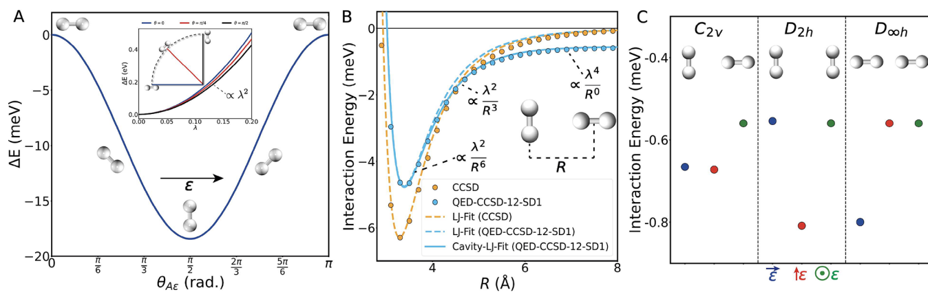
Figure 3. (A) Energy difference, \Delta E , between a single \text{H}_2 molecule inside a cavity aligned perfectly along the cavity polarization vector, \epsilon , and different angles relative to the cavity polarization vector. The inset shows that the energy of a single molecule within a cavity increases with \lambda^2 . (B) Intermolecular interaction energies, E_{AB} , and fits to a Lennard-Jones type potential given by eq 3 (dashed lines) and cavity-modified Lennard-Jones type potential given by eq 4 (solid line). (C) Intermolecular interaction energies, E_{AB} , at 25 Å for various high-symmetry molecular orientations and cavity polarizations. All calculations shown in this figure were performed using QED-CCSD-12-SD1 with \lambda = 0.1 au.
