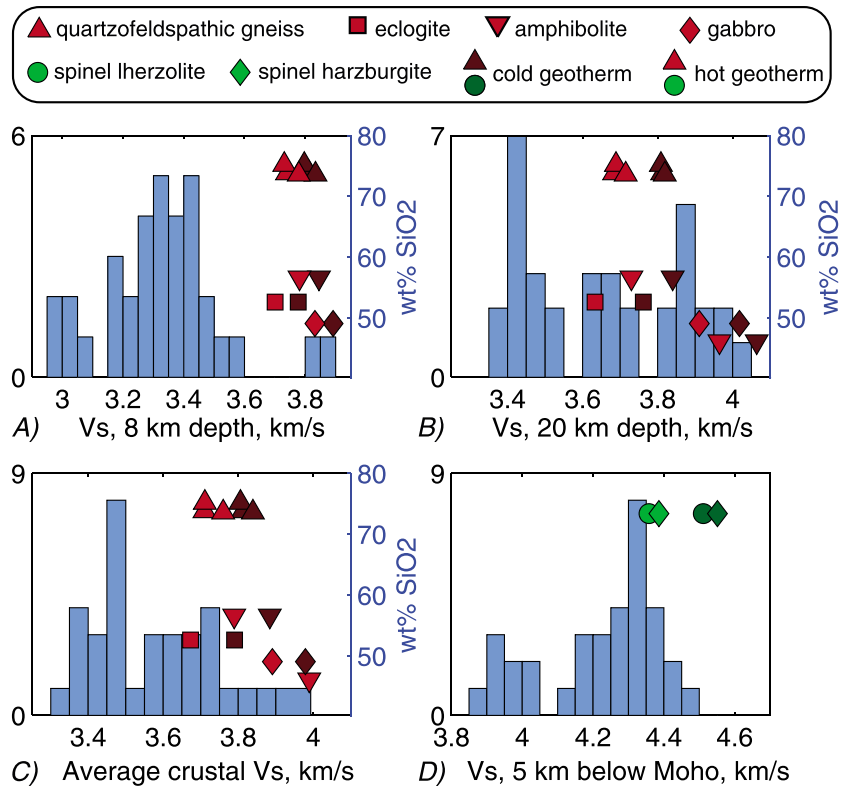
Figure 8. Histograms of V_S for all depth ranges and stations shown in Figure 6. Symbols show V_S predictions from different lithologies, plotted against wt % \text{SiO}_2 . (a–c) Histograms of V_S at crustal depths (left axis) compared with predictions for crustal lithologies (symbols; right axis) from Brownlee et al. [2011] or Brooks and Tegner [2001] as described in text. (d) Uppermost mantle V_S and predictions for ultramafic rocks (symbols); compositions from Hacker et al. [2003]. Compositions are described in legend (top). Velocities are calculated [ Hacker and Abers , 2004; Abers and Hacker , 2016] at the depths of 8 km in Figure 8a, 20 km in Figure 8b, average between Moho and base of layers with V_S < 2.5 km/s in Figure 8c, and 40 km in Figure 8d. Two geotherms are assumed, a cold one with surface flux of 50 \text{ mW/m}^2 (dark symbols) and a hot one with 150 \text{ mW/m}^2 (bright symbols); see Figure 9. Calculations are for solid parts of rock only; small melt fractions could lower V_S substantially, depending on melt topology.
