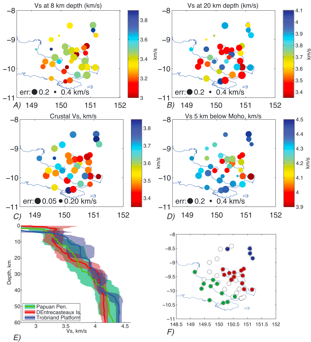
Figure 6. V_S at different depths. (a) Upper crust at 8 km depth. (b) Lower crust at 20 km depth. (c) Mean crustal V_S above Moho, averaged as 1/V_S to preserve travel times. Only depths where V_S > 2.5 km/s are included in averages to remove effects of near-surface sediment. (d) V_S 5 km below Moho. For Figures 6a–6d, symbol size scales inversely to formal error as shown; error represents 80% probability range. (e) V_S versus depth averaged over groups of stations, as indicated by key. Solid shading indicates 1\sigma variation in V_S between stations in the same group. (f) Stations used in groupings for Figure 6e as indicated by color; open circles indicate stations not used.
