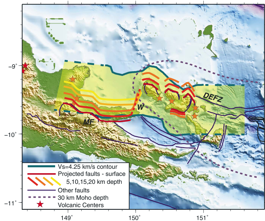
Figure 10. Comparison of low-velocity upper mantle anomaly [Jin et al. , 2015] to downward projection of surface faults. Yellow field bounded by teal line represents V_S \leq 4.25 km/s at 50 km depth. Purple dashed line shows 30 km Moho depth contour. Red, orange, and yellow lines show major faults projected downward as indicated by seismicity or focal mechanisms, at dips of 30^\circ for north dipping faults and 60^\circ for south dipping faults that are seismically active; geometry of Ward Hunt Strait transfer zone (W) is guessed from seismicity and focal mechanism (Figure 3a). Following the maximum depths of earthquakes, the Mai'iu Fault is extrapolated to 20 km depth and faults bounding the Goodenough-Fergusson MCCs are extrapolated to 10 km depth. Thick black line east of 151.7^\circ\text{E} shows oceanic spreading center, and surrounding black line denotes new ocean crust. Other symbols and abbreviations are same as Figure 2.
