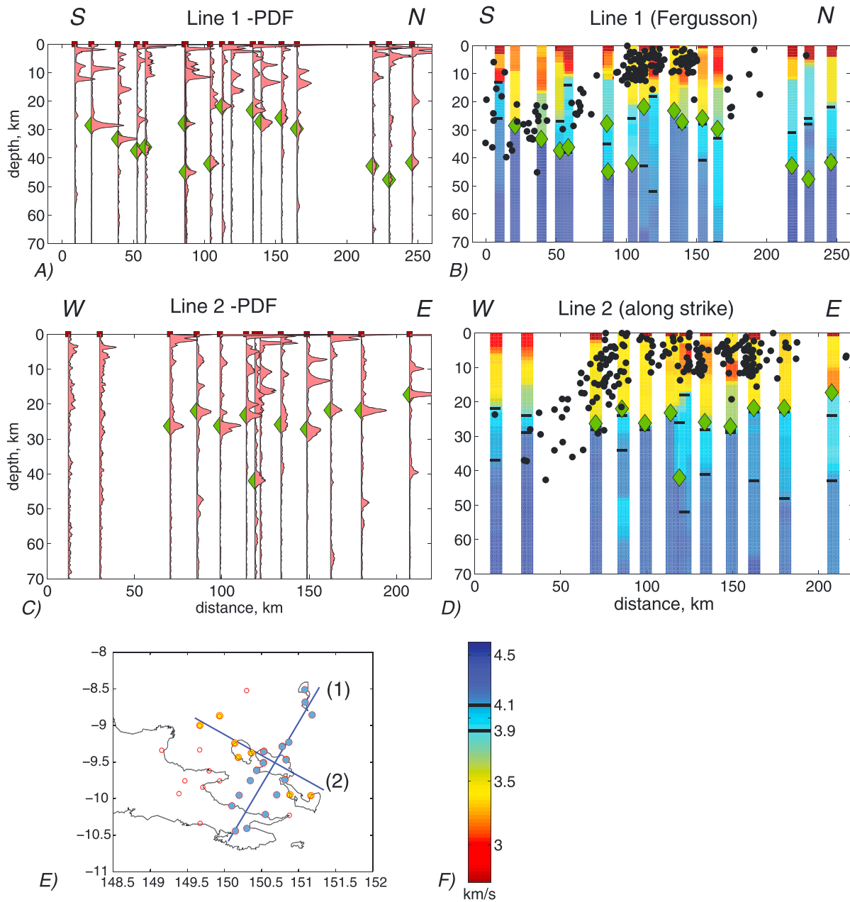
Figure 7. Cross sections of joint inversion results. (a and b) Cross section (1) through Fergusson Island. (c and d) Cross section (2) through Dayman Dome and Kiribisi Basin. (e) Locations of cross sections, stations colored if used in cross sections (1). (f) Color scale for velocities shown in Figures 7b and 7d. Figures 7a and 7c are pdfs for interface depth beneath each station. Figures 7b and 7d show V_S columns beneath each station, with horizontal bars corresponding to V_S = 3.9 and 4.1 km/s and seismicity within 35 km of the section as black dots. Green diamonds on Figures 7a–7d indicate maximum-likelihood interface depth identified as Moho, in cases where dV_M > 0.25 km/s (velocity contrast \pm 5 km from interface).
