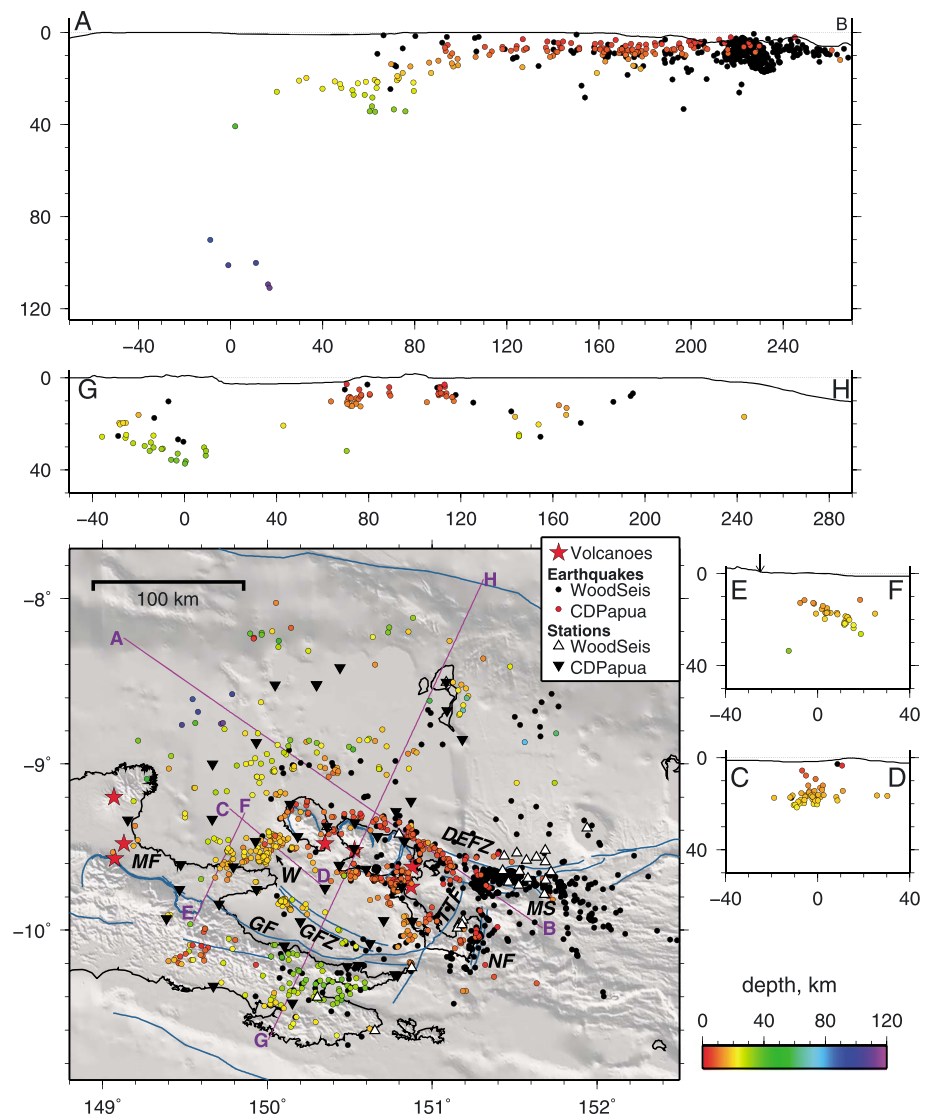
Figure 2. Microseismicity determined from regional arrays, from CDPAPUA (colored dots) and WOODSEIS (black dots). All relocations redetermined by HypoDD [Waldhauser and Ellsworth, 2000] as described in text. For the CDPAPUA hypocenters, depths are color coded as per lower right scale bar. Abbreviations are MF: Mai'iu Fault, W: Ward Hunt Strait Fault Zone, GF: Goodenough Bay Fault, GFZ: Goshen Fault Zone [Mutter et al., 1996], DEFZ: D'Entrecasteaux Island Fault Zone, TTF: Trobriand Transfer Fault [Little et al., 2011], NF: Normanby Fault [Little et al., 2007], and MS: Moresby Seamount. Cross sections are shown in other panels as labeled; topography exaggerated two times and dotted line shows sea level. Arrow on E-F indicates surface trace of Mai'iu Fault. Earthquakes are projected \pm 10 km from locations of cross sections shown on map, except for A-B where projection is \pm 25 km.
