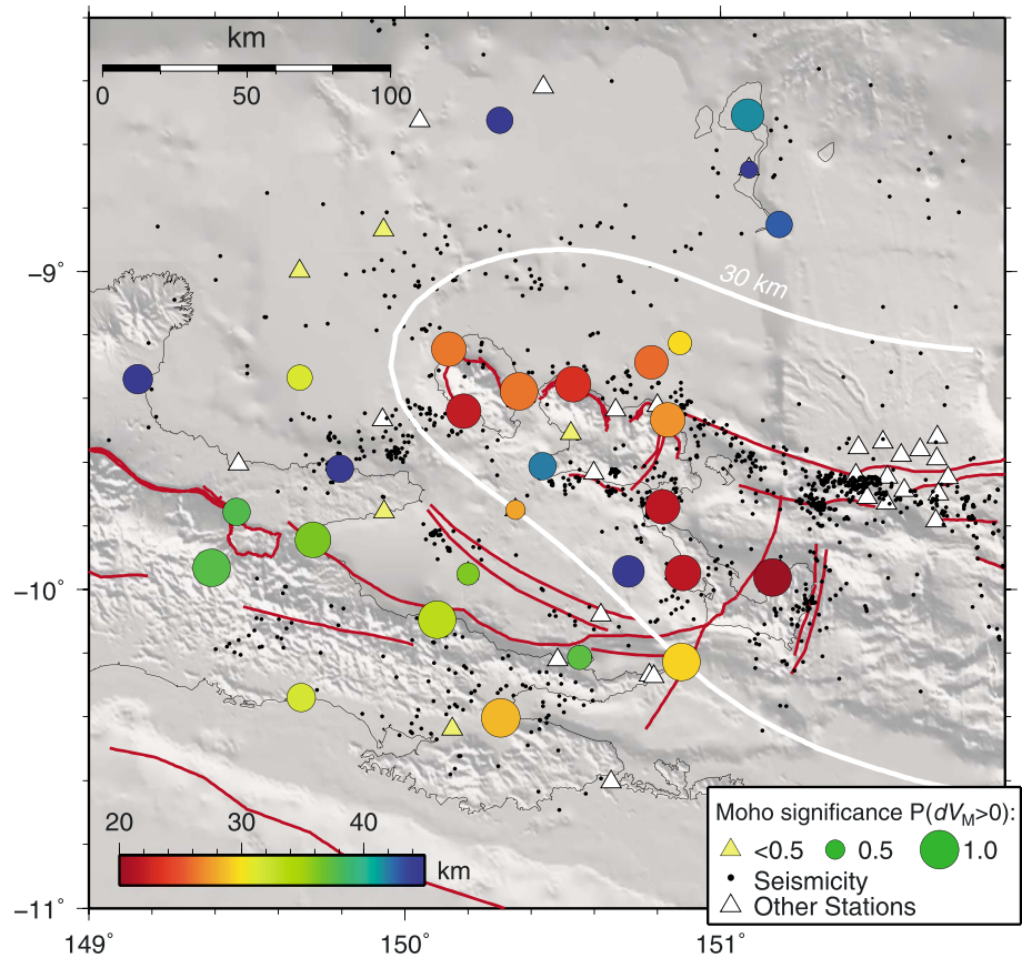
Figure 5. Crustal thickness below each station determined from joint inversions. Circles, colored by best fitting Moho depth, are scaled to P(dV_M > 0) the fraction of successful models for which the Moho velocity step dV_M is positive. Triangles show stations for which P(dV_M > 0) is less than 0.5 (yellow), or no receiver functions could be determined (open). Black dots show relocated seismicity. White line shows approximate 30 km depth contour from fitting third-order polynomial surface to these data.
