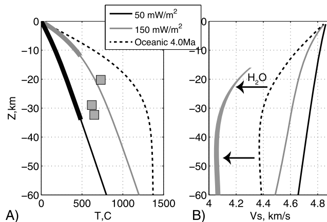
Figure 9. Geotherms and predicted mantle V_S . (a) Temperatures along a hot (gray) and cool (black) continental geotherm as described in text and a young oceanic geotherm (dashed) calculated for typical half-space cooling parameters, a 1350°C potential temperature, a plate age of 4 Ma, and 0.35 K/km adiabat [Turcotte and Schubert, 2002]. Gray squares show conditions estimated for 2–4 Ma metamorphic rocks in the D’Entrecasteaux MCCs [Hill and Baldwin, 1993]. Thick lines indicate depth range of seismogenic crust beneath the MCCs (gray) and Papuan Peninsula (black). (b) Corresponding anelastic V_S calculated along the three geotherms for dry olivine [Jackson and Faul, 2010], for typical mantle grain size of 1 cm, and at Rayleigh wave dominant periods of (3Z)/(4.2 \text{ km/s}) where Z is depth [Forsyth, 1992]. Slower gray field shows mantle V_S estimate for the 4 Ma plate geotherm including effect of typical concentrations of \text{H}_2\text{O} in olivine (50 wt ppm) and equilibrium grain sizes appropriate for strain rates of 10^{-14} to 10^{-13} \text{ s}^{-1} , at temperatures > 900^\circ\text{C} where anelastic effects are calibrated and grain size equilibrium can be assumed (calculations described in Abers et al. [2014]).
