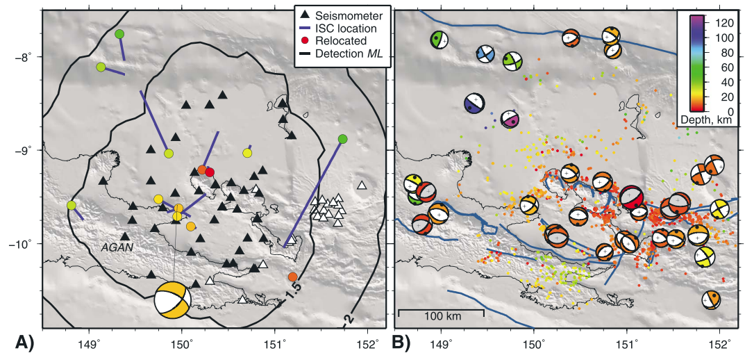
Figure 3. (a) Comparison of CDPAPUA to ISC catalog, 2010–2011. Circles show 14 earthquakes common to both catalogs at CDPAPUA epicenters, colored by relocated depth. Blue lines connect them to the corresponding ISC epicenter. Beach ball shows gCMT best double-couple solution for the one earthquake common to CDPAPUA and the gCMT catalog. Contours show detection limits for M_L = 1.5 and 2.0 . Triangles show stations, open for older WOODSEIS stations not used in detection analysis. (b) Relocated CDPAPUA seismicity and double-couple focal mechanisms from the gCMT catalog [Ekström et al. , 2012] and, for older events, from body wave inversion [Abers et al. , 1997]. The latter are indicated by gray dilatational quadrants. Compressional quadrants and epicenters are colored by depth; scale in inset.
