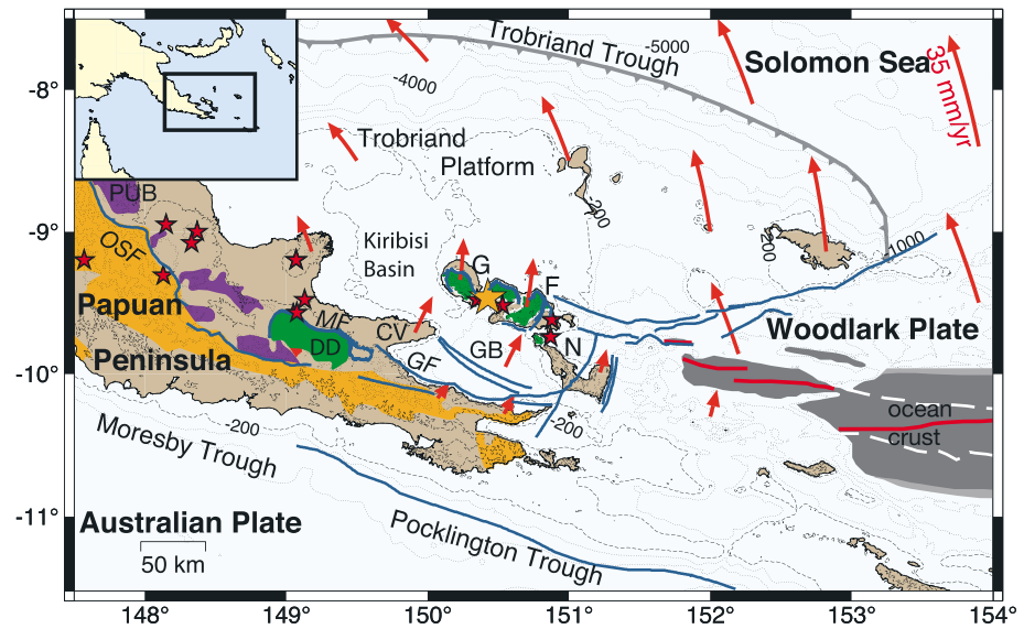
Figure 1. Main tectonic features of the Woodlark-D'Entrecasteaux Rift. Blue lines show selected active faults, and toothed gray line shows inactive Trobriand Trough. Purple field shows ultramafic rocks, orange shows Owen Stanley Metamorphics, and green shows main MCCs [e.g., Baldwin et al. , 2008; Little et al. , 2011]. Gray field shows new oceanic crust, and red line at center is spreading axis [Taylor et al. , 1999]. Red stars show Quaternary volcanic centers [Smith and Milsom, 1984]; orange star shows UHP locality [Baldwin et al. , 2008]; red arrows show GPS model velocities relative to Australia [Wallace et al. , 2014]. Labeled features include the D'Entrecasteaux Islands, G: Goodenough Island, F: Fergusson Island, and N: Normanby. Other abbreviations are PUB: southeast end of Papuan Ultramafic Belt, OSF: Owen Stanley Fault, DD: Dayman Dome, MF: Mai'iu Fault, CV: Cape Vogel, GF: Goodenough Bay Fault, and GB: Goodenough Basin. Dashed line shows 200 m water depth; dotted lines contour deeper depths at 1000 m intervals.
