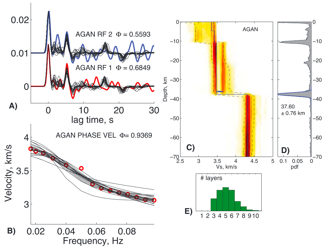
Figure 4. Example of velocity inversion for station AGAN (see Figure 3a). (a) Receiver functions for two back azimuths, 90–135° (bottom) and 315–360° (top); colored lines show stacked data, and thin black lines show best fit model predictions. (b) Phase velocities for fundamental mode Rayleigh waves. \Phi denotes misfit measure. Red circles are observed data, and black lines show best fit predictions. Figures 4a and 4b show a randomly selected 20 of the 2000 best fitting models. (c) Pdf for V_S with depth; darker colors indicate higher probability. Dashed lines bound the central 80% of acceptable models. (d) Probability density function (pdf) for interface depth; peaks show most likely depths for interfaces. The Moho is picked from the peak as described in the text, here assigned a depth of 37.60 \pm 0.76 km (1 \sigma uncertainty in local maximum probability). (e) Pdf for number of layers in the best fitting model.
