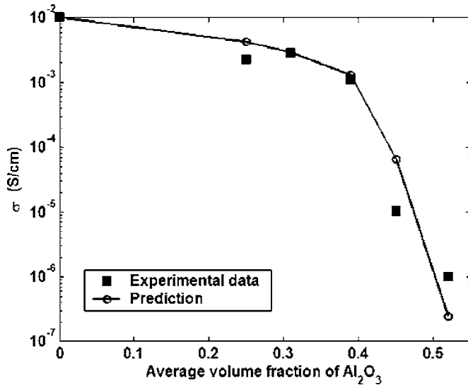
FIG. 7. Effective electric conductivity variation with average volume fraction of \text{Al}_2\text{O}_3 for the \text{Al}_2\text{O}_3/\text{Y-TZP} FGMS.
