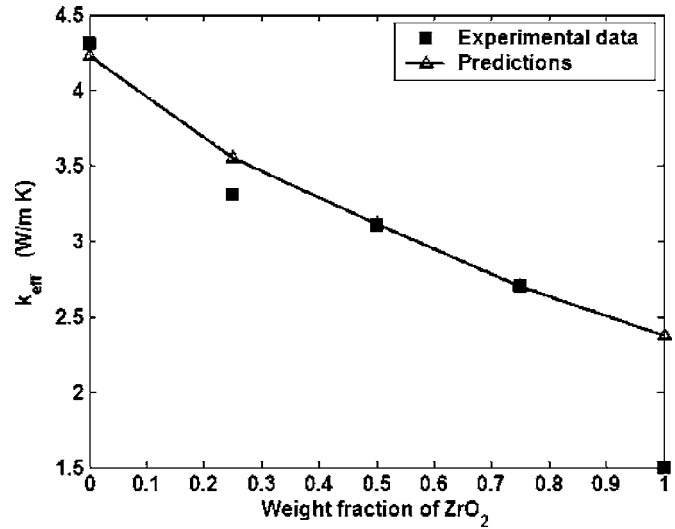
FIG. 8. Effective thermal conductivity variation with weight fraction of \text{ZrO}_2 for the \text{ZrO}_2/\text{NiCoCrAlY} FGMS.
