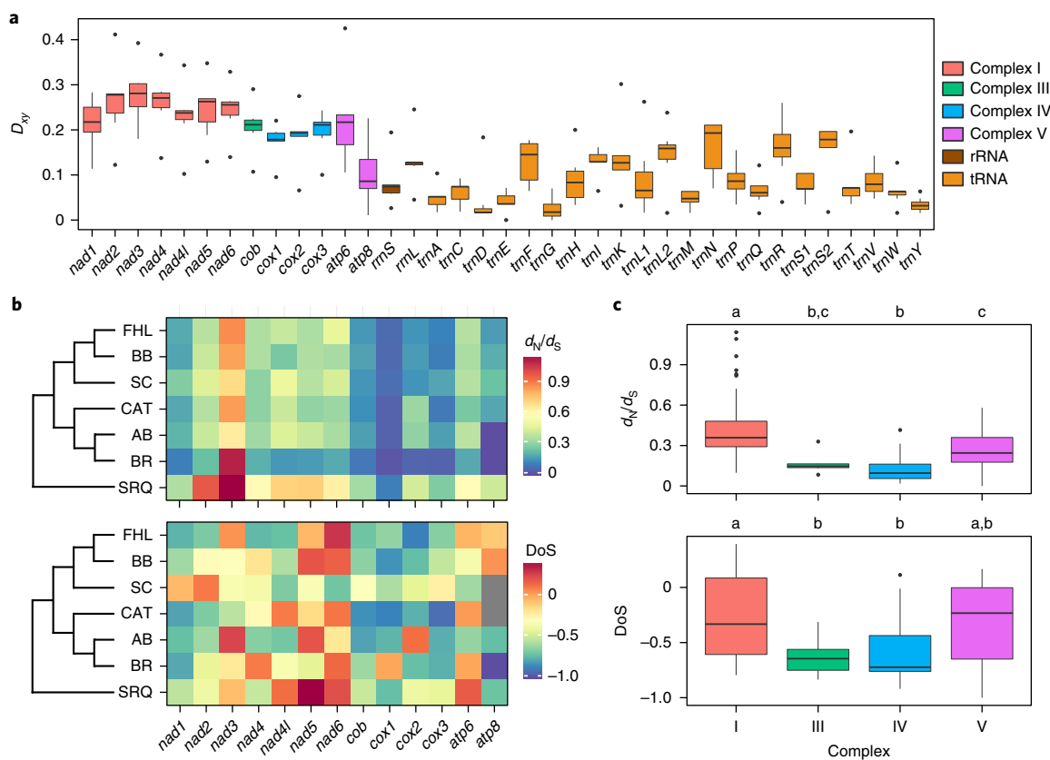
Fig. 2 | Mitochondrial divergence and evolution. a , Pairwise nucleotide divergence ( D_{xy} ) for re-sequenced populations relative to the San Diego reference across all mtDNA-encoded genes. b , Estimates of d_N/d_S (top) and DoS (bottom) relative to the San Diego reference across the 13 protein-coding genes. Missing data are represented as grey squares. AB, Abalone Cove; BB, Bodega Bay; BR, Bird Rock; CAT, Catalina Island; FHL, Friday Harbor; SC, Santa Cruz; SRQ, San Roque. c , d_N/d_S (top) and DoS (bottom) for protein subunits of the OXPHOS complexes. For each complex, values were pooled across the seven interpopulation alignments. Superscript, lower-case letters above the bars denote the results of Mann-Whitney U -tests, followed by correction for multiple testing; complexes not sharing a letter are significantly different (FDR < 5%). Boxplots show the median, lower and upper quartiles, with whiskers extending to 1.5 times the interquartile range; single points are data beyond this range.
