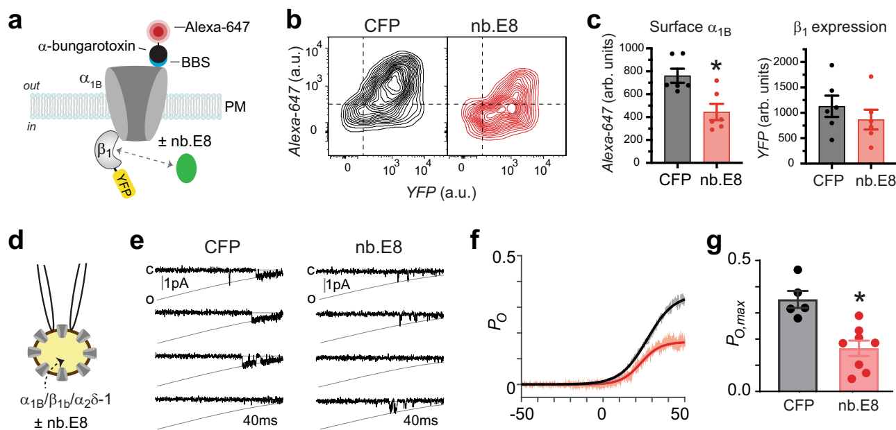
Fig. 5 | Nb.E8 inhibits Cav2.2 surface density and single channel P_o . a Schematic of BBS- \alpha_{1B} + \beta_{1b} -YFP \pm nb.E8. b Flow cytometry contour plots showing Cav2.2 surface density (Alexa647) vs \beta_{1b} expression (YFP) in HEK293 cells expressing \alpha_{1B} + \beta_{1b} + \alpha_2\delta -1 with either CFP (left) or nb.E8 (right). c Bar charts showing impact of nb.E8 on Cav2.2 surface density ( n = 6 over 3 independent experiments for both CFP and nb.E8 groups) and \beta_{1b} -YFP expression ( n = 6 over 3 independent experiments for both CFP and nb.E8 groups). ^*P = 0.0052 compared to CFP control, two-tailed unpaired t test. d Schematic of cell-attached single channel recording.
