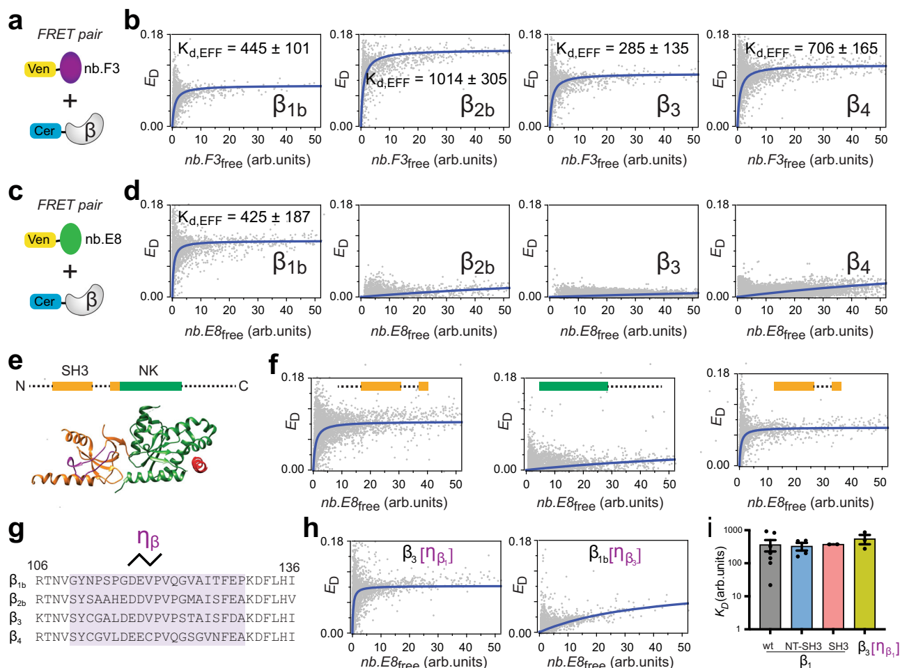
Fig. 2 | Identification of nb.E8 as a Cavβ 1 -selective nanobody. a Schematic of fluorescence resonance energy transfer (FRET) pair, Venus-nb.F3 + Cerulean-Cavβ. b Flow cytometry FRET (flow-FRET) scatter plots with FRET efficiency ( E_D ) plotted vs free nb.F3 concentration. The blue lines fit a 1:1 binding model to the data. Data show nb.F3 binds all four Cavβ subunit isoforms. K_{d,EFF} , effective dissociation constant. c Schematic of Venus-nb.E8 + Cerulean-Cavβ. d Flow-FRET scatter plots and binding curves show nb.E8 exclusively binds Cavβ 1 . e Top, schematic of Cavβ structural organization. Conserved src homology 3 (SH3, orange) and nucleotide kinase (NK, green) domains are bounded by variable N- and C-termini, and separated by a HOOK domain. Bottom, cryoEM structure of Cavβ 1a (PDB: 5GJV). f Flow-
