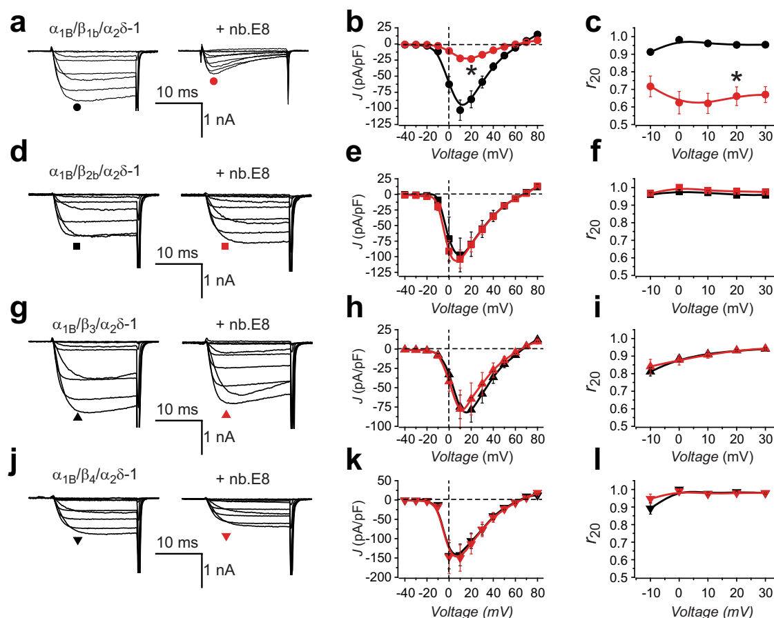
Fig. 4 | Nb.E8 inhibits current amplitude and speeds inactivation in Ca v β 1 -associated Ca v 2.2 channels. a Exemplar family of whole cell currents from HEK293 cells expressing reconstituted Ca v 2.2 channels (α 1 β+β 1 β+α 2 δ-1) in the absence (left) or presence (right) of nb.E8. b Population current density vs voltage (J-V) relationship for cells expressing α 1 β+β 1 β+α 2 δ-1 in the absence (black circles; n = 20 cells examined over 4 independent experiments) or presence (red circles; n = 16 cells examined over 4 independent experiments) of nb.E8. * P = 6.5 × 10 -5 , two-tailed unpaired t -test. c Fractional current remaining after 20 ms ( r 20 ) at various test pulse voltages for cells expressing α 1 β+β 1 β+α 2 δ-1 in the absence (black circles; n = 20 cells examined over 4 independent experiments) or presence (red circles; n = 13 cells examined over 4 independent experiments) of nb.E8. * P = 7.4 × 10 -5 , two-tailed unpaired t test. d-f Data for α 1 β+β 2 β+α 2 δ-1 ± nb.E8, same format as (a-c). e n = 8 cells examined over 3 independent experiments (black symbols) and n = 6 cells
