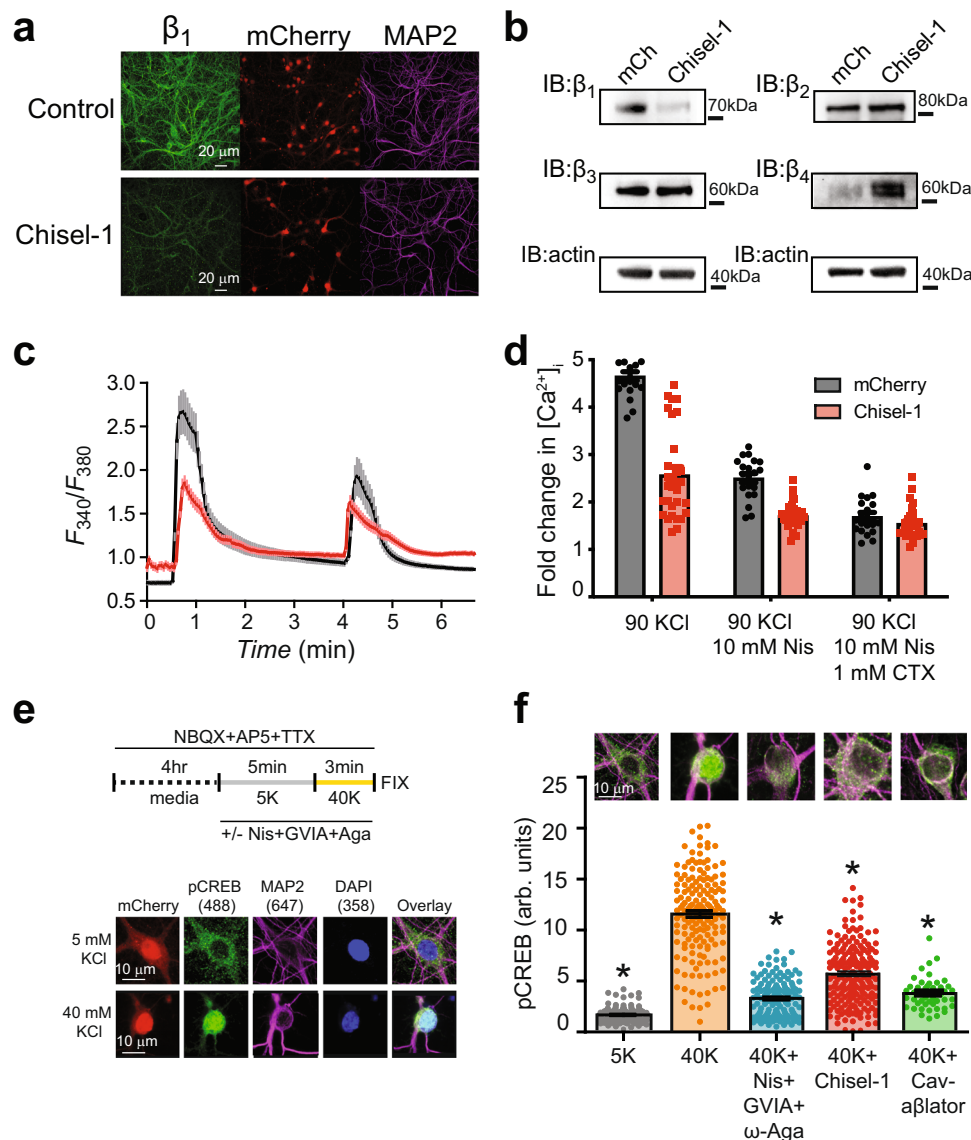
Fig. 9 | Chisel-1 inhibits Ca^{2+} influx and excitation-transcription coupling in hippocampal neurons. a Representative hippocampal neuron cultures expressing mCherry (top row) or Chisel-1-P2A-mCherry (bottom row) with immunofluorescence detection of \beta_{1b} (green) and MAP2 (purple). Images are representative of three independent experiments. b Representative Ca\beta isoform immunoblots from hippocampal neurons expressing either mCherry or Chisel-1. Immunoblots are representative of three independent experiments. c Time course of mean 90 KCl-evoked Ca^{2+} transients in hippocampal neurons expressing either mCherry (black line) or Chisel-1 (red trace). d Bar charts showing impact of Chisel-1 on 90 KCl-evoked Ca^{2+} transients before and after the addition of Ca_v1/Ca_v2 channel blockers (mCherry, n = 20 over 3 independent experiments; Chisel-1, n = 30 over 3 independent experiments). e Top, schematic of experimental protocol for assessing excitation-transcription coupling in cultured hippocampal neurons. Bottom,
