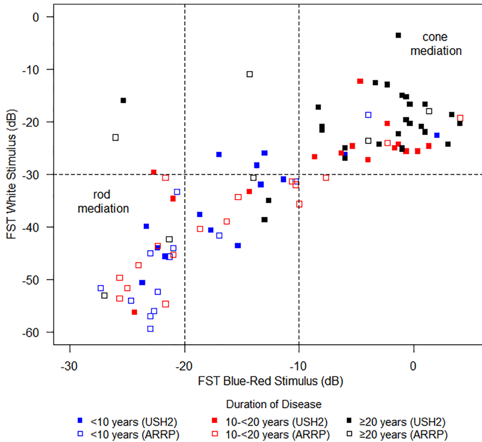
Figure 3. Full-field stimulus thresholds (FST) white versus blue-red by duration of disease and clinical diagnosis. Filled symbols represent USH2 participants and open symbols represent ARR participants. Blue, red, and black symbols represent duration of disease at < 10 years, 10 to < 20 years, and ≥20 years, respectively.
