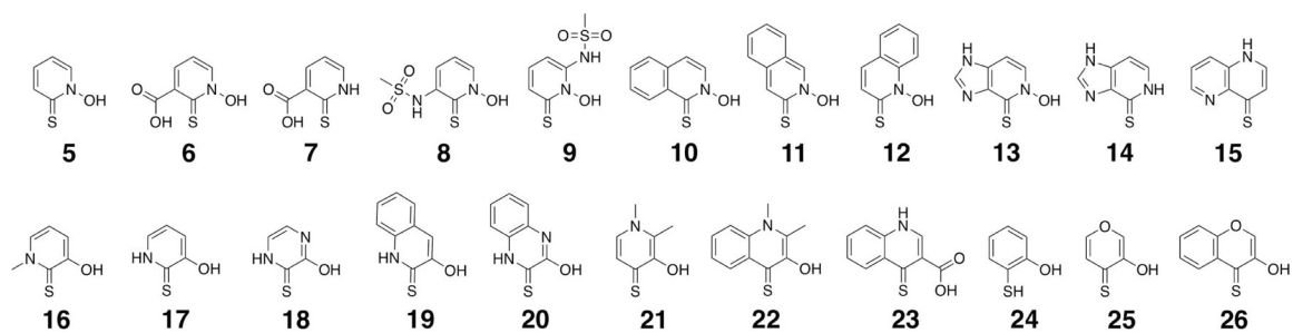
Figure 4. HOPTO derivatives tested for IDE inhibition.
