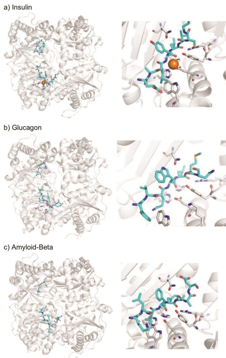
Figure 2. Binding of IDE to a broad range of substrates, as exemplified by: a) insulin, b) glucagon, and c) A \beta . [2] The full structure of IDE bound to each substrate is shown on the left, with close-ups of the catalytic site shown on the right. The zinc ion is depicted as an orange sphere in (a). Images produced from PDB IDs 2G54, 2G49, and 2G47, respectively.
