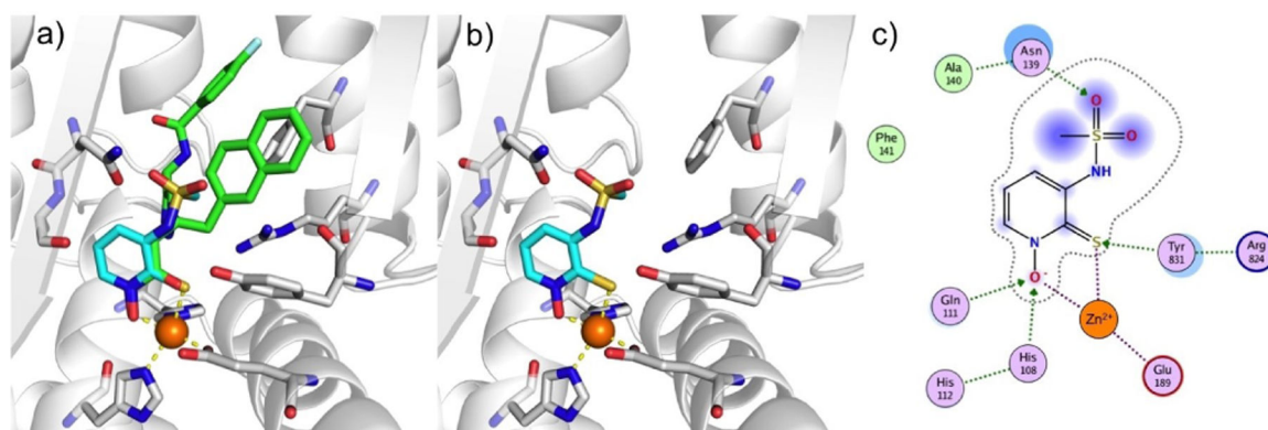
Figure 5. Model of 8 bound to the Zn 2+ within the active site of IDE. a) Superposition of 8 and 2 , which was used to create b) a model of 8 bound to the Zn 2+ in the IDE active site. c) A 2-D representation of the model of 8 binding, with Zn 2+ in orange, coordination bonds as pink dashes, interactions as green arrows, and solvent exposed regions as blue spheres.
