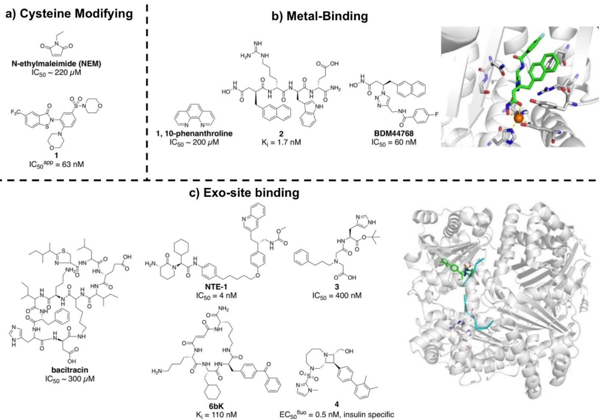
Figure 3. Structures and inhibitory values of reported IDE inhibitors. [3,18,21,22,24–28] a) Cysteine-modifying IDE inhibitors. b) Metal-binding IDE inhibitors; inset: crystal structure of hydroxamate-based compound 2 coordinating to the active site Zn^{2+} , PDB ID: 4NXO. [22] c) Exosite-binding IDE inhibitors; inset: crystal structure of 4 (green) bound to the exosite and co-crystallized with insulin (cyan) PDB ID: 6EDS. [18]
