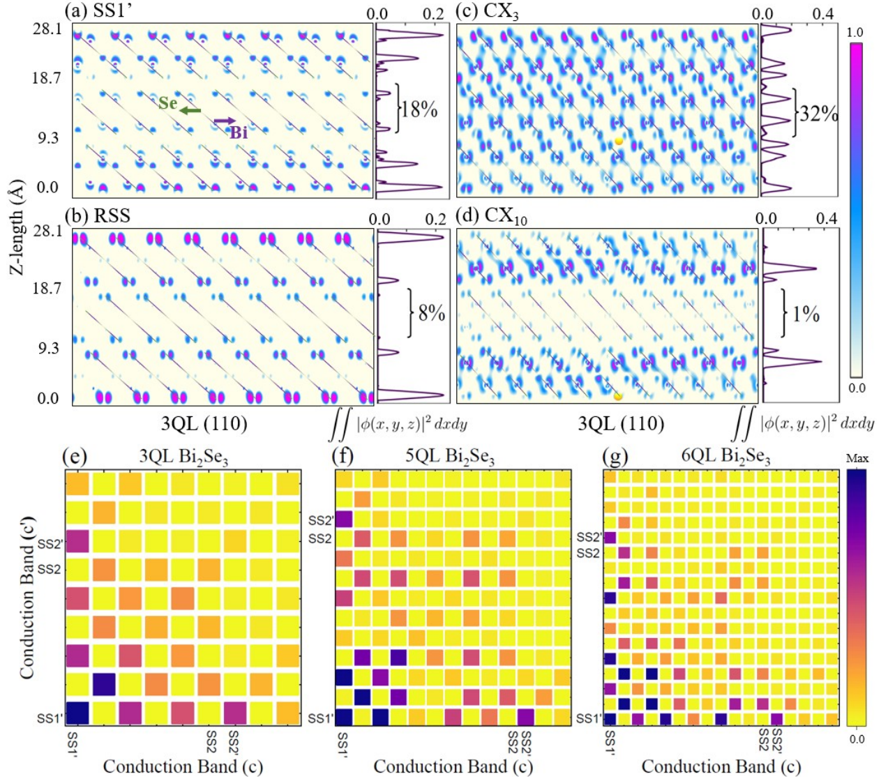
FIG.4 (a-b) The modulus of the electronic wavefunction in 3QL Bi 2 Se 3 for the surface states SS1' and RSS at the \Gamma point. (c-d) The modulus of the exciton wavefunction for CX 3 and CX 10 , when the hole (yellow sphere) is fixed. The hole position is set at the location that maximizes the wavefunction amplitude. The integral of the modulus squared of each wavefunction over the x-y plane is shown as a side panel in (a-d). The percentage label indicates the contribution to the wavefunction from the central QL. For clarity, the Bi and Se atoms are not explicitly shown. The bonds are depicted as purple lines in the vicinity of Bi and green lines in the vicinity of Se. (e-g) Electron-hole exchange matrix elements \langle vc k | K^x | v' c' k' \rangle for k=k'=\Gamma and v=v'=SS1 for (e) 3QL, (f) 5QL and (g) 6QL slabs of Bi 2 Se 3 .
