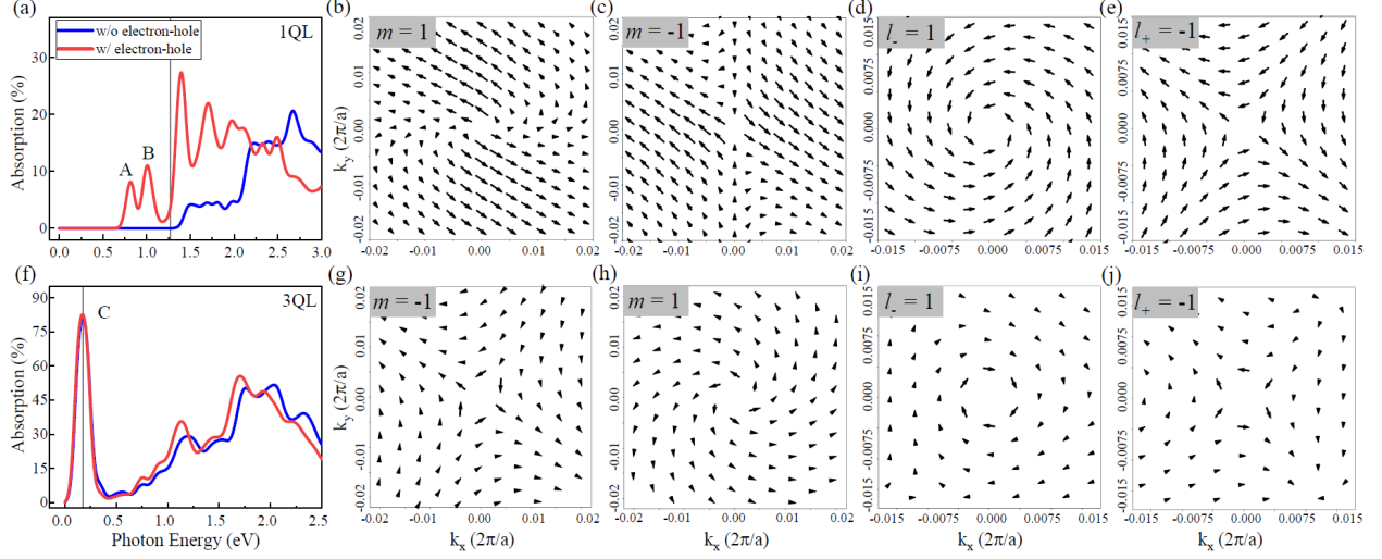
FIG.2 Calculated absorption spectra of (a) 1QL and (f) 3QL Bi 2 Se 3 with(without) electron-hole interactions included at the GW-BSE(GW-RPA) level in red(blue). The gray vertical line indicates the G_0W_0 quasiparticle bandgap. (b-c) The phase winding of the exciton envelope wavefunction, A_{vc}^S , of the degenerate bright excitons contributing to peak A of 1QL Bi 2 Se 3 and (g-h) degenerate bright excitons contributing to peak C of 3QL Bi 2 Se 3 . The angle of the arrows indicates the phase, and the length of each arrow indicates the amplitude. The index m denotes the winding number around the \Gamma point. (d-e) The winding of the optical interband dipole transition matrix element between the highest valence band and the lowest conduction band for 1QL and (i-j) 3QL Bi 2 Se 3 . The index l_{-(+)} denotes the winding number of left(right) circularly polarized light respectively. A maximally smooth local gauge is imposed following Refs. [59,60]. The exciton wavefunction and optical interband transitions are plotted in a patch centered around the \Gamma point in the BZ, marked by grey area in Fig. 1(c).
