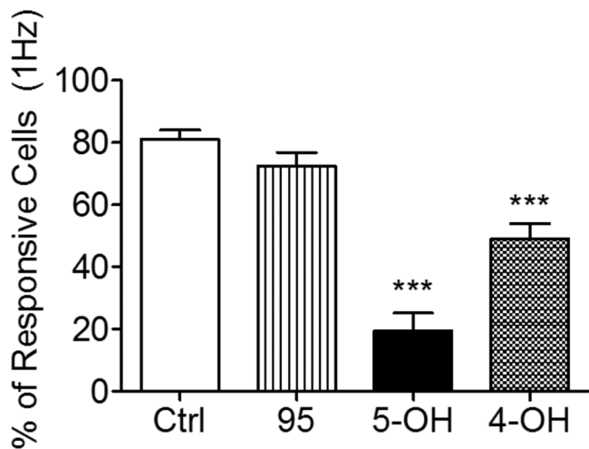
FIG. 7. Subacute exposure to 4-OH- and 5-OH-PCB95 impairs ECC in myotubes. The percent of cells retaining electrically evoked ECC was scored after 3-h exposure to 300 nM vehicle or PCB. Response is defined as the total number of cells responding to a minimum of 1 Hz electrical stimulation within 3–5 fields/well of control and PCB-treated wells within at least 2 different cultures. Fields within each well were chosen randomly, and the ratio of cells responding to total cells was determined. Error bars represent SEM. *** p < .001 ; one-way ANOVA with Dunnett multiple comparison post hoc test. Abbreviations: ECC, excitation-contraction coupling; PCB, polychlorinated biphenyl.
