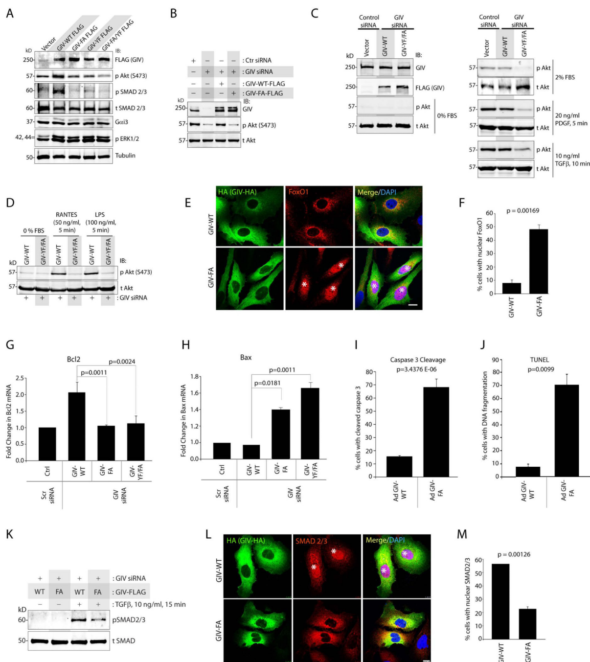
Figure 6. GIV's GEF function enhances profibrogenic Akt and SMAD signals in HSCs
