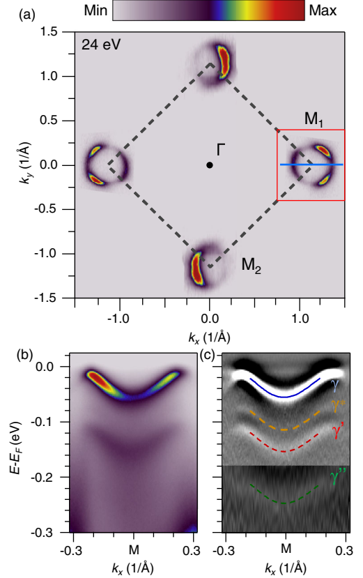
FIG. 1. Fermi surface and replica band topology in single-layer FeSe/SrTiO 3 . (a) Fermi surface map of single-layer FeSe/SrTiO 3 taken with p -polarized light at h\nu = 24 eV. (b) High-statistics spectra along the cut shown at M 1 (blue). (c) Second-derivative of the spectra in (b). An additional 60 meV replica (labeled \gamma^* in the figure) is clearly visible, as well as a second-order replica (labeled \gamma'' ) after saturating the color scale over the higher binding energy region.
