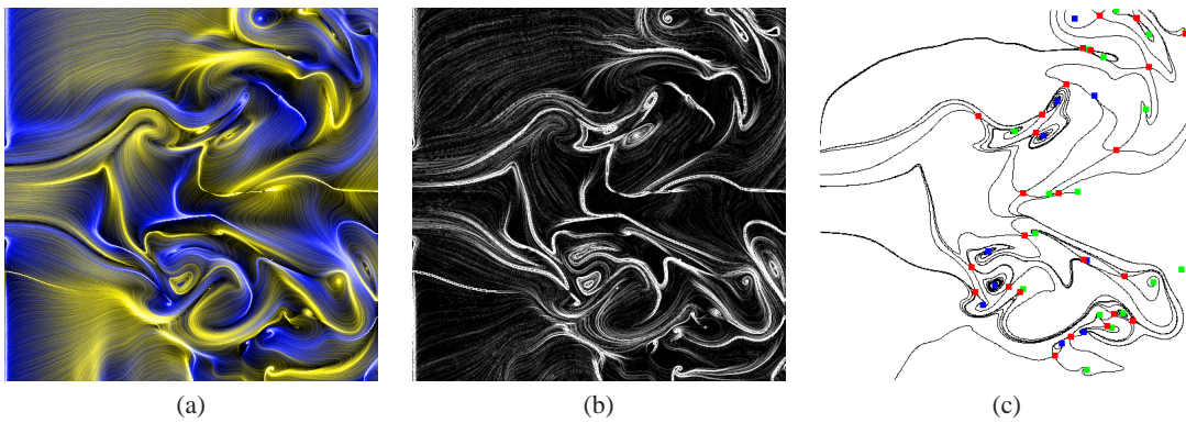
Figure 6: Two-dimensional simulation of a swirling jet, our method for two different transfer functions, (a) Overall flow behavior and (b) transfer function applied to the gradient magnitude of the density function in to focus on the structure, in comparison with (c) the explicit topology. (The explicit topology image generated with the software FAnToM developed at the university of Kaiserslautern.)
