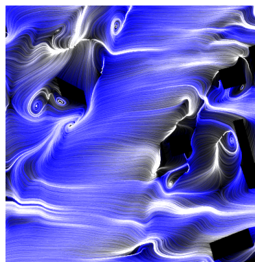
Figure 4: Structure visualization of a 2D slice of the New Orleans airflow dataset. Critical points like saddle, sources and sinks and their connections with context are emphasized by the visualization.
