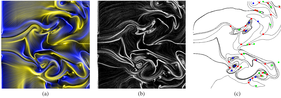
Figure 6: Two-dimensional simulation of a swirling jet, our method for two different transfer functions in comparison with the explicit topology. (The explicit topology image is generated with the software FAnToM developed at the university of Kaiserslautern.)
